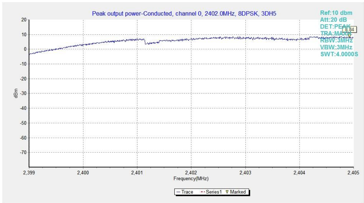
Fig.7. Peak Output Power -Conducted: 8DPSK, Channel 0,
