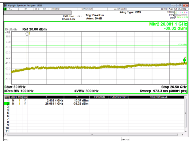
OUT-OF-BAND 0 CHANNEL
