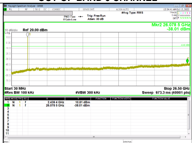
OUT-OF-BAND 19 CHANNEL
