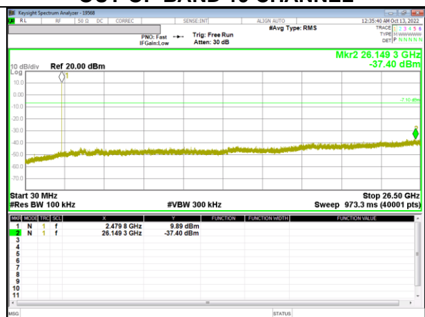
OUT-OF-BAND 39 CHANNEL
