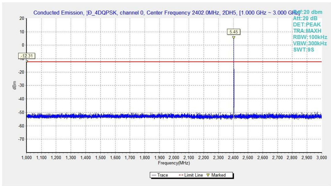
Fig.45. Conducted spurious emission: \pi/4 DQPSK, Channel 0, 1GHz - 3GHz
