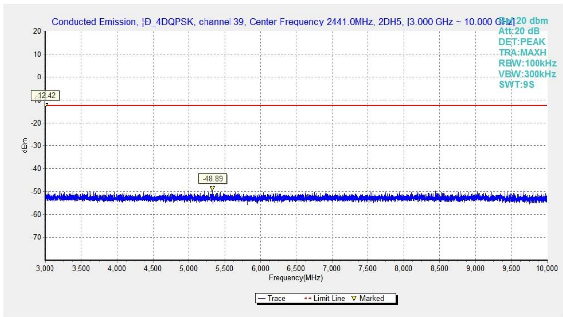
Fig.51. Conducted spurious emission: \pi/4 DQPSK, Channel 39, 3GHz - 10GHz
