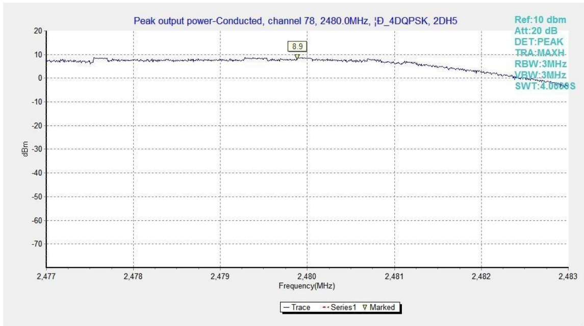
Fig.6. Peak Output Power -Conducted: \pi/4 DQPSK, Channel 78,
