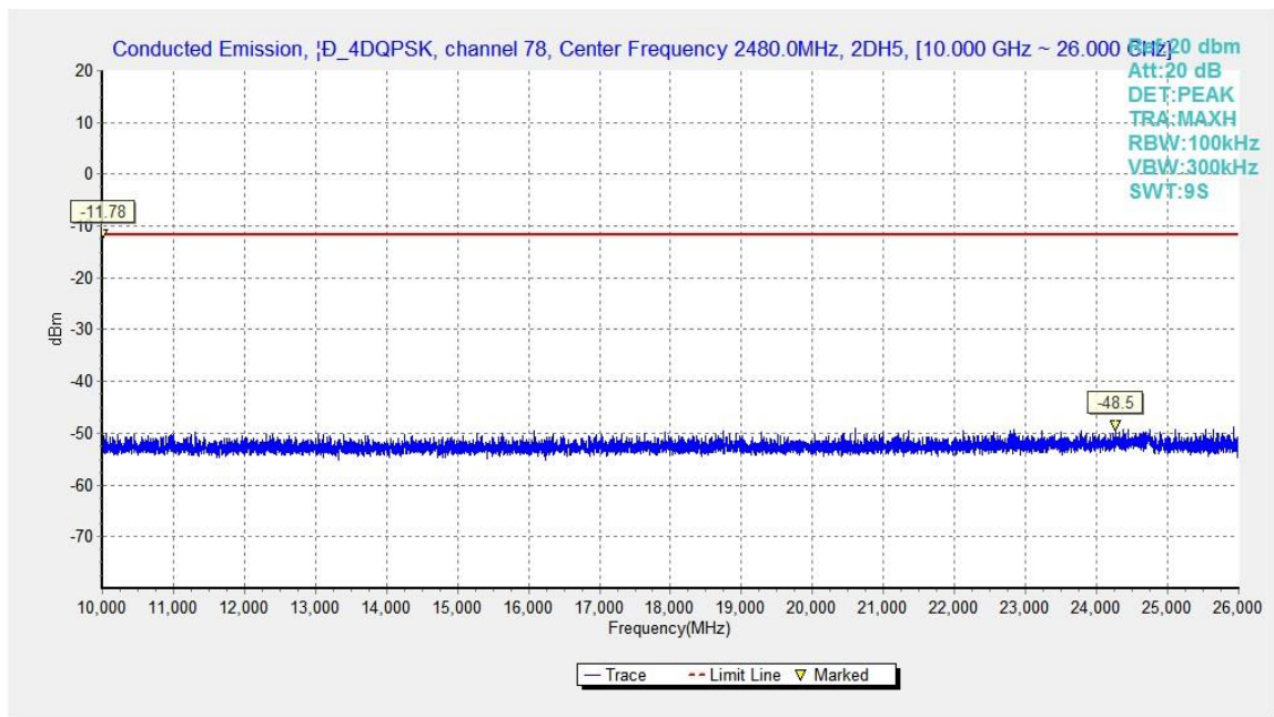
Fig.57. Conducted spurious emission: \pi/4 DQPSK, Channel 78, 10GHz - 26GHz
