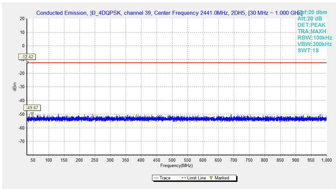
Fig.49. Conducted spurious emission: \pi/4 DQPSK, Channel 39, 30MHz - 1GHz
