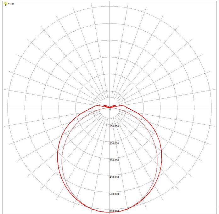
EV/UMBRA/PRO/IP65/600/3000K
