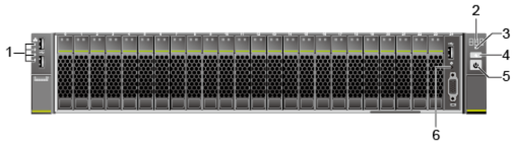
Figure 4-12 Front panel of a server with twenty-four 2.5-inch drives
