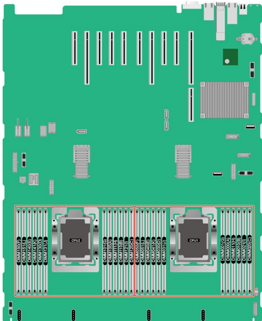
Figure 6-1 DIMM slots
