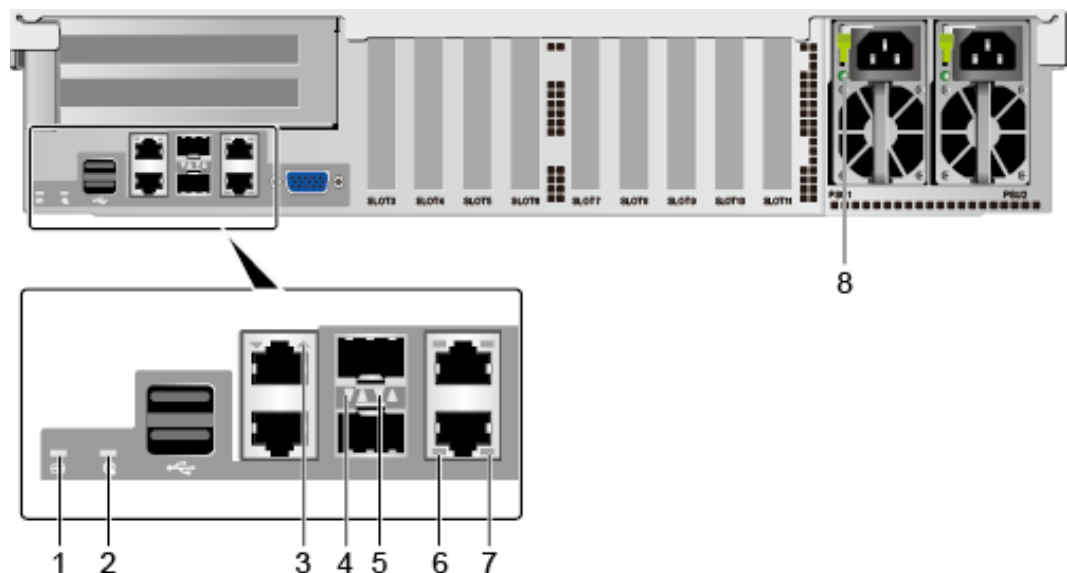
Figure 4-14 Indicators on the rear panel
