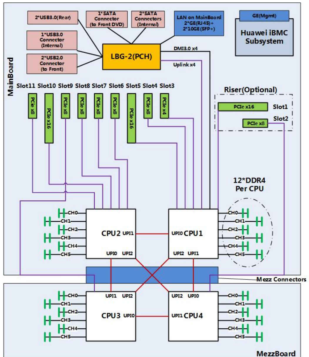
Figure 3-1 Logical structure of the 2488H V5
