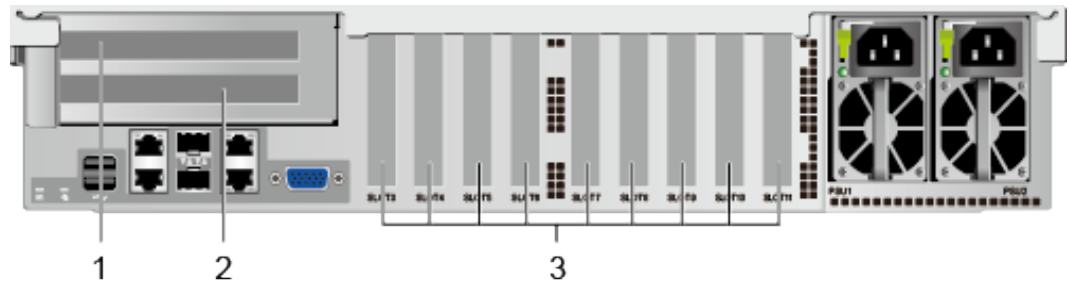
Figure 4-17 PCIe slots
