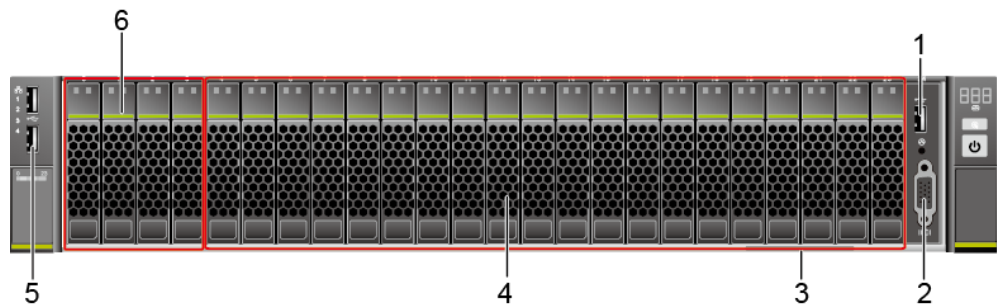
Figure 4-9 Front panel of a server with 24 NVMe SSDs
