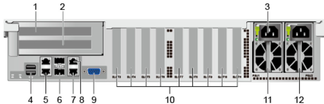
Figure 4-10 Rear panel
