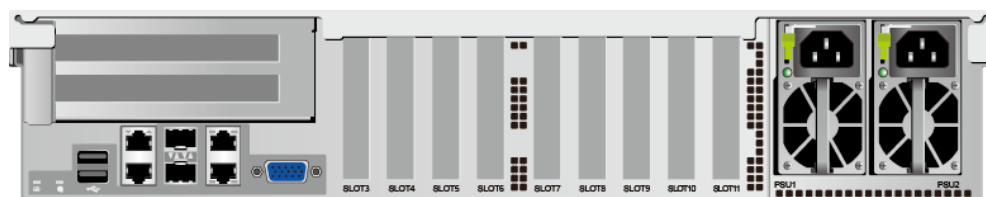
Figure 4-4 Rear panel
