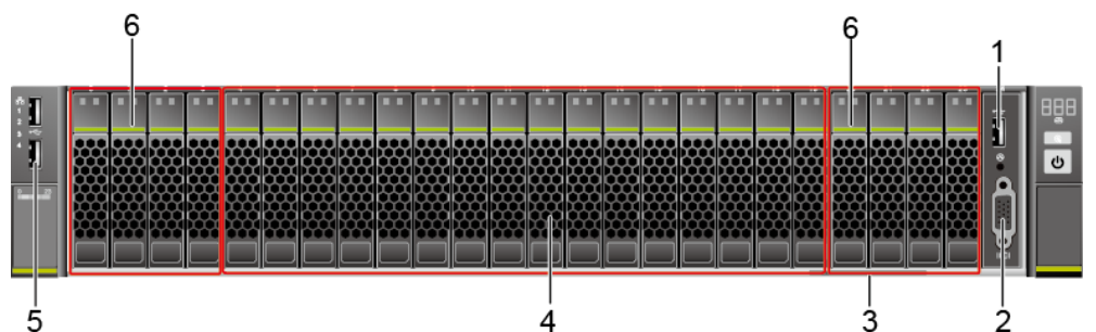
Figure 4-8 Front panel of a server with 16 SAS/SATA drives and 8 NVMe SSDs
