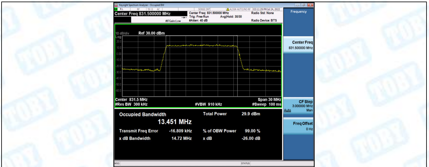
Band26-15MHz-QPSK-26915-75RB#0
