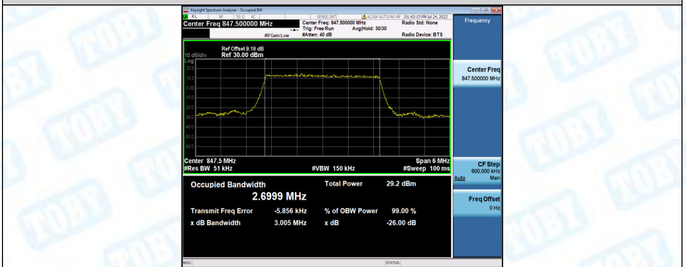
Band26-3MHz-16QAM-26805-15RB#0
