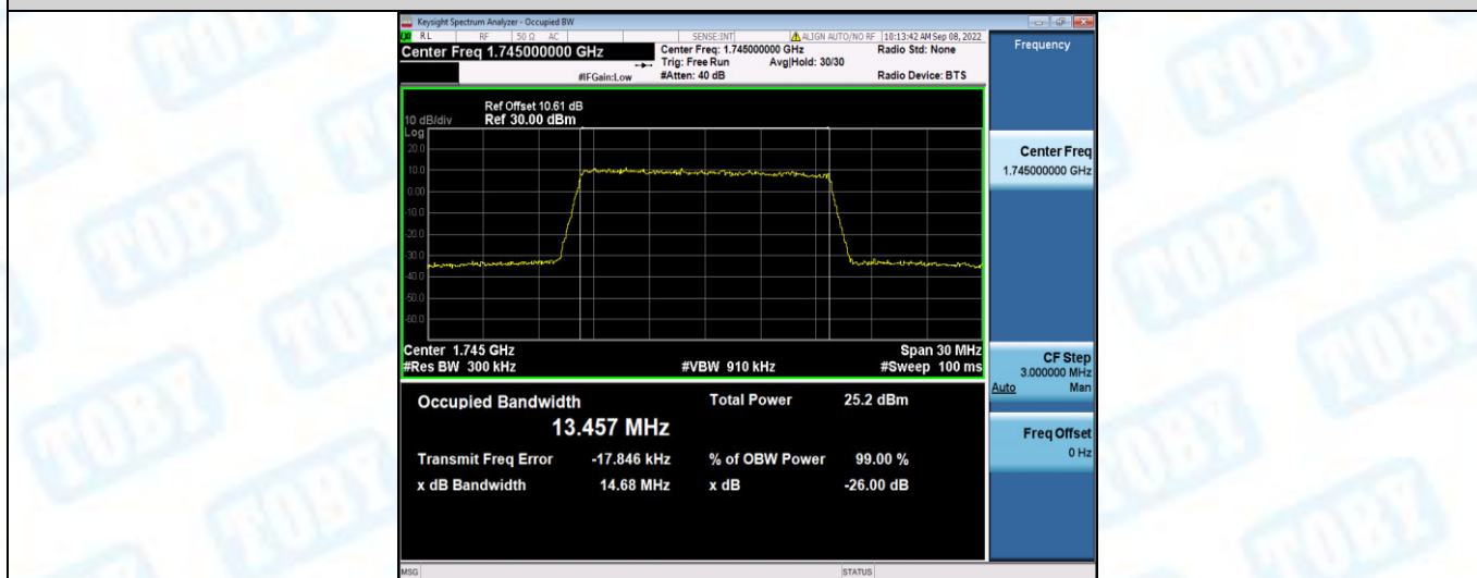
Band66-15MHz-16QAM-132597-75RB#0
