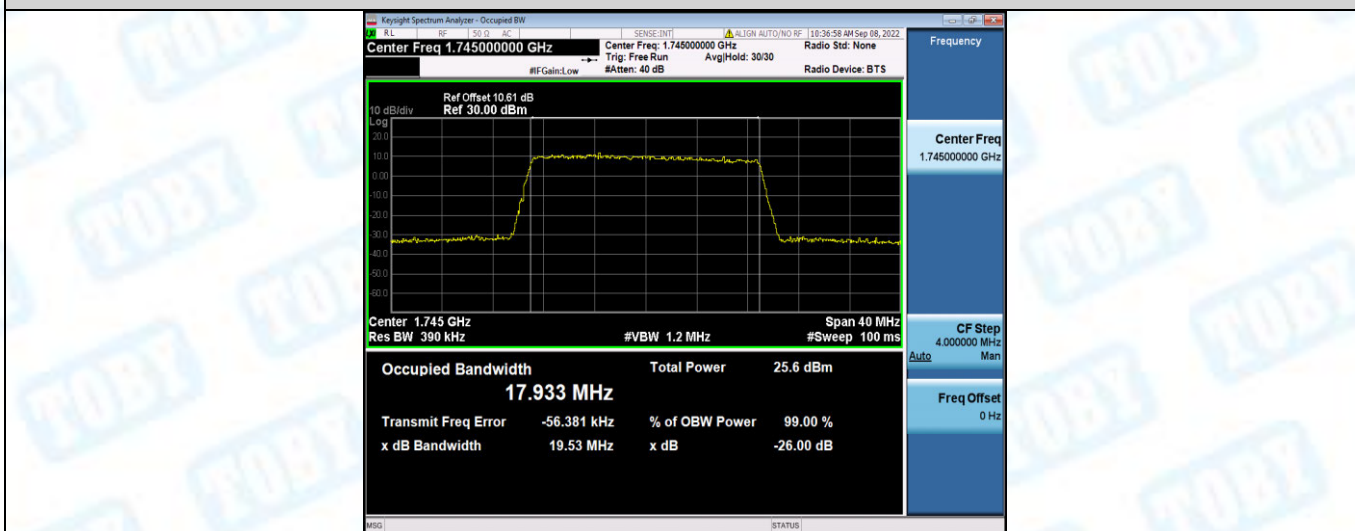
Band66-20MHz-16QAM-132572-100RB#0
