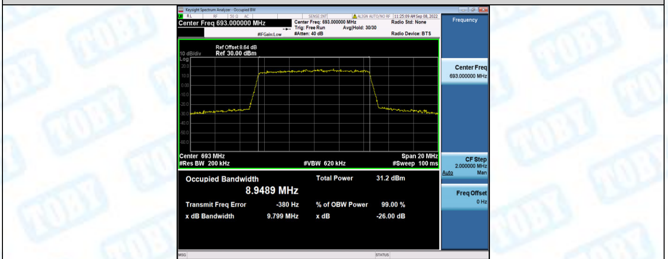
Band71-15MHz-QPSK-133197-75RB#0
