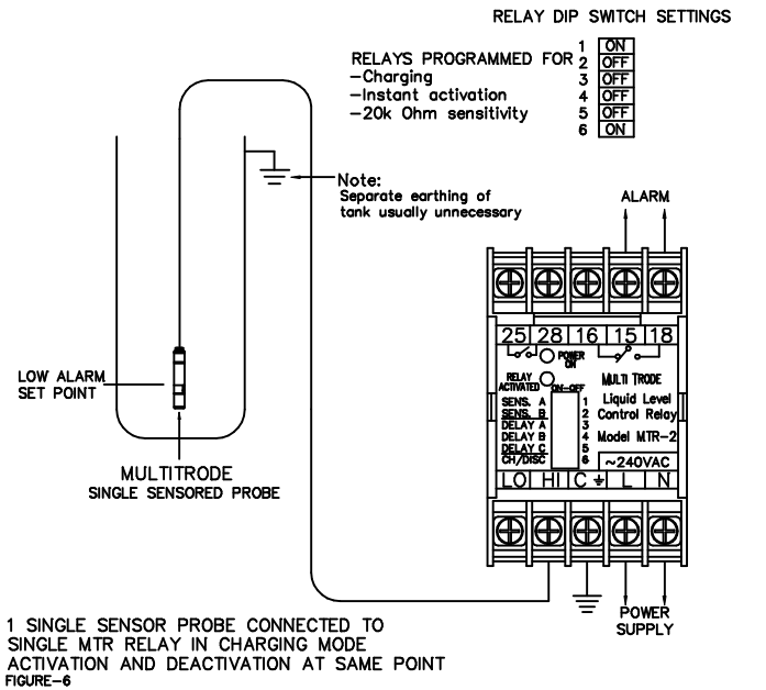
1 SINGLE SENSOR PROBE CONNECTED TO SINGLE MTR RELAY IN CHARGING MODE ACTIVATION AND DEACTIVATION AT SAME POINT
