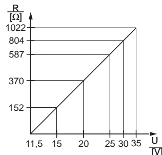
Temperature head transmitter load chart for estimating the load resistance. Additional resistances have to be subtracted from the value calculated as shown in the equation.
