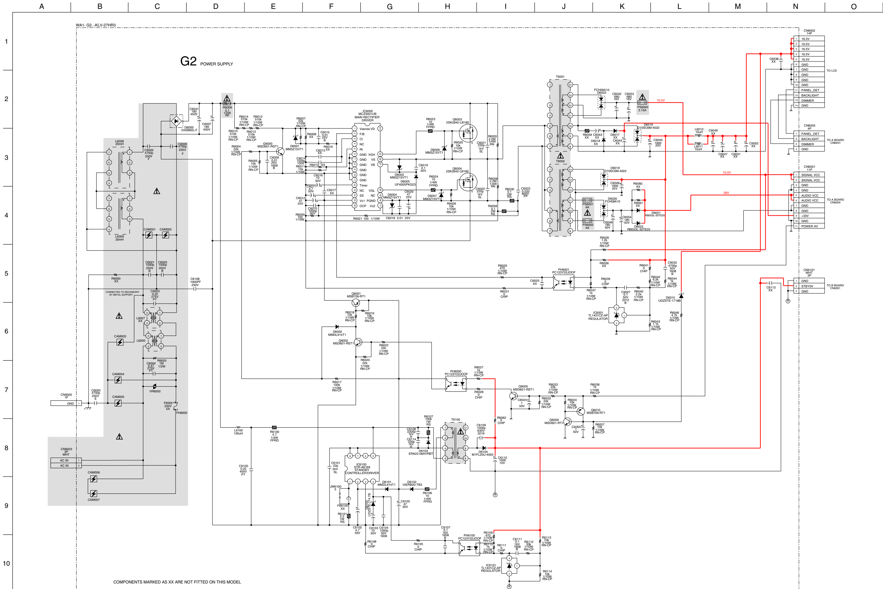
~ G2 Board Schematic Diagram [ Power Supply ] ~
