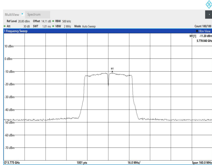
11AC80SISO_Ant2_5775
