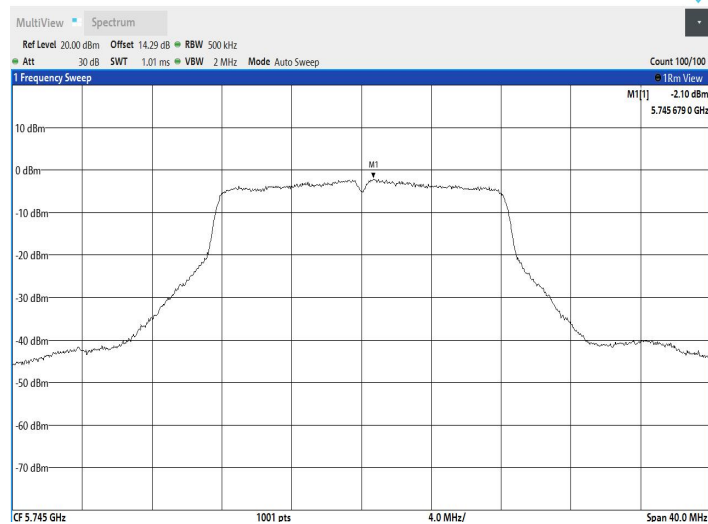
11A_Ant1_5785
