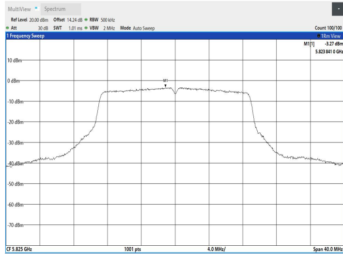
11N40SISO_Ant1_5755
