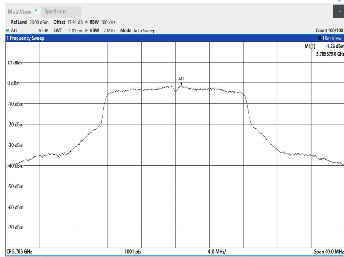
11A-CDD_Ant2_5785
