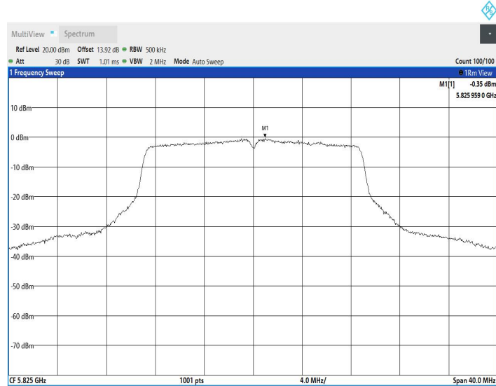
11AC20SISO_Ant2_5825
