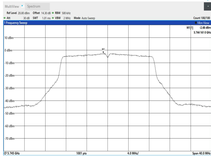
11N20SISO_Ant1_5785
