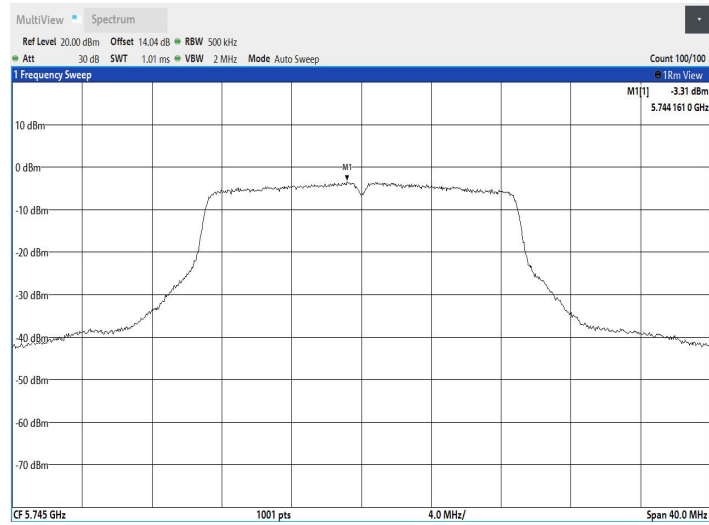
11AC20SISO_Ant2_5745
