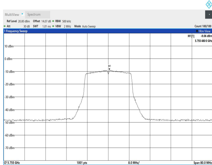
11AC40SISO_Ant2_5755
