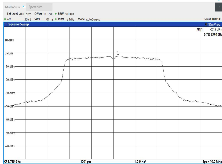
11AC20SISO_Ant2_5785
