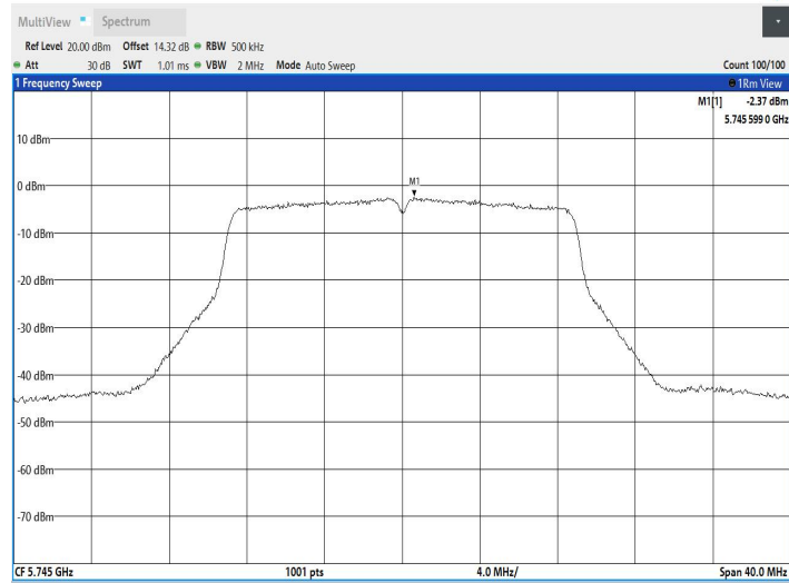
11AC20SISO_Ant1_5785
