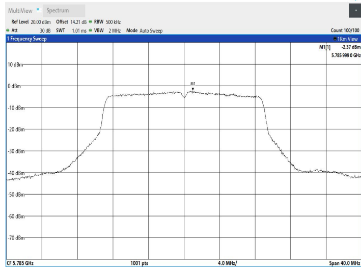
11N20SISO_Ant1_5825
