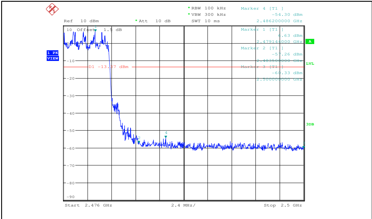
Band-edge for RF Conducted Emissions_3DH5_2480_Hopping Off
