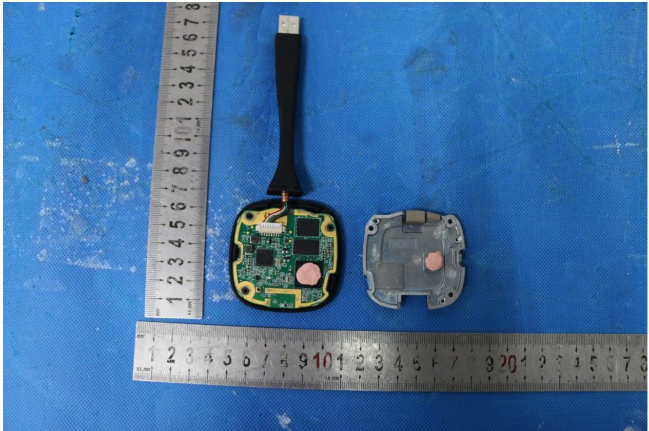
Internal View of AirPresence Key
