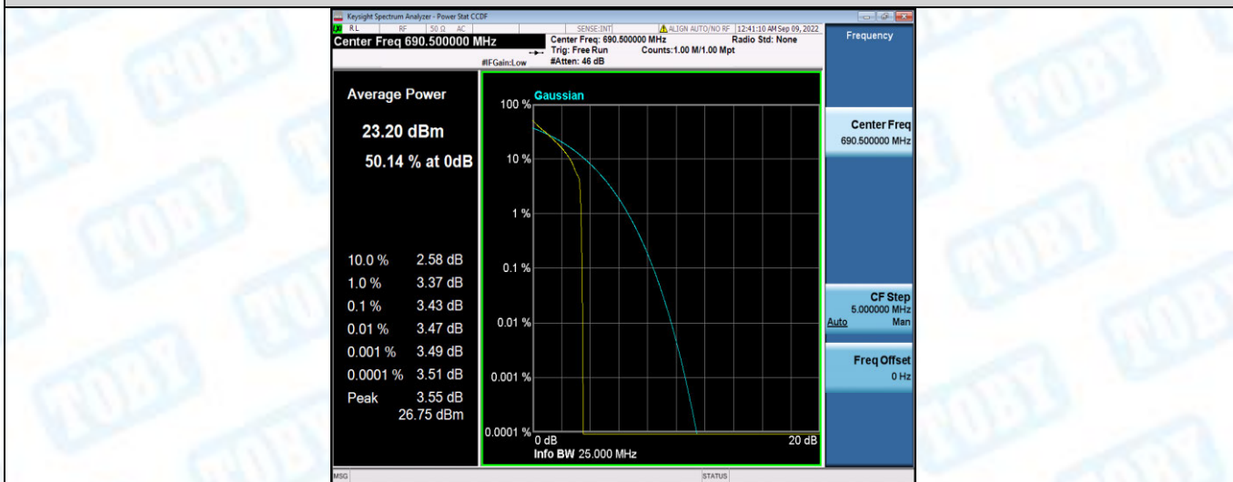
Band71-15MHz-QPSK-133397-75RB#0
