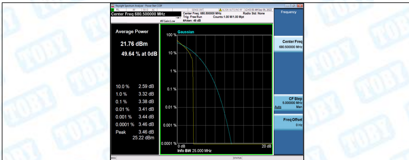
Band71-20MHz-QPSK-133297-100RB#0
