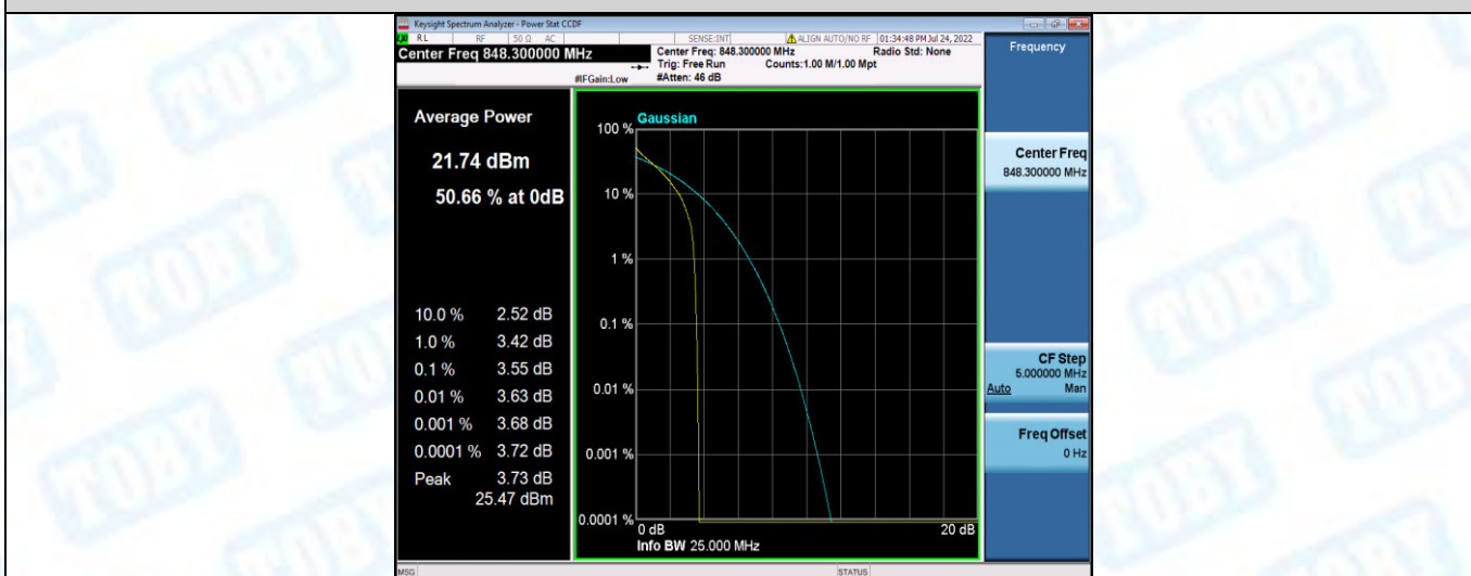
Band26-1.4MHz-QPSK-27033-6RB#0
