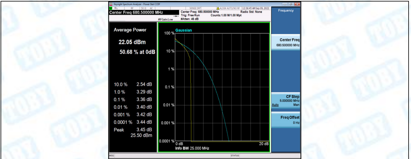
Band71-10MHz-QPSK-133297-50RB#0
