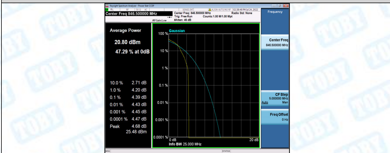
Band26-5MHz-16QAM-27015-25RB#0
