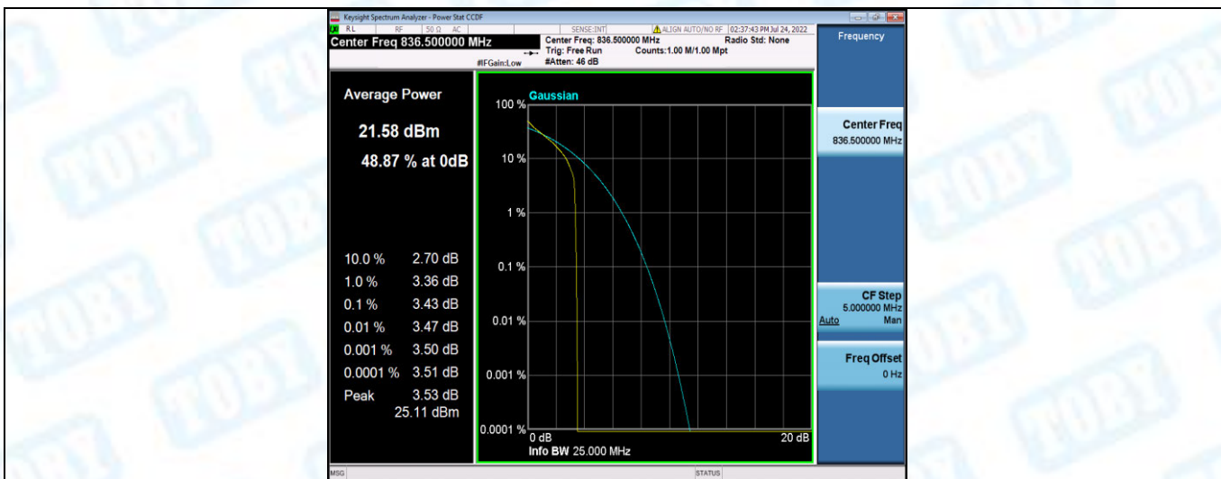
Band26-5MHz-QPSK-26915-25RB#0
