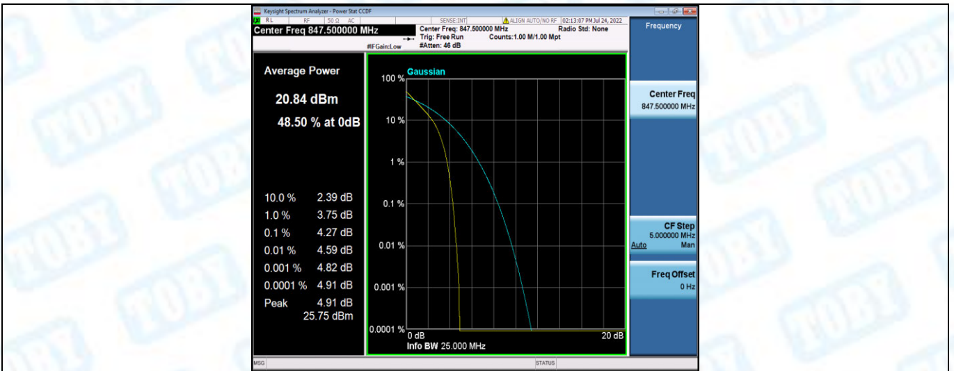
Band26-3MHz-16QAM-26805-1RB#0
