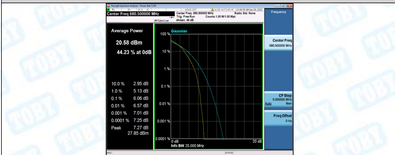
Band71-15MHz-16QAM-133397-1RB#0
