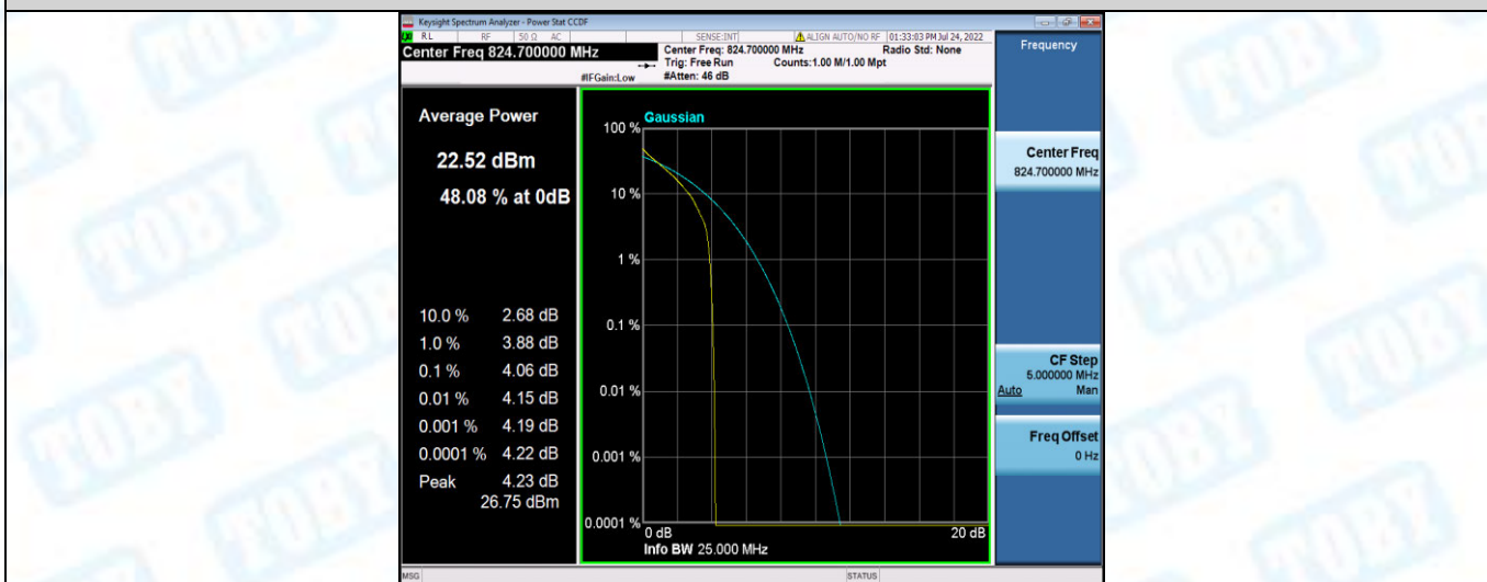
Band26-1.4MHz-QPSK-26797-6RB#0
