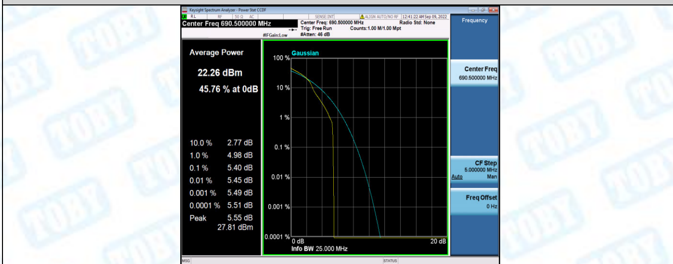
Band71-15MHz-16QAM-133397-75RB#0
