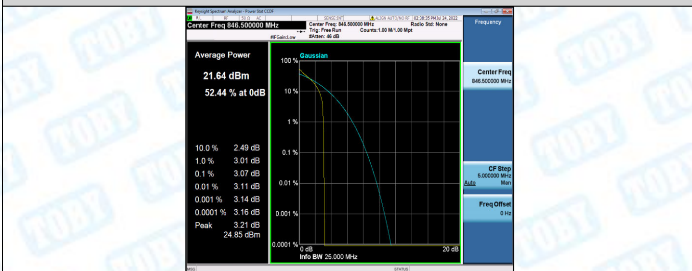
Band26-5MHz-QPSK-27015-25RB#0
