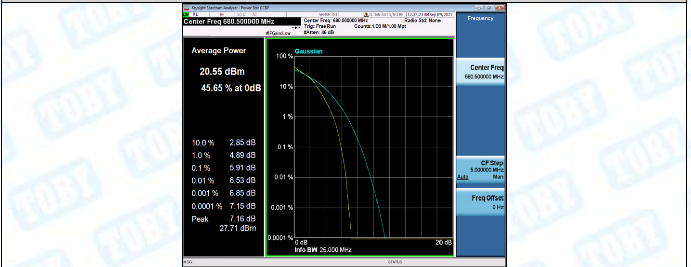
Band71-10MHz-16QAM-133422-1RB#0
