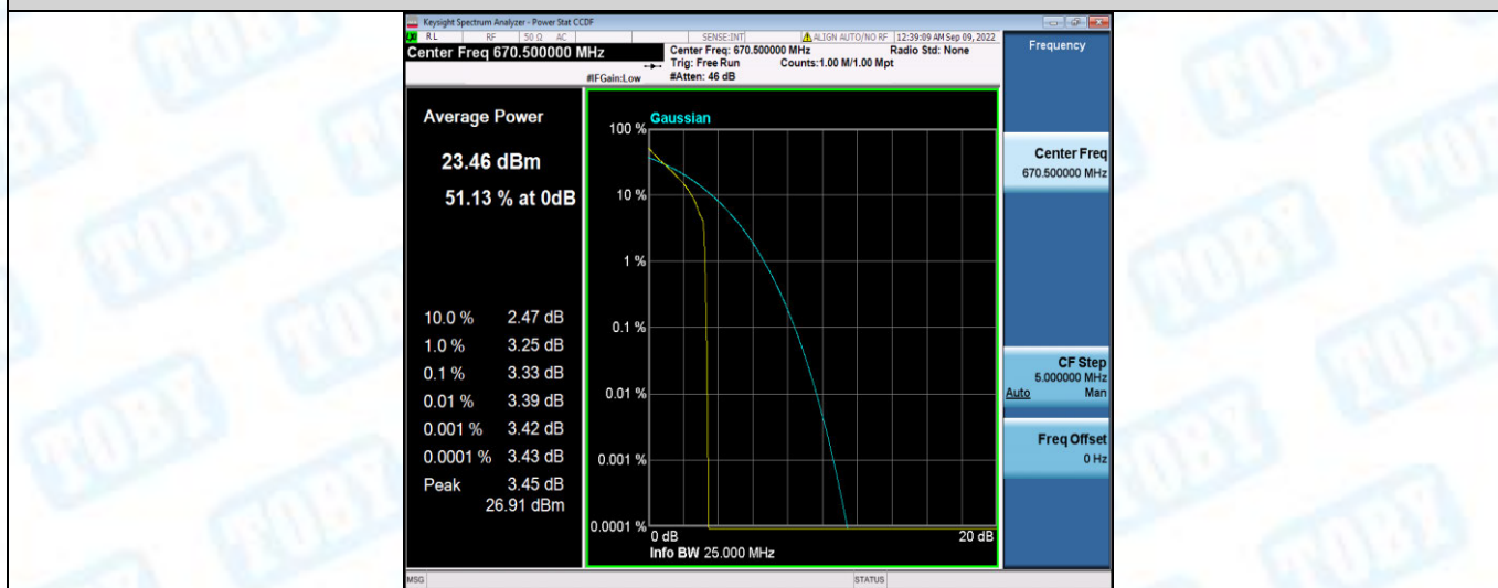
Band71-15MHz-QPSK-133197-75RB#0
