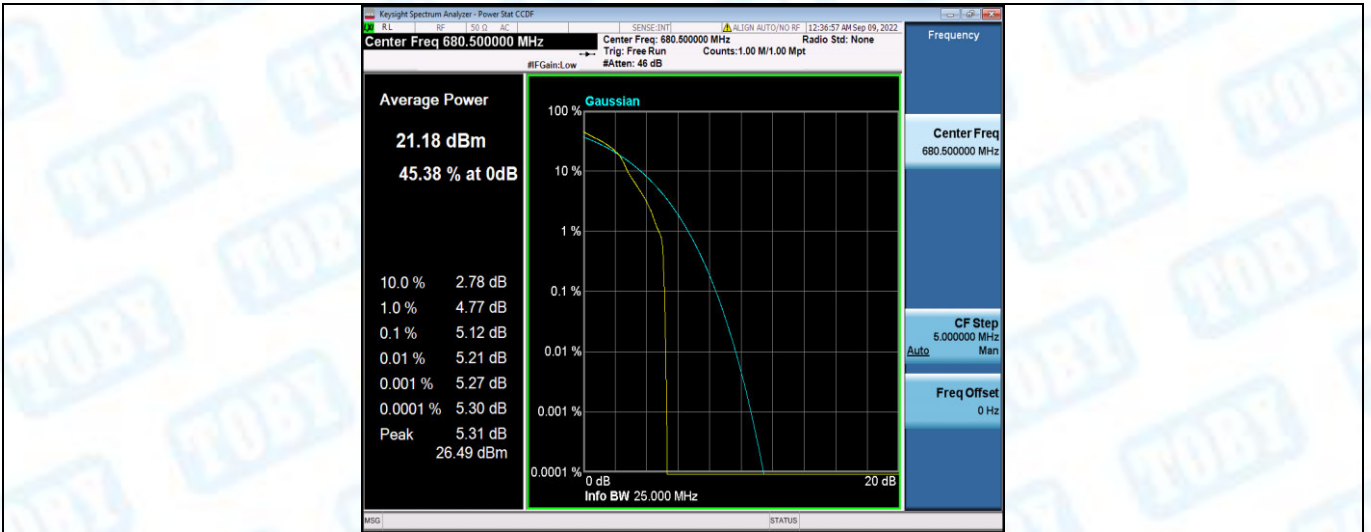
Band71-10MHz-16QAM-133297-50RB#0
