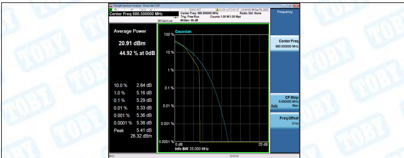
Band71-20MHz-16QAM-133297-100RB#0
