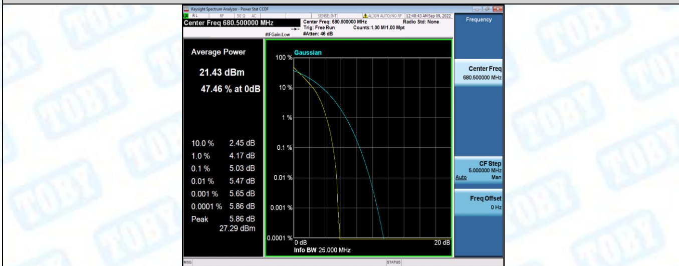
Band71-15MHz-QPSK-133397-1RB#0
