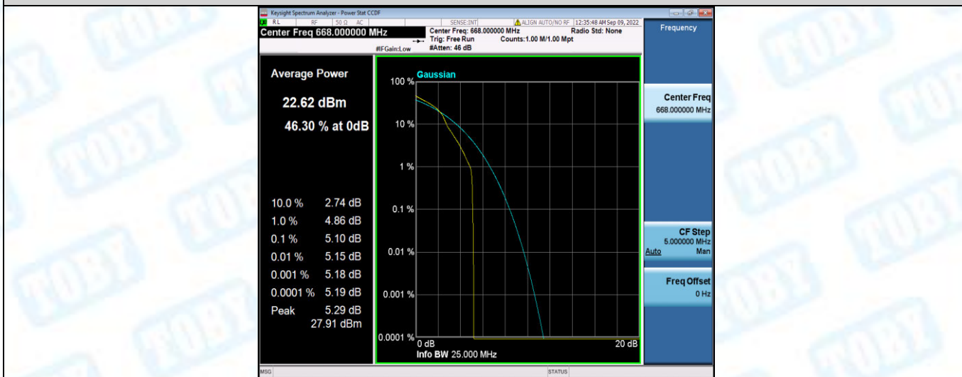
Band71-10MHz-16QAM-133172-50RB#0
