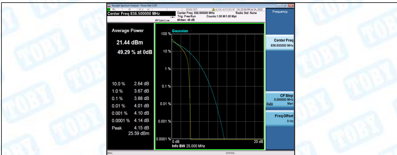
Band26-1.4MHz-QPSK-26915-6RB#0
