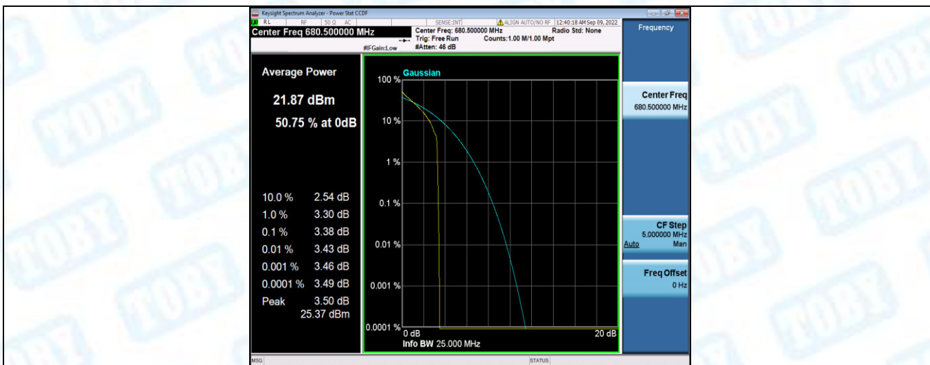
Band71-15MHz-QPSK-133297-75RB#0
