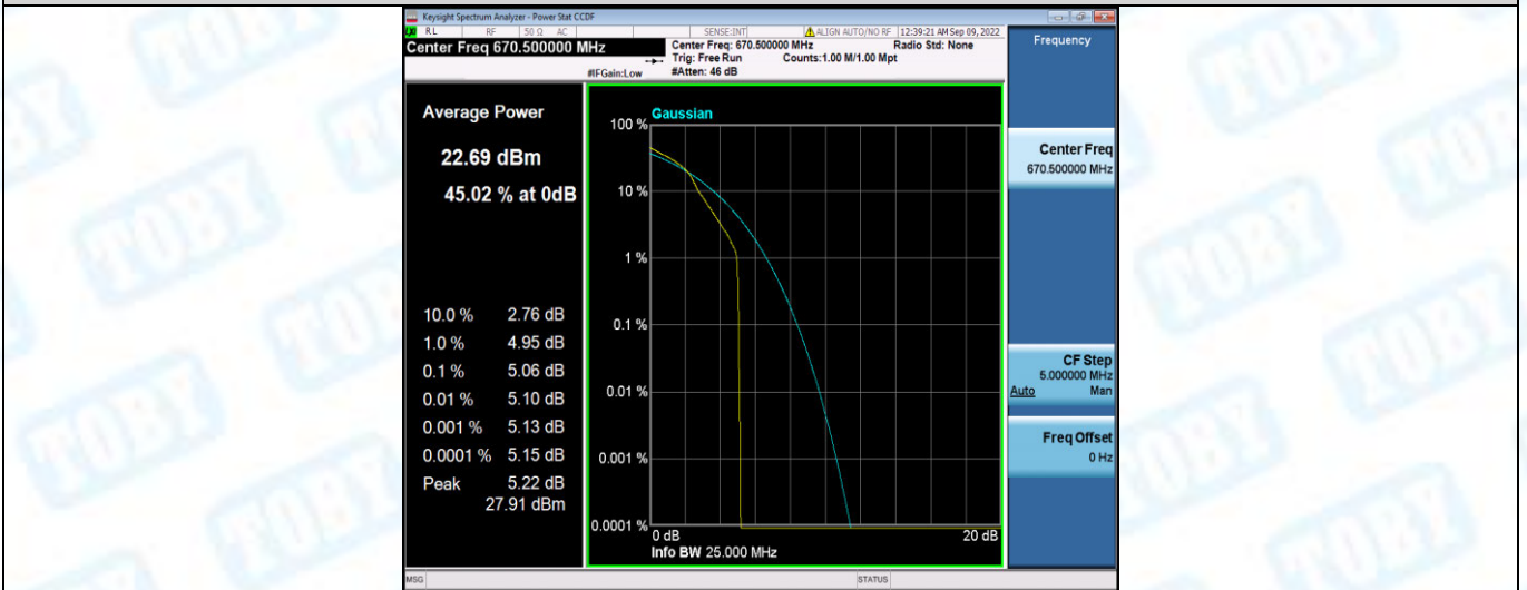
Band71-15MHz-16QAM-133197-75RB#0
