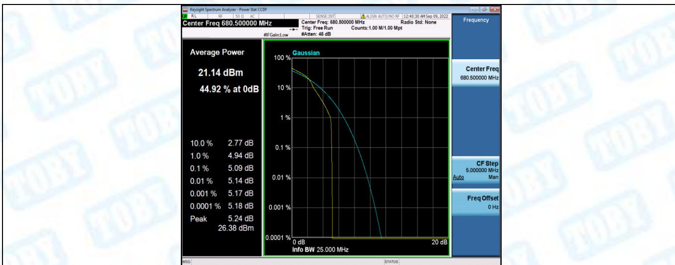
Band71-15MHz-16QAM-133297-75RB#0
