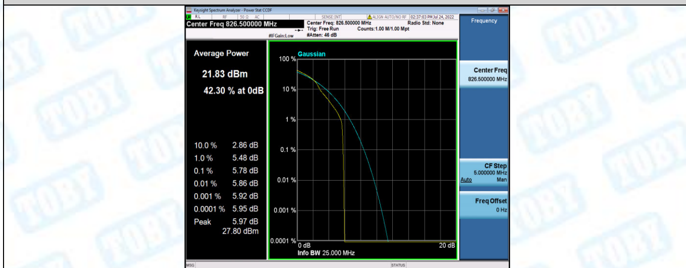
Band26-5MHz-16QAM-26815-25RB#0
