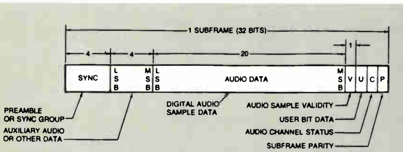
Figure 2: AES/EBU Serial Interface Format
