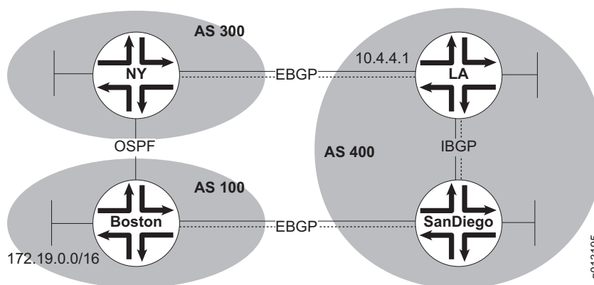
Figure 40: Backdoor Route
