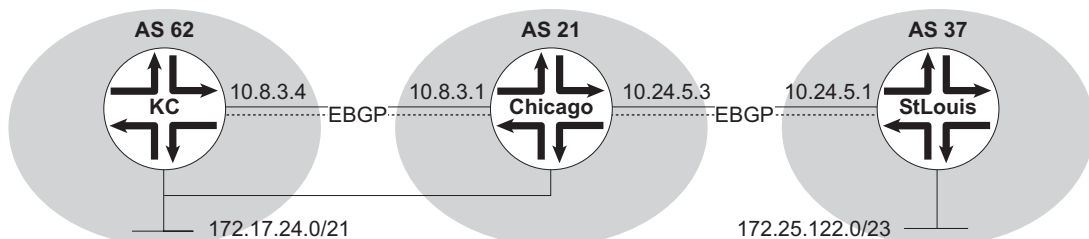
Figure 38: Administrative Distances
