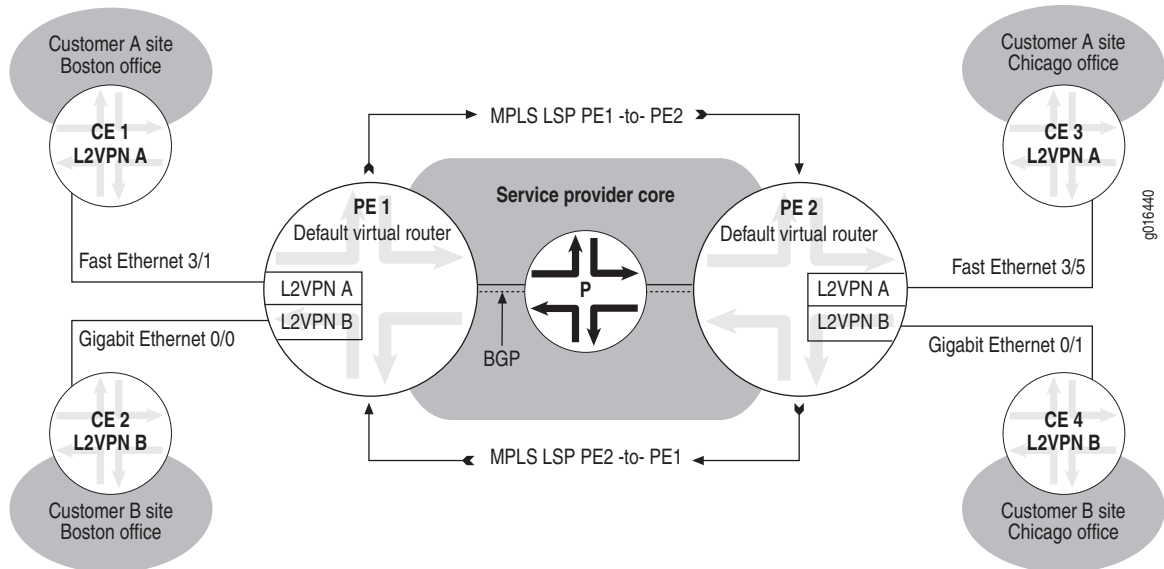
Figure 124: L2VPN Components
