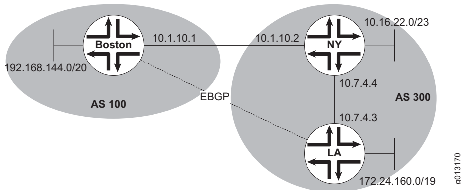
Figure 12: Using EBGP-Multihop
