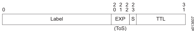
Figure 50: Shim Header
