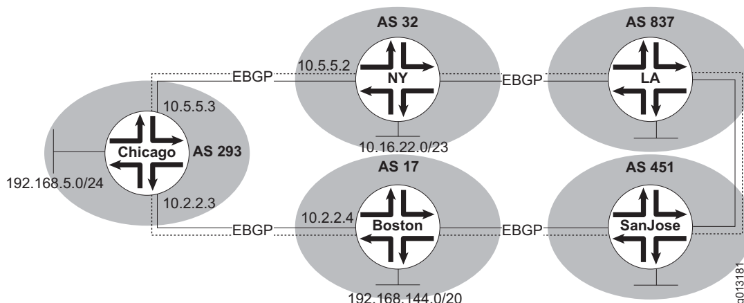
Figure 25: Route Map Filtering
