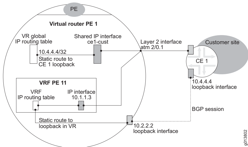
Figure 103: BGP Session Between CE Router and Parent VR
