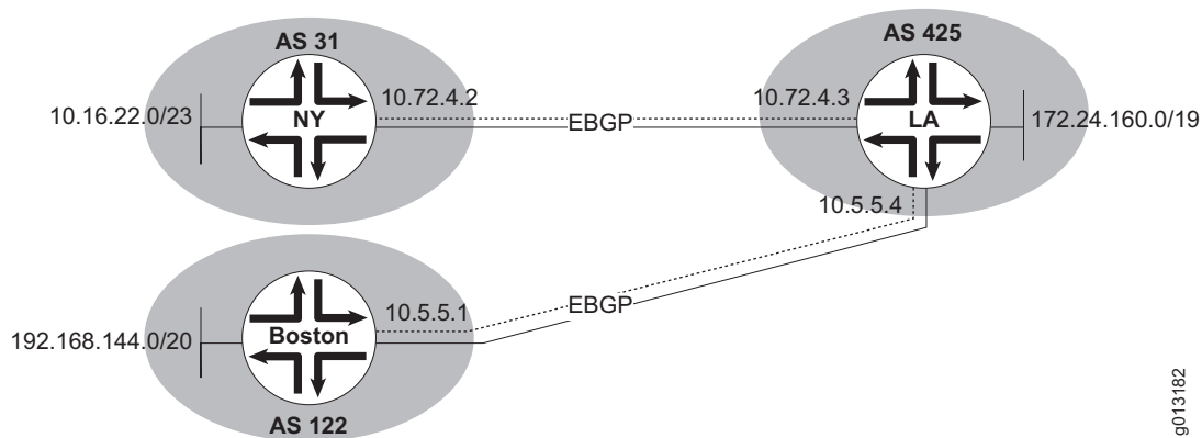
Figure 26: Communities
