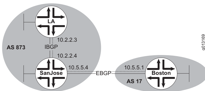
Figure 10: Configuring Neighbors
