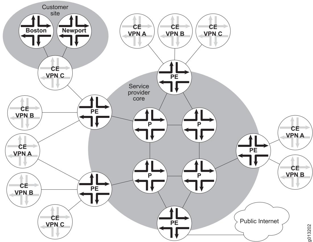
Figure 68: BGP/MPLS VPN Scenario
