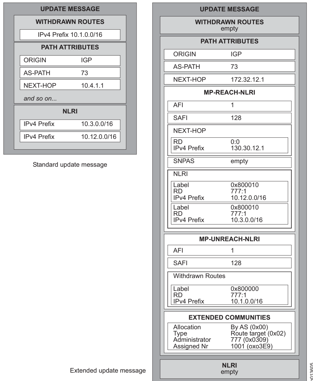
Figure 71: Standard and Extended BGP Update Messages
