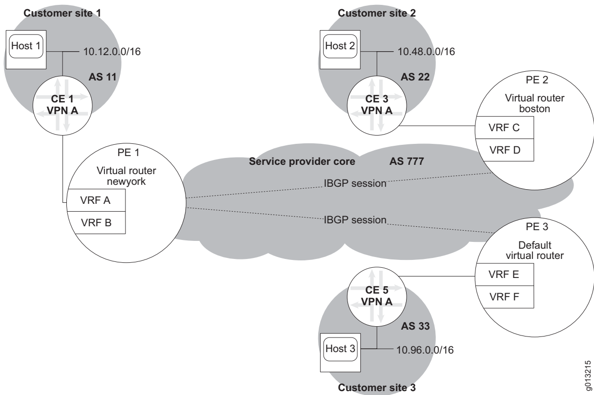
Figure 89: Hub-and-Spoke VPN
