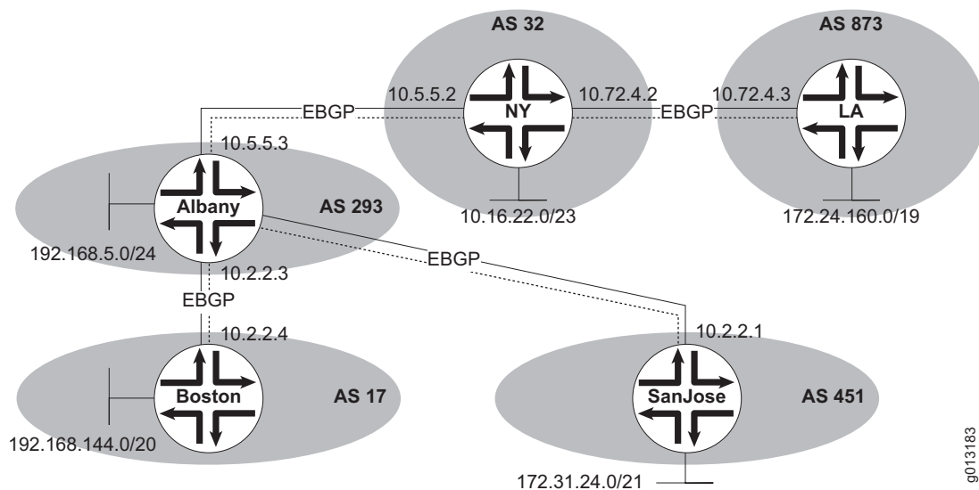
Figure 27: Community Lists
