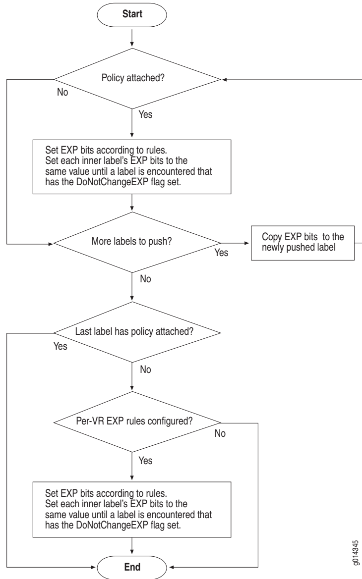
Figure 63: Flow for Setting EXP Bits for All Pushed Labels
