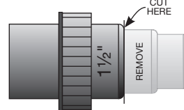
Hosetail ready for 1 1/2" tubing
