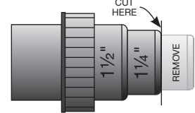
Hosetail ready for 1 1/4" tubing
