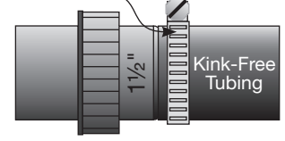
Installation of stainless steel hose clamp
