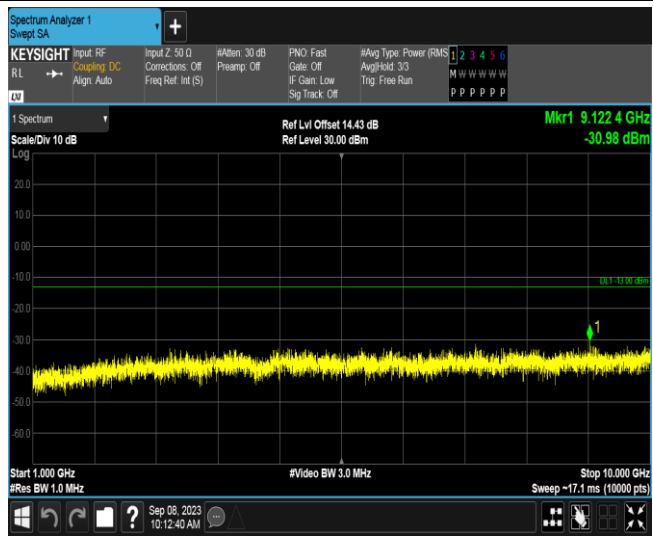
Band12-5MHz-16QAM-23095-1RB#0-Range2:1000~10000MHz
