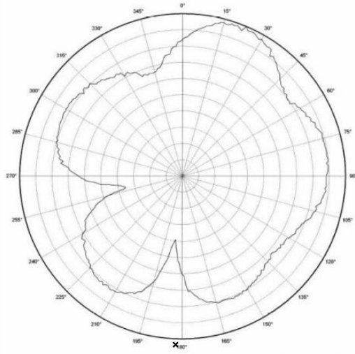
Vertical Polarization usb XZ
