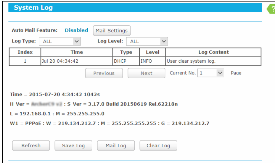
Figure 5-116 System Log
