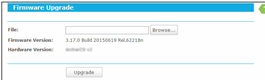
Figure 5-111 Firmware Upgrade
