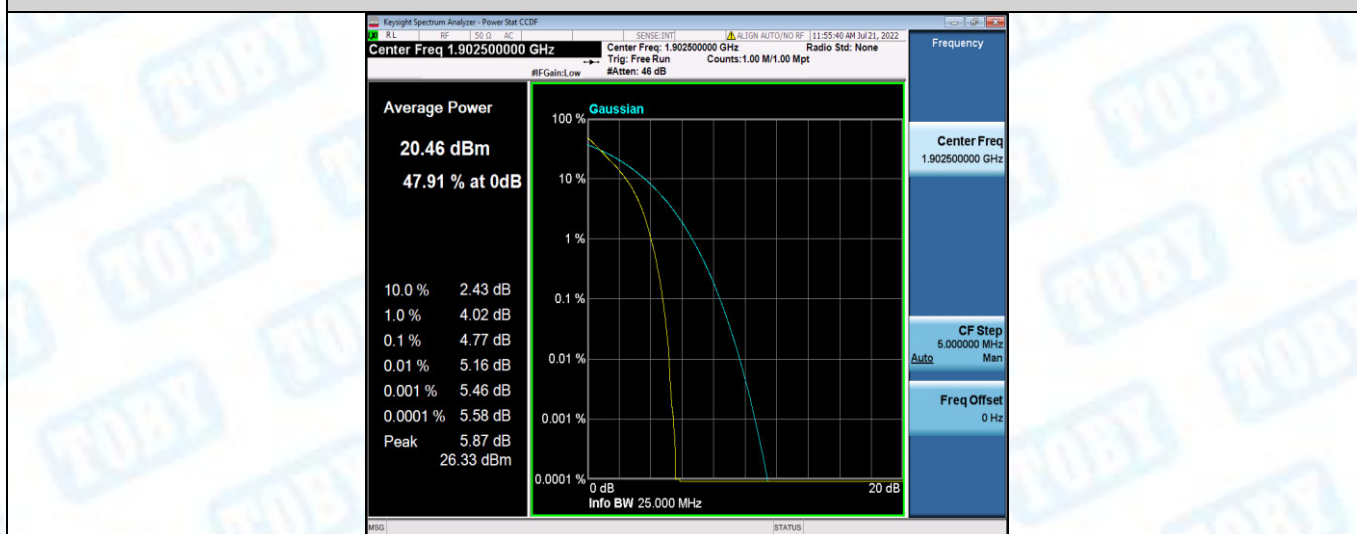
Band2-15MHz-16QAM-18675-1RB#0
