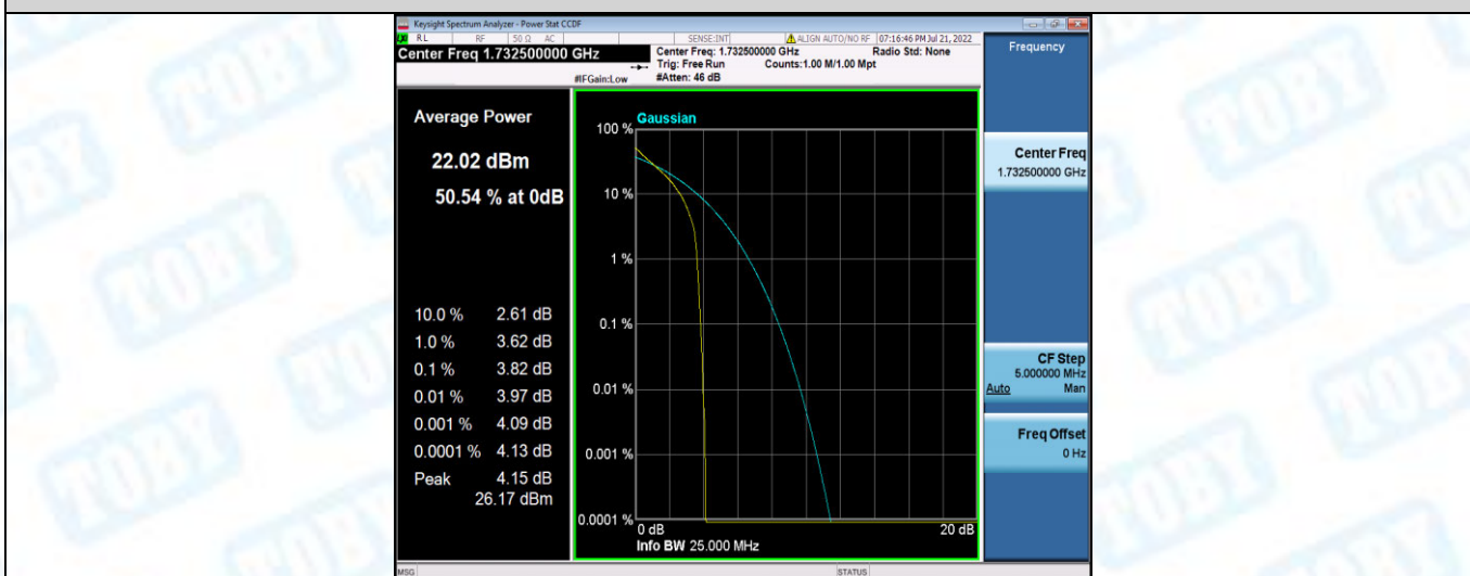
Band4-1.4MHz-QPSK-20175-6RB#0
