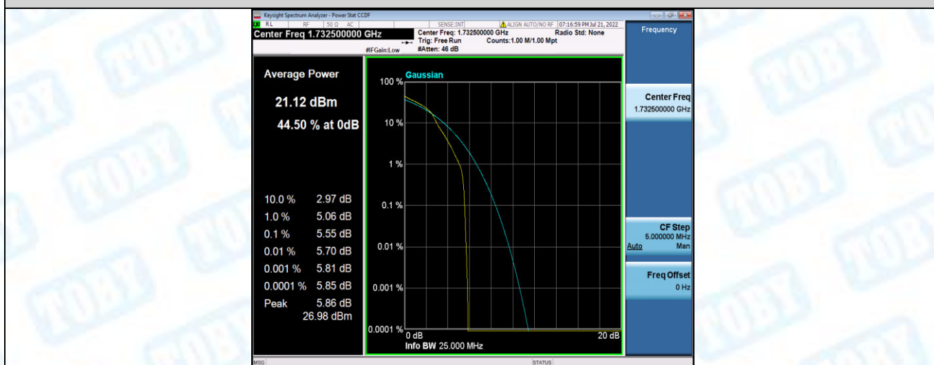
Band4-1.4MHz-16QAM-20175-6RB#0
