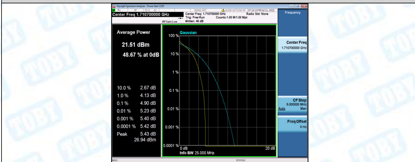
Band4-1.4MHz-QPSK-20175-1RB#0
