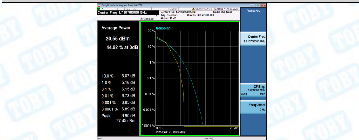
Band4-1.4MHz-16QAM-20175-1RB#0
