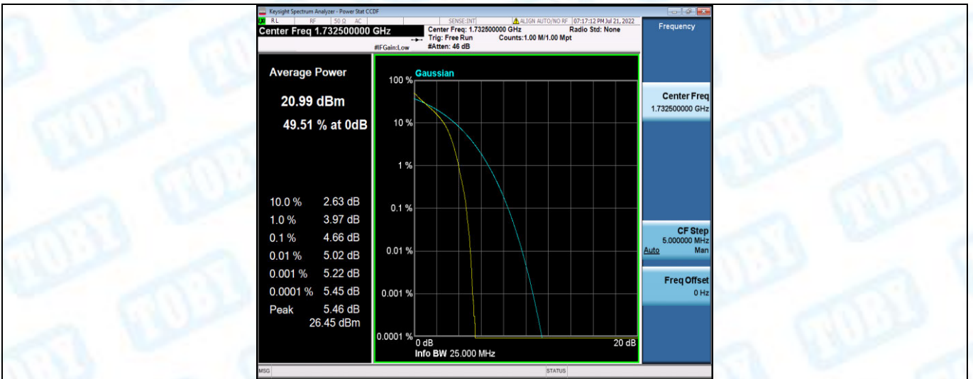
Band4-1.4MHz-QPSK-20393-1RB#0
