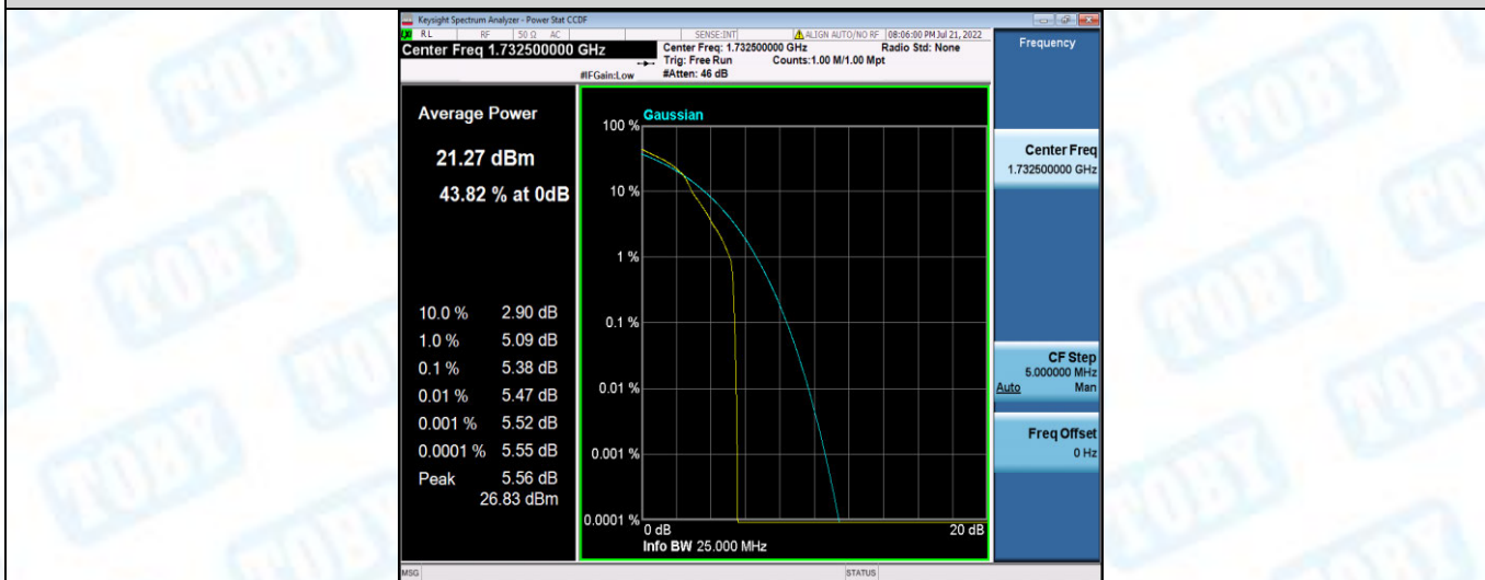
Band4-5MHz-16QAM-20175-25RB#0
