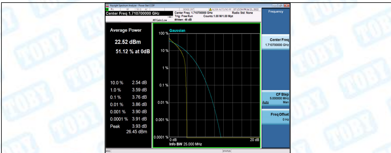
Band4-1.4MHz-QPSK-19957-6RB#0
