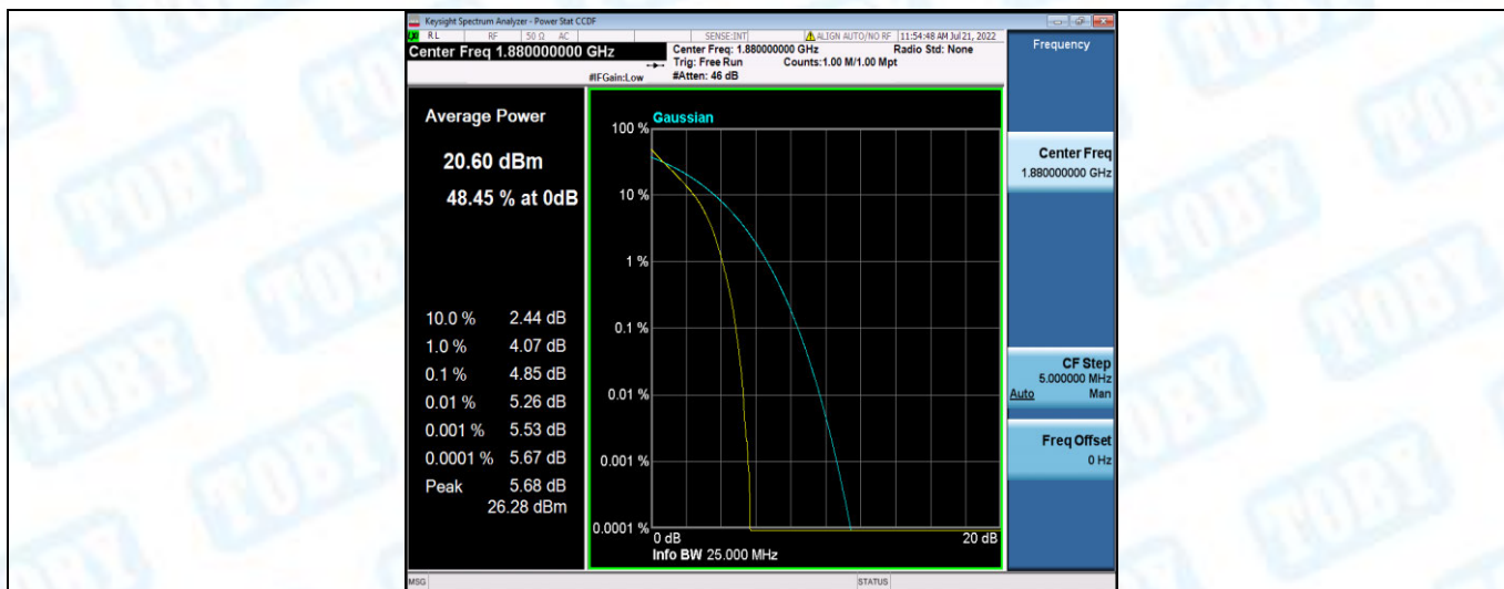
Band2-15MHz-QPSK-19125-1RB#0
