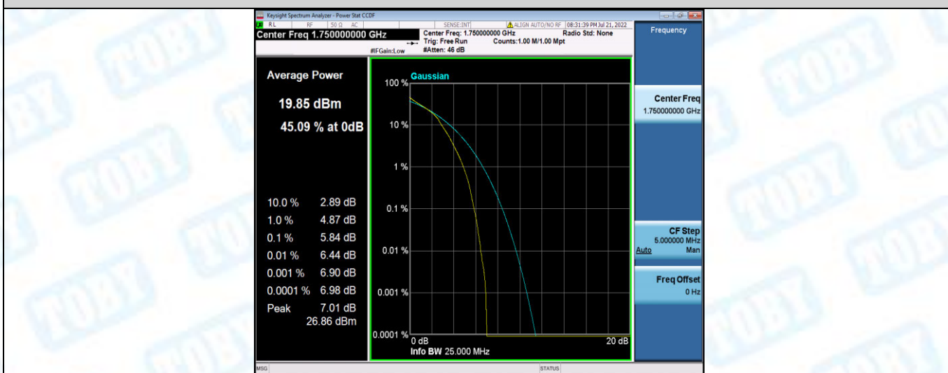
Band4-15MHz-QPSK-20025-1RB#0
