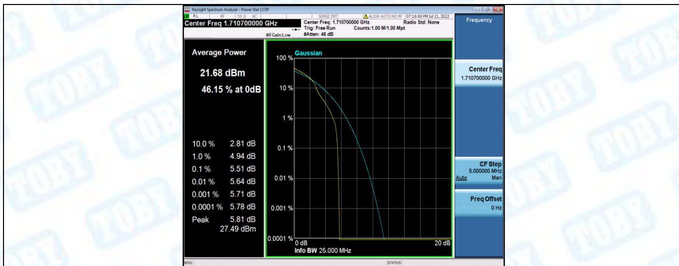
Band4-1.4MHz-16QAM-19957-6RB#0
