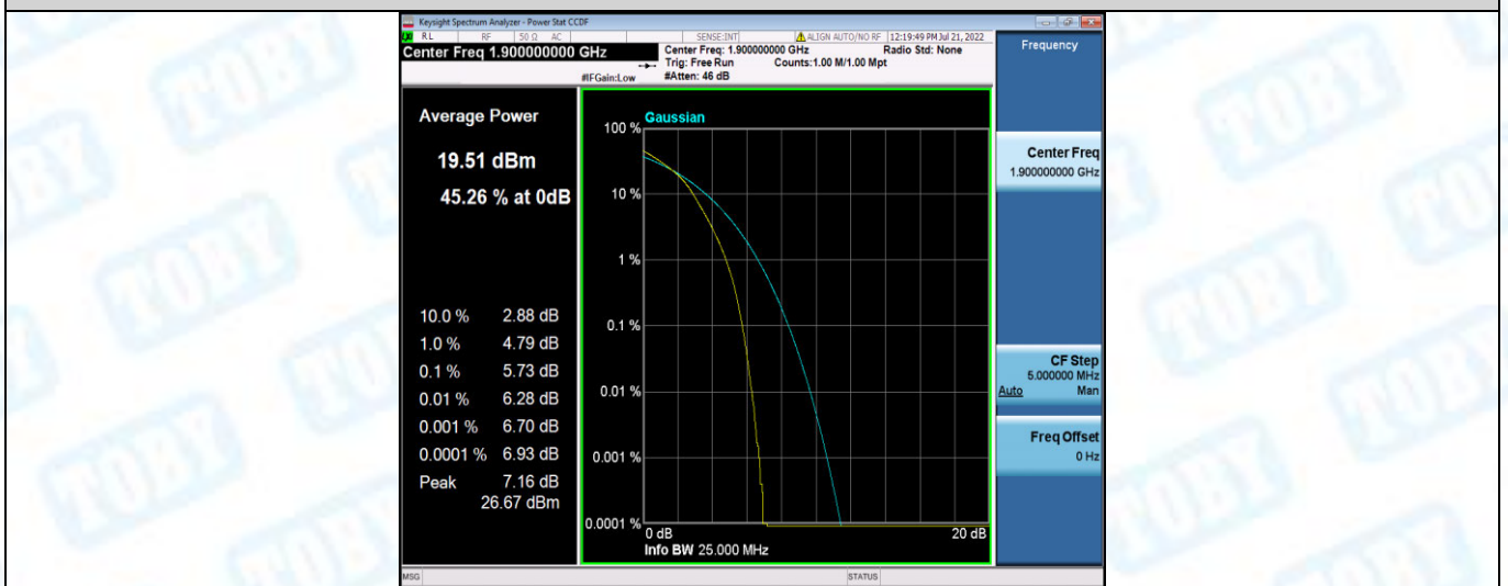
Band4-1.4MHz-QPSK-19957-1RB#0
