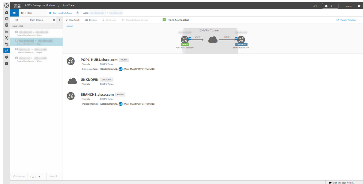
Figure 7: Path Trace Window Showing DMVPN Tunnel
