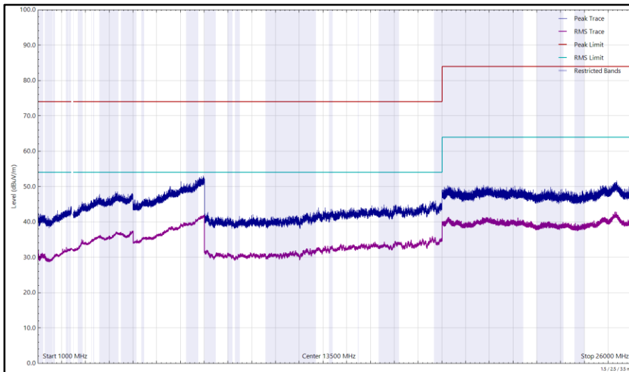
Figure 189 - 2440 MHz (CH17), LE1M, ePA, Core 1, 1 GHz to 26 GHz, Horizontal
