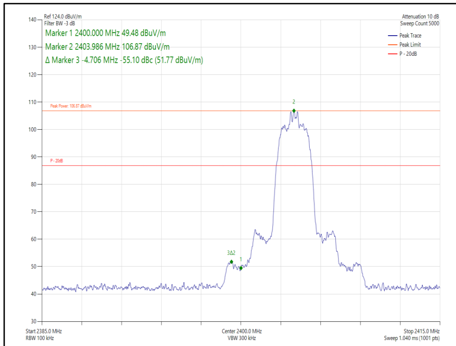
Figure 210 Core 2- GFSK/DH4- 2404 MHz – Band Edge Frequency 2400.0 MHz
