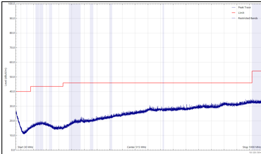
Figure 188 - 2440 MHz (CH17), LE1M, ePA, Core 1, 30 MHz to 1 GHz, Horizontal (Peak)
