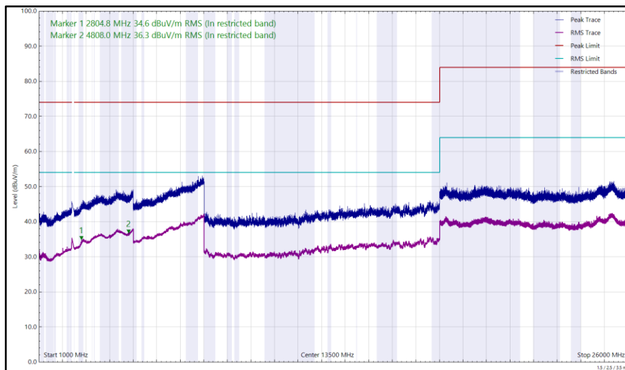
Figure 186 - 2404 MHz (CH0), LE1M, ePA, Core 1, 1 GHz to 26 GHz, Horizontal
