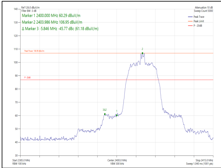
Figure 215 Core 2- GFSK/DH8- 2404 MHz – Band Edge Frequency 2400.0 MHz
