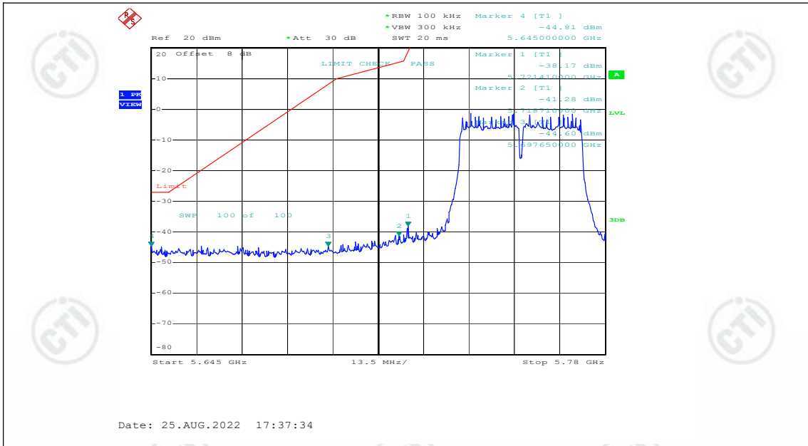
11AC40SISO_Ant1_Low_5755
