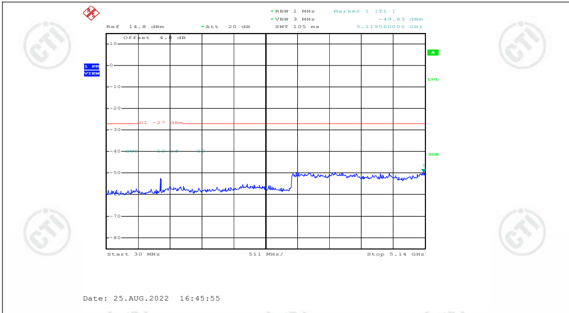
11AC20SISO_Ant1_5200_30~5140
