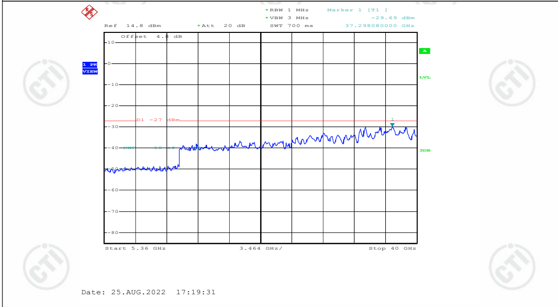
11AC40SISO_Ant1_5190_5360~40000
