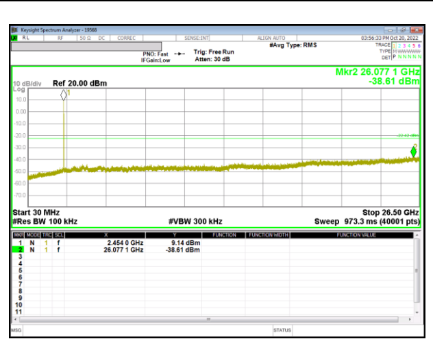
Out-Of-Band 11 Channel(0RU)
