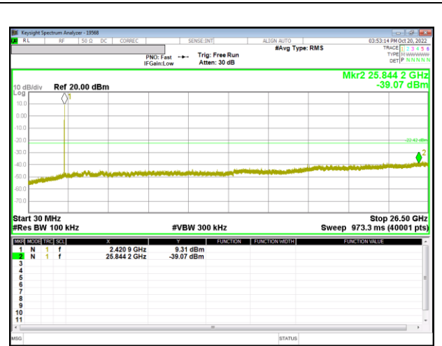
Out-Of-Band 1 Channel(8RU)
