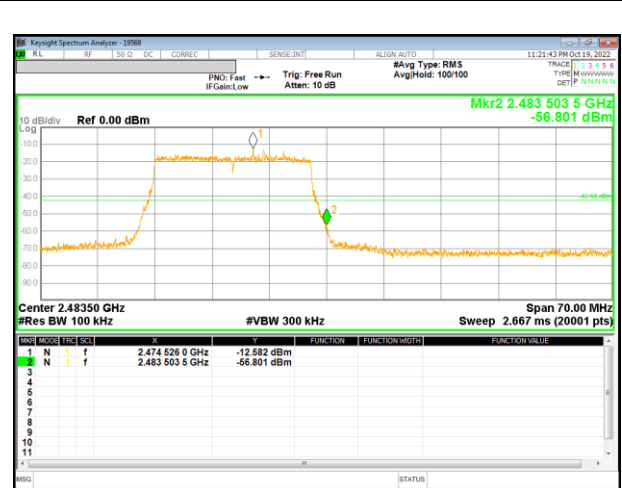
13 Channel Band-edge
