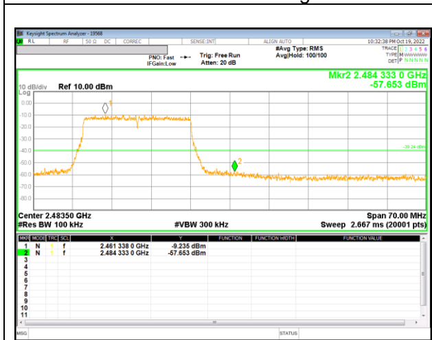
12 Channel Band-edge
