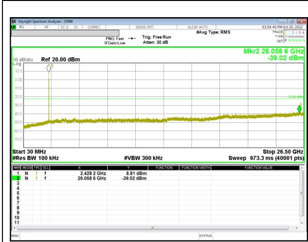
Out-Of-Band 6 Channel(0RU)
