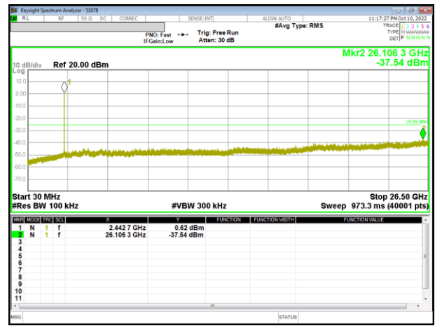
Out-Of-Band 6 Channel
