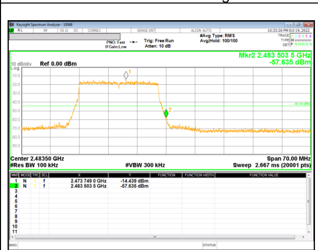
13 Channel Band-edge
