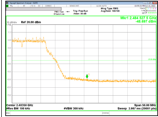
11 Channel Band-edge
