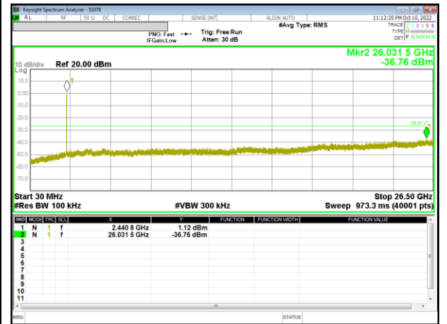
Out-Of-Band 6 Channel
