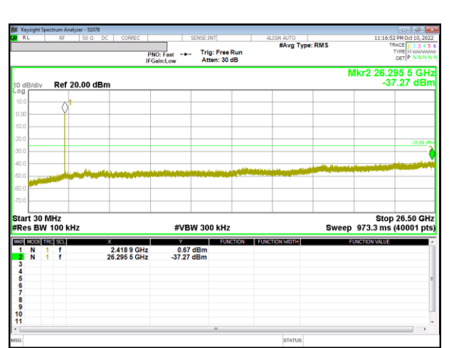
Out-Of-Band 1 Channel
