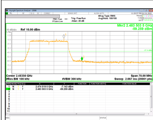
12 Channel Band-edge
