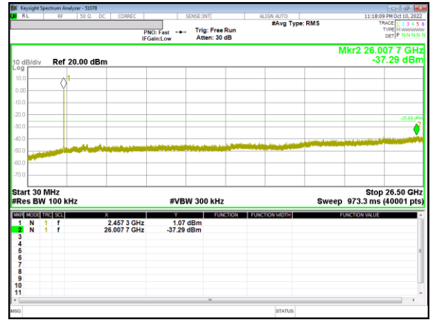
Out-Of-Band 11 Channel
