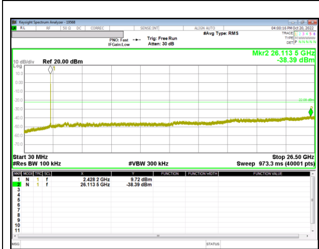
Out-Of-Band 6 Channel(0RU)
