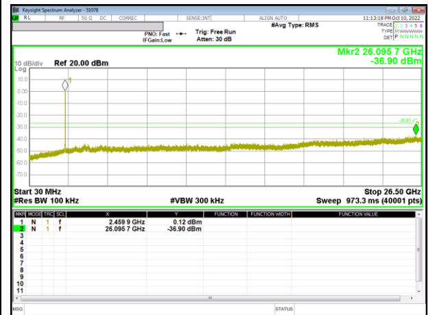
Out-Of-Band 1 Channel
