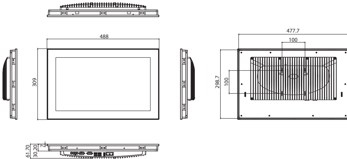
Panel Cutout Dimensions: 479.3 x 300.3 mm (18.87 x 11.82 in)
