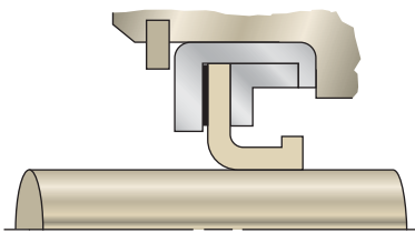
Elf Toe Lip without Spring
