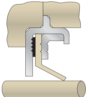
FlexiCase in gas turbine engine sump for high speed, 15,000 sfpm
