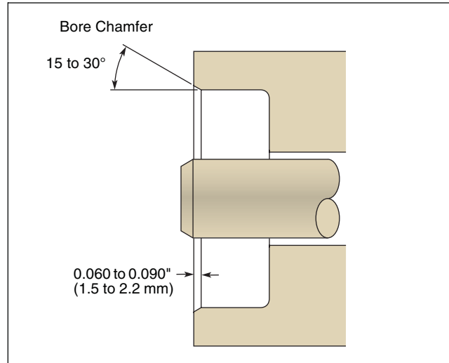
Figure 2-10. Housing Profile
