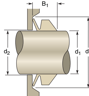
Assembly Dimensions
