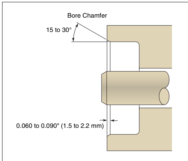
Figure 2-19. Housing Profile
