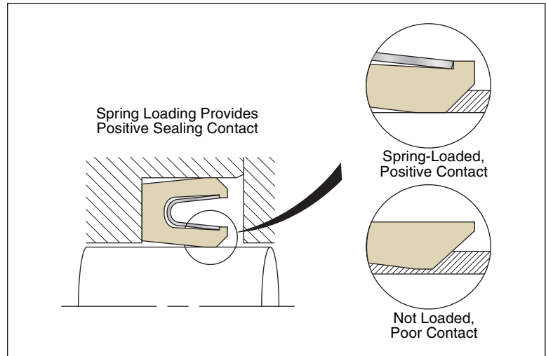
Figure 2-13. Spring Loading
