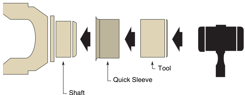
Quick Sleeve Installation
