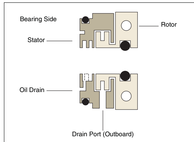
Figure 8-2. Position the Rotor Halves
