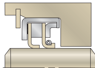
FlexiCase in Gland
