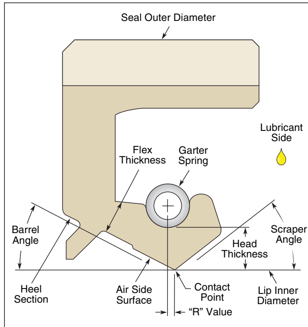
Figure 2-2. Seal Components
