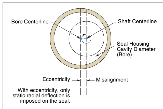
Figure 2-11. STBM
