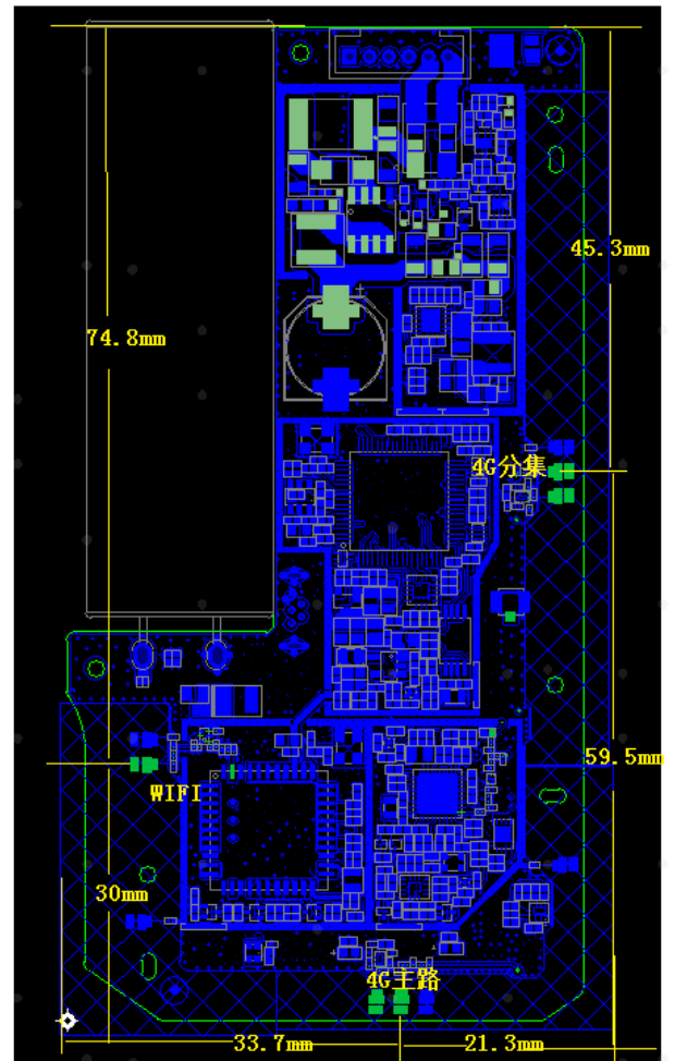
EUT Back View
