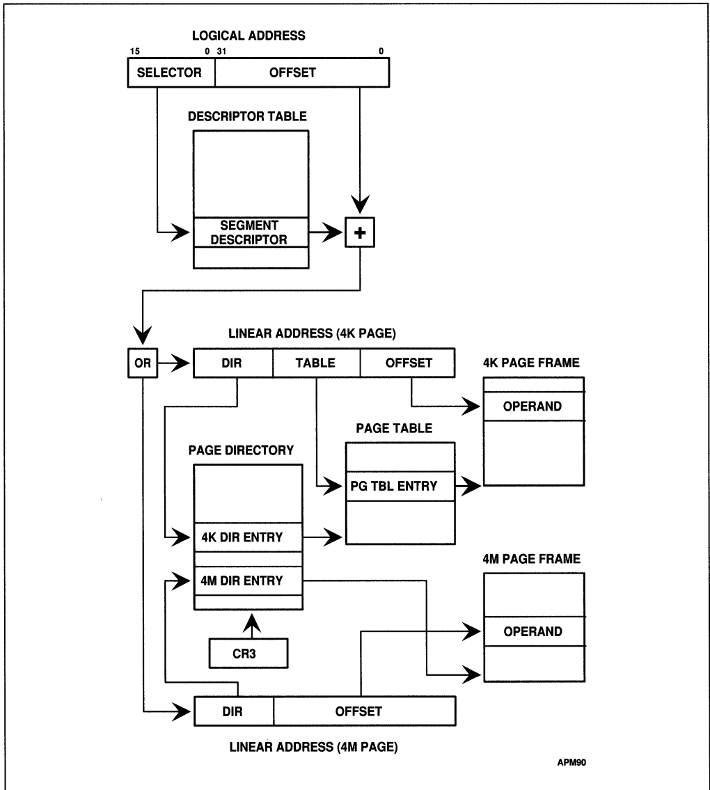
Figure 11-16. Combined Segment and Page Address Translation
