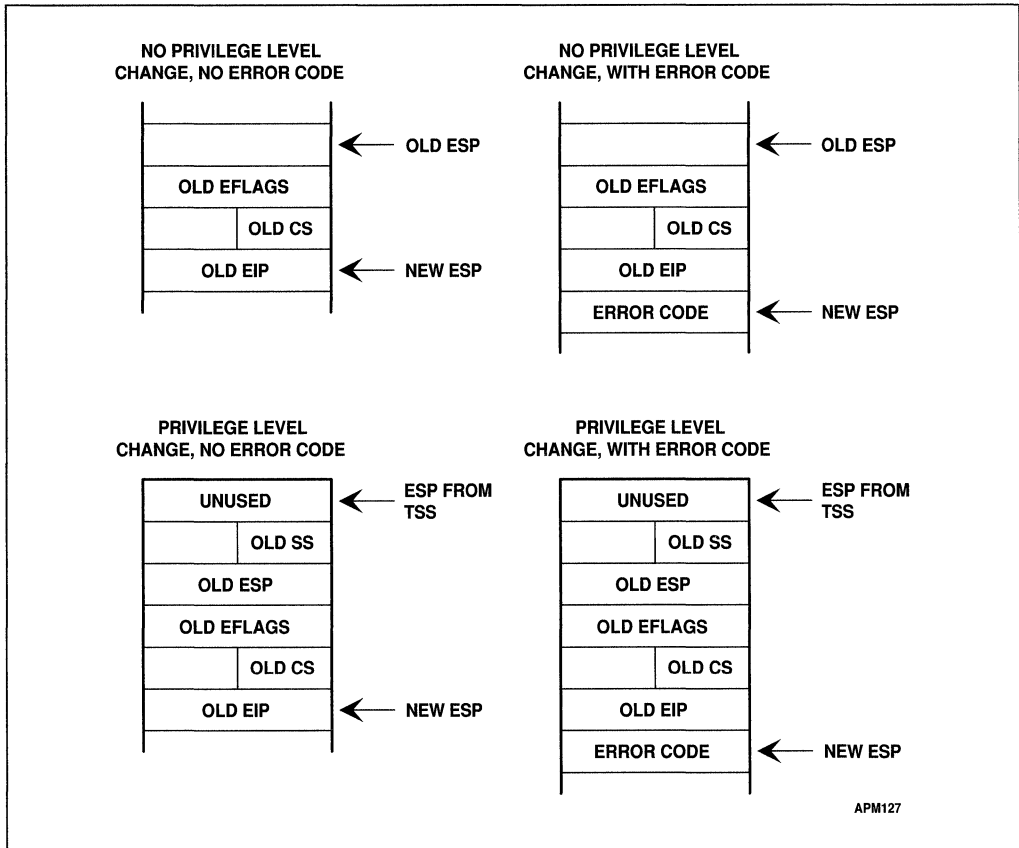
Figure 14-4. Stack Frame after Exception or Interrupt
