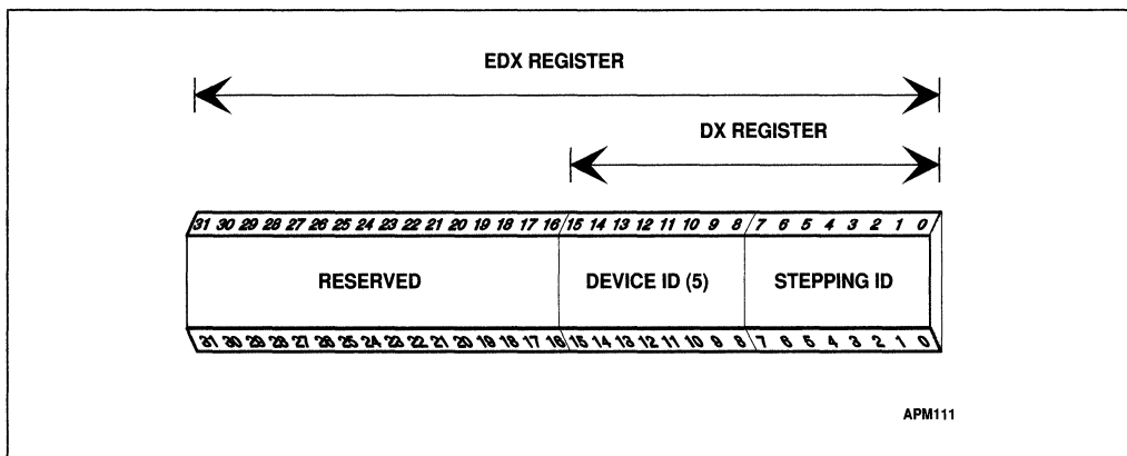
Figure 16-1. Contents of the EDX Register After Reset
