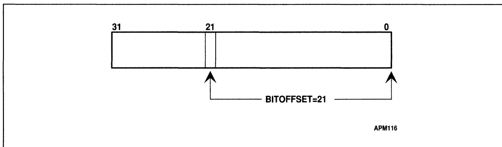
Figure 25-3. Bit Offset for BIT[EAX,21]
