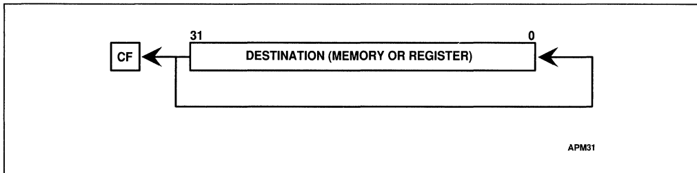
Figure 4-11. ROL Instruction
