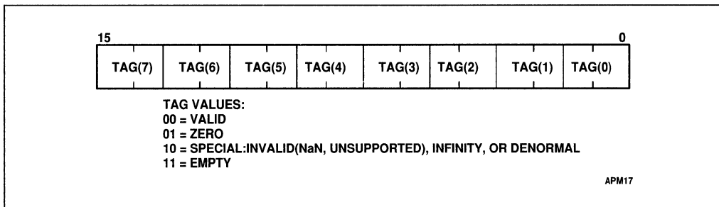
Figure 6-4. Tag Word Format
