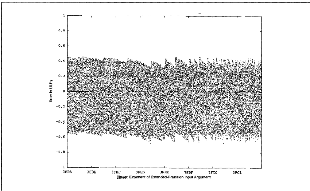
Figure G-20. Scatterplot for F2XM1 (3FBA-3FFE)
