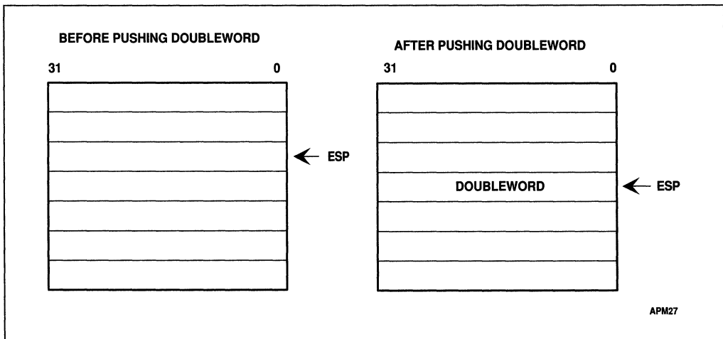
Figure 4-1. PUSH Instruction
