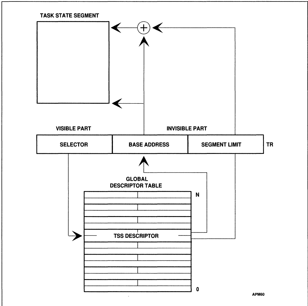
Figure 13-3. Task Register
