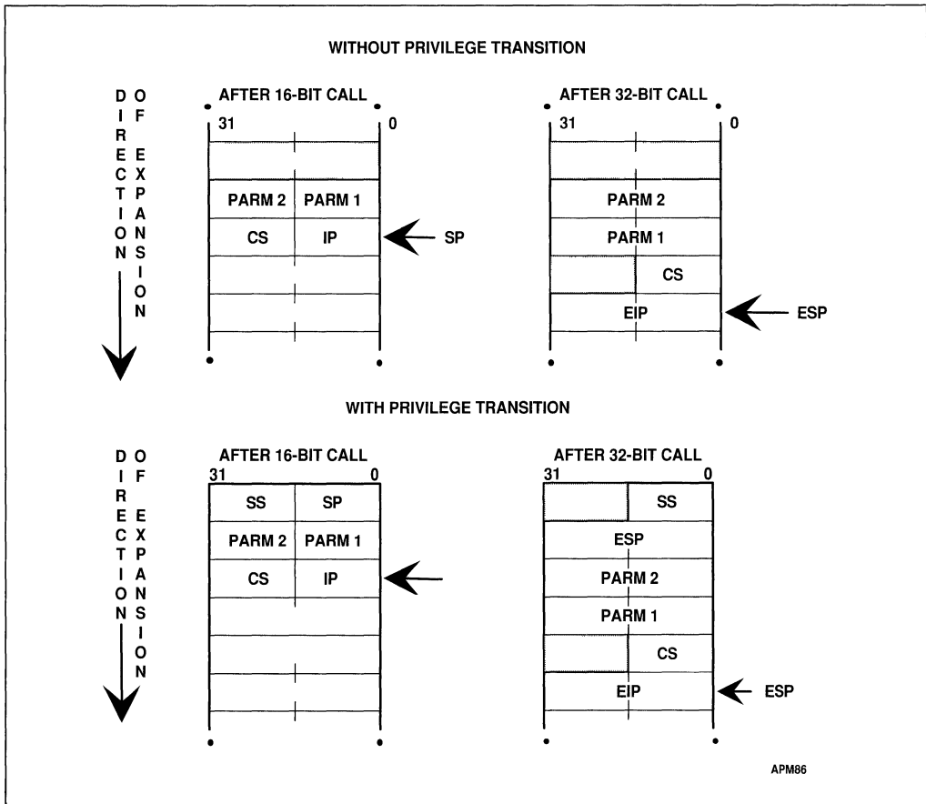
Figure 21-1. Stack After Far 16- and 32-Bit Calls
