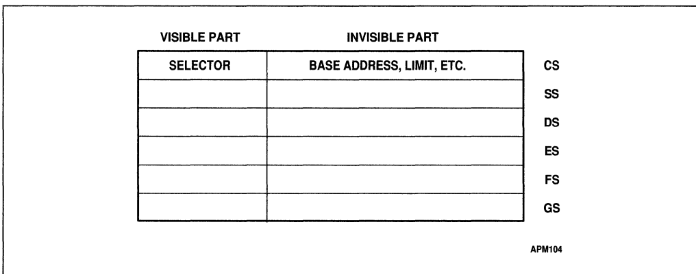
Figure 11-6. Segment Registers
