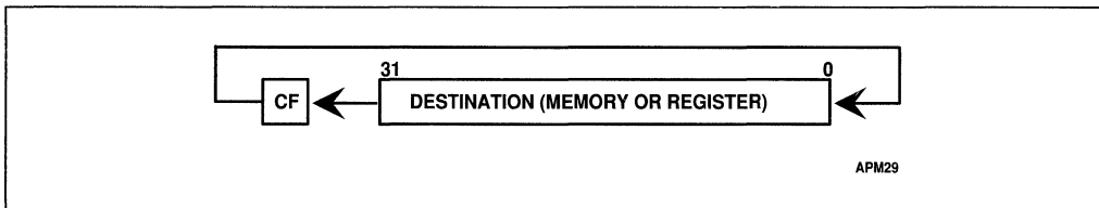
Figure 4-13. RCL Instruction
