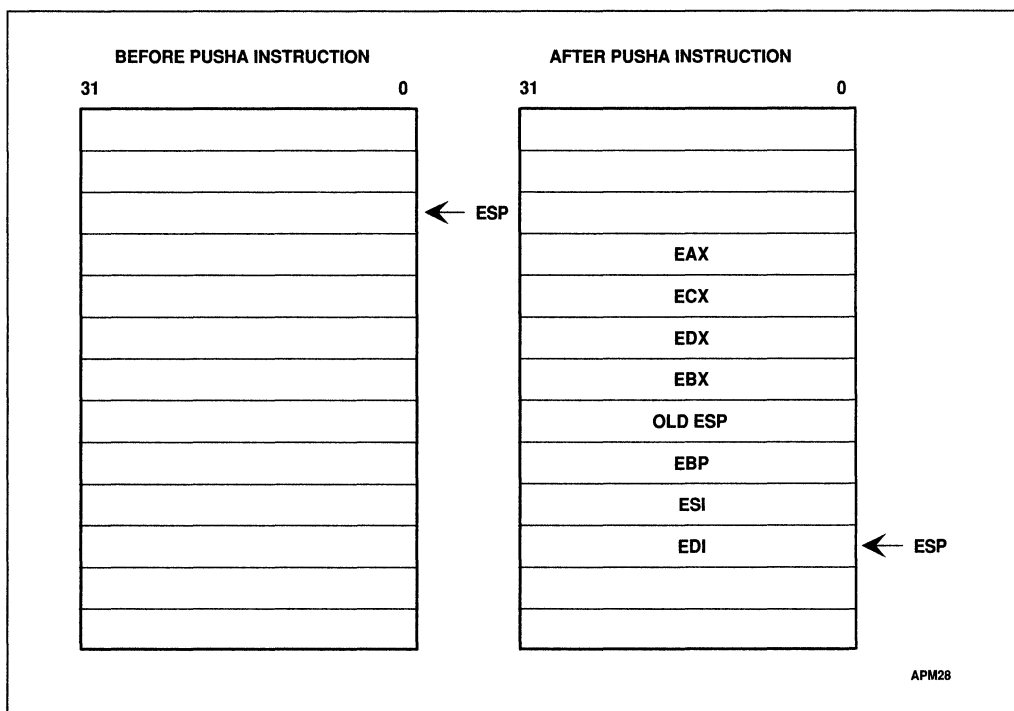
Figure 4-2. PUSHAs Instruction
