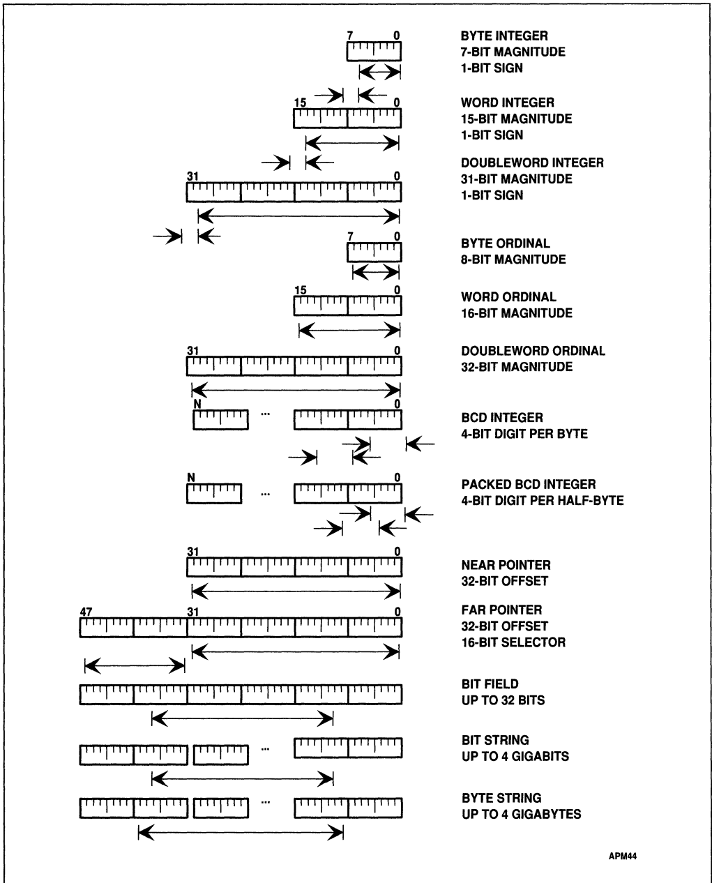
Figure 3-4. Data Types
