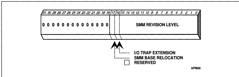
Figure 20-2. SMM Revision Identifier
