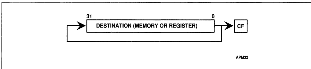
Figure 4-12. ROR Instruction
