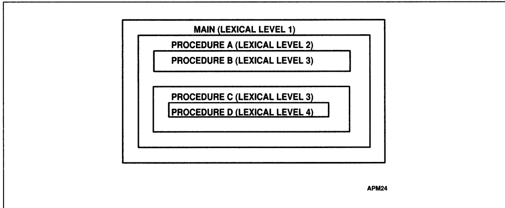
Figure 4-15. Nested Procedures
