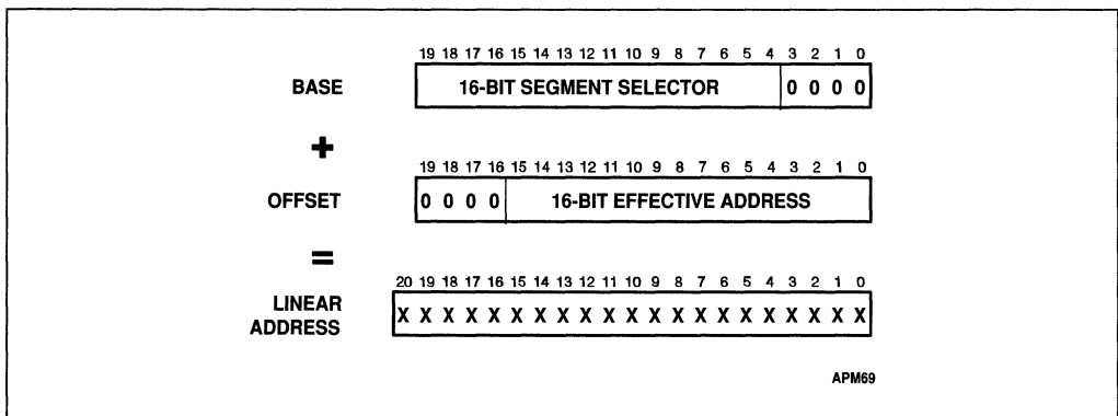
Figure 9-1. 8086 Address Translation
