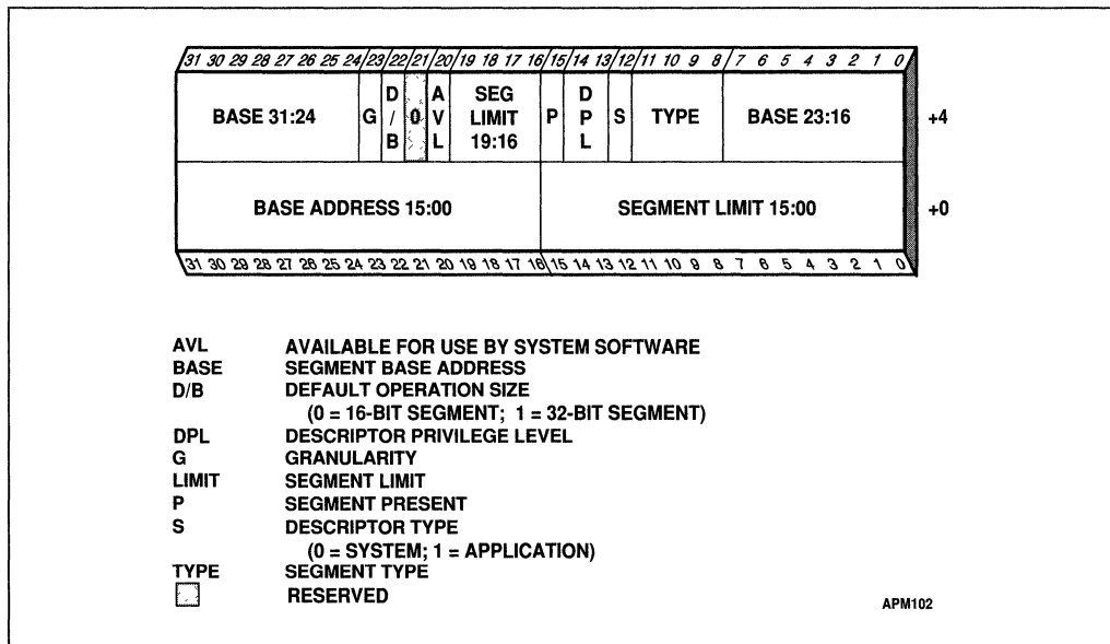
Figure 11-8. Segment Descriptors
