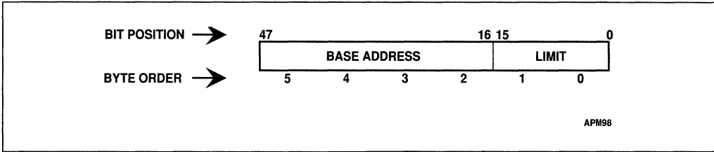
Figure 11-11. Pseudo-Descriptor Format
