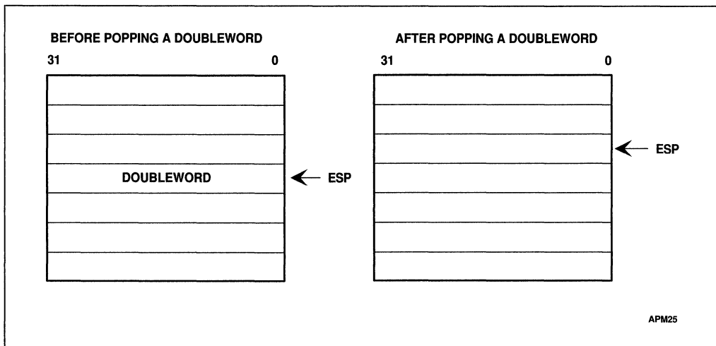
Figure 4-3. POP Instruction
