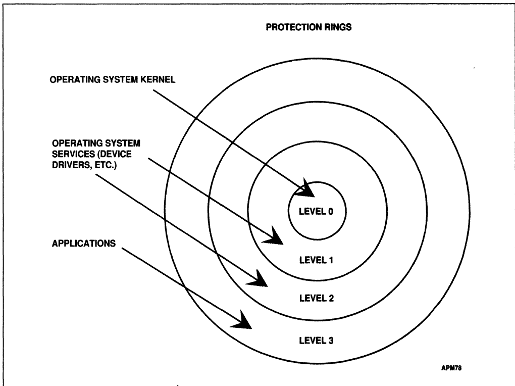
Figure 12-2. Protection Rings
