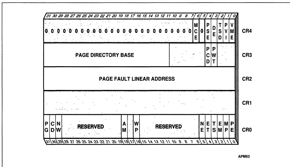
Figure 10-3. Control Registers
