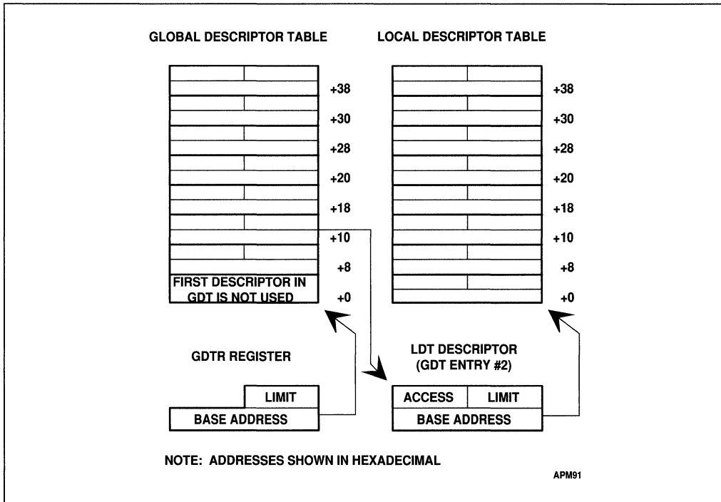
Figure 11-10. Descriptor Tables
