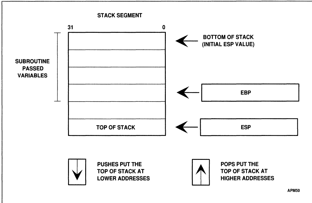
Figure 3-8. Stacks
