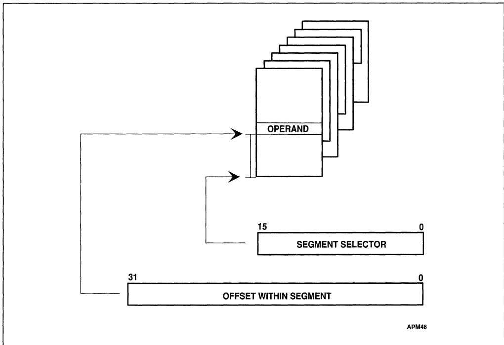
Figure 3-1. Segmented Addressing
