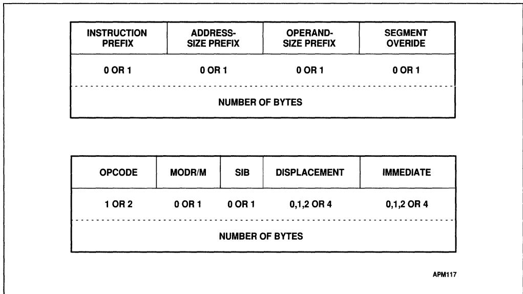
Figure 25-1. Instruction Format
