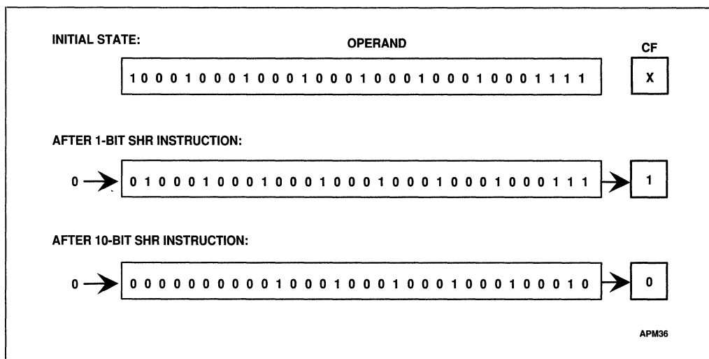
Figure 4-7. SHR Instruction
