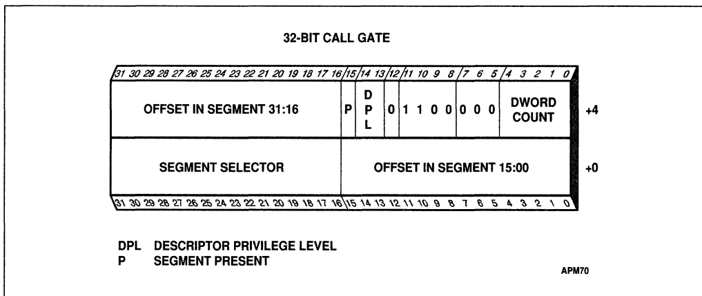
Figure 12-5. Call Gate
