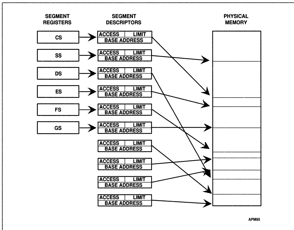
Figure 11-3. Multisegment Model
