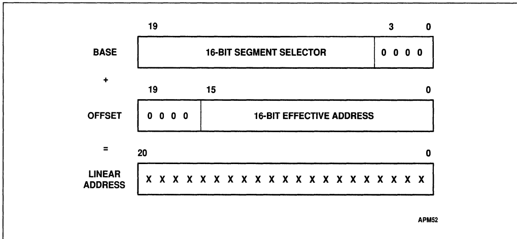
Figure 22-1. 8086 Address Translation
