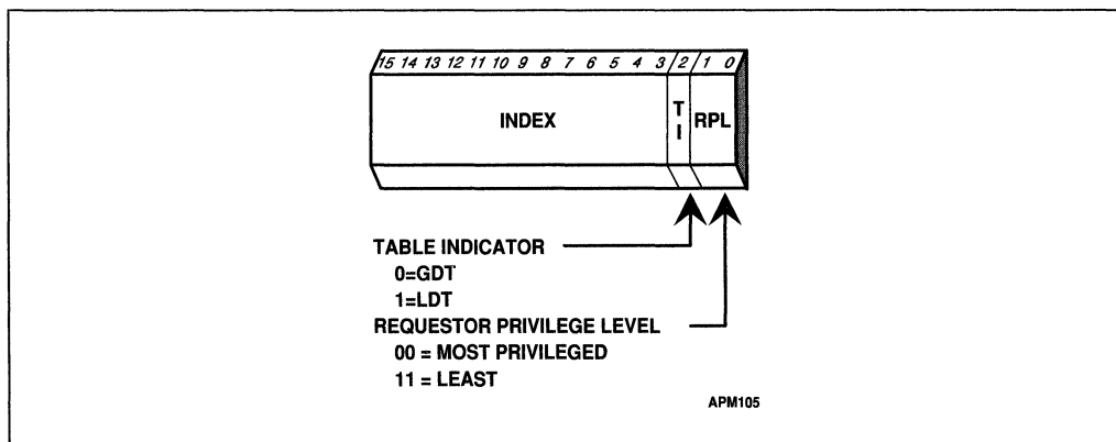
Figure 11-7. Segment Selector
