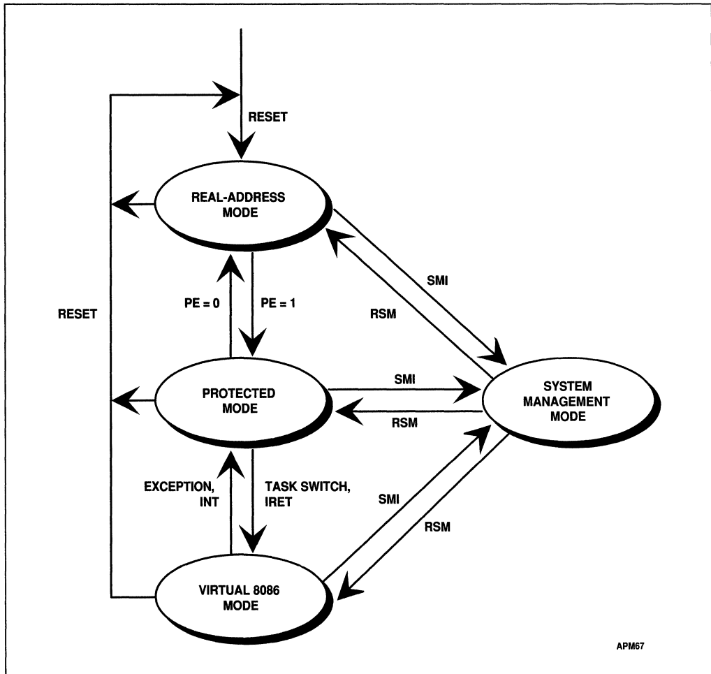
Figure 20-1. Mode State Transitions
