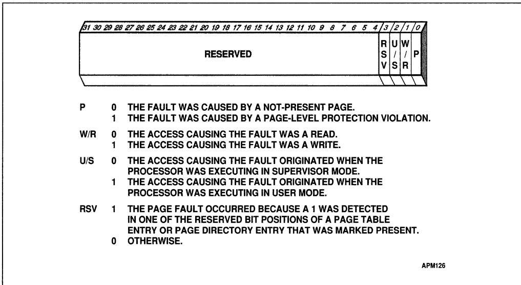
Figure 14-7. Page Fault Error Code
