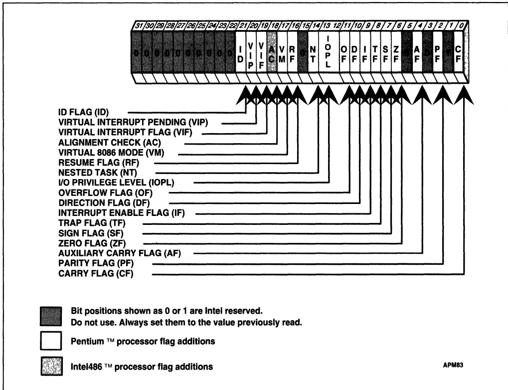
Figure 23-1. Pentium™ Processor EFLAGS Register
