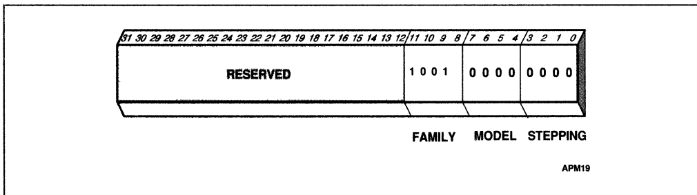
Figure 4-22. EAX Following the CPUID Instruction
