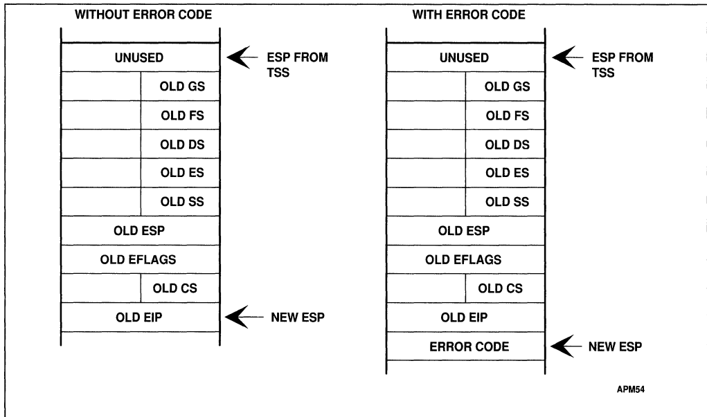
Figure 22-3. Privilege Level 0 Stack After Interrupt in Virtual-8086 Mode
