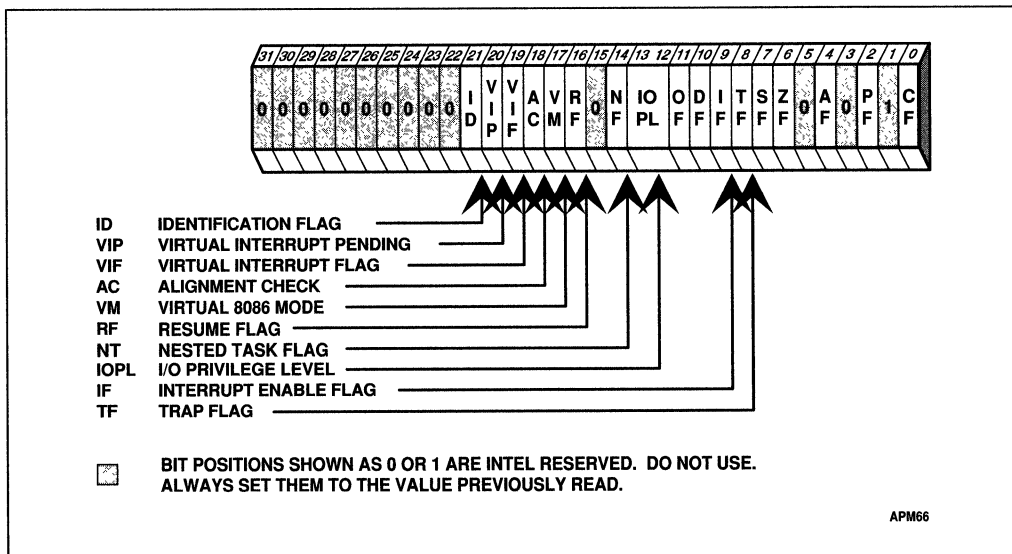
Figure 10-1. System Flags
