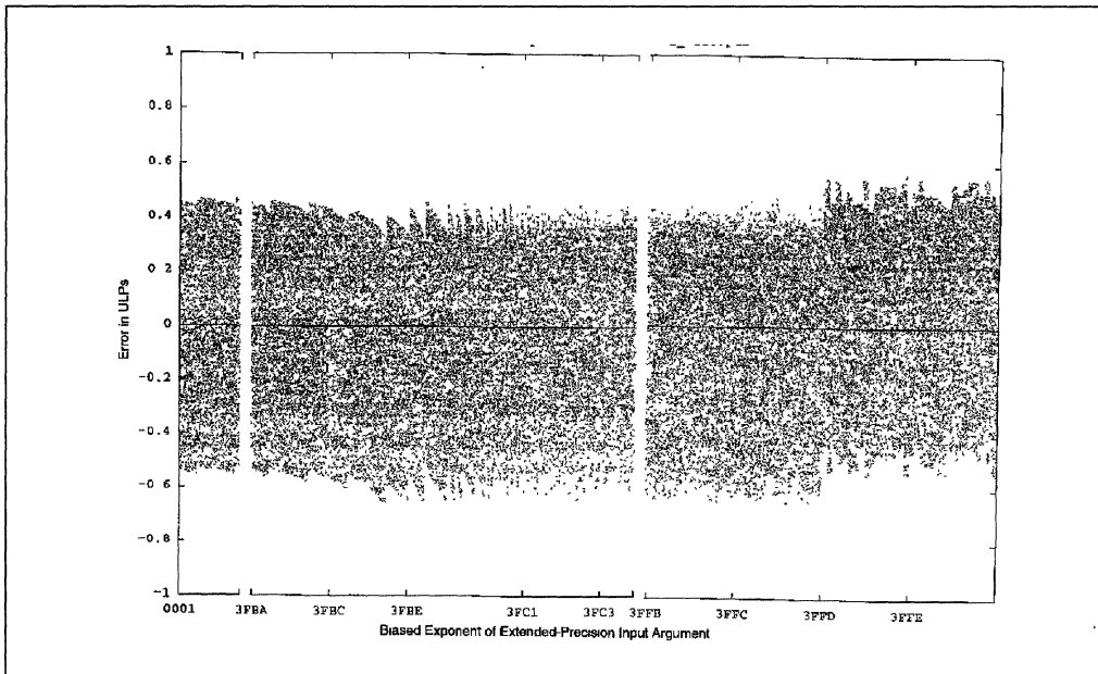
Figure G-19. Scatterplot for F2XM1 (0001-3FFE)
