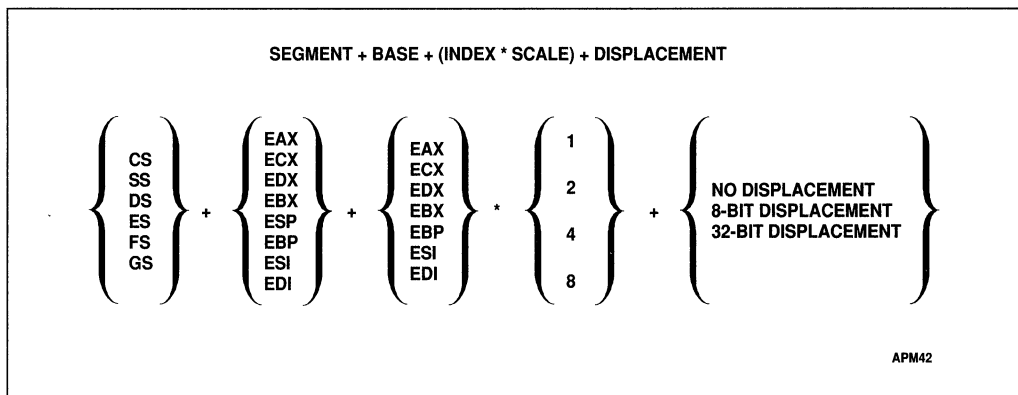
Figure 3-10. Effective Address Computation
