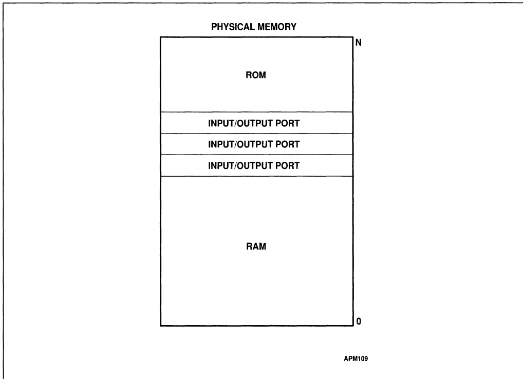
Figure 15-1. Memory-Mapped I/O
