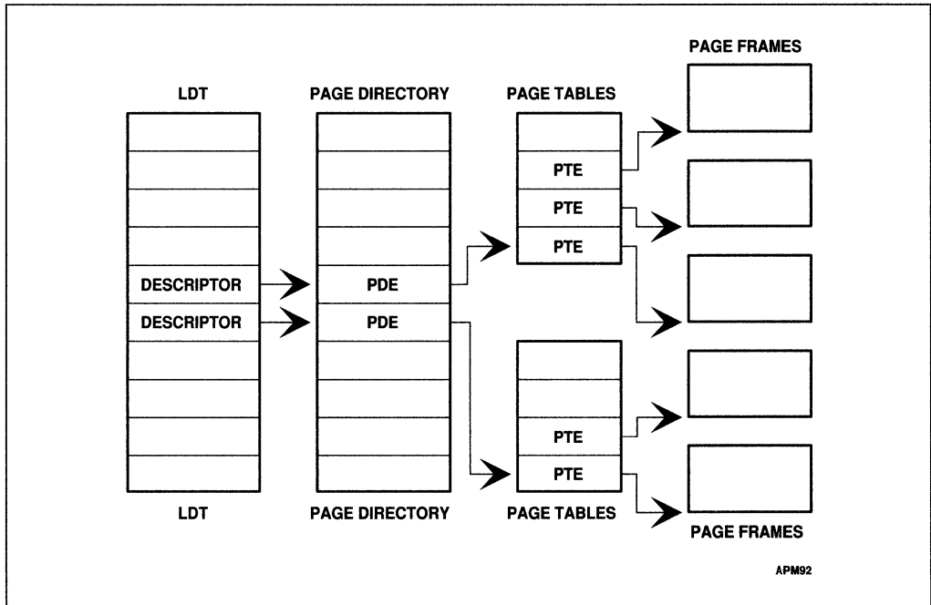
Figure 11-17. Each Segment Can Have Its Own Page Table
