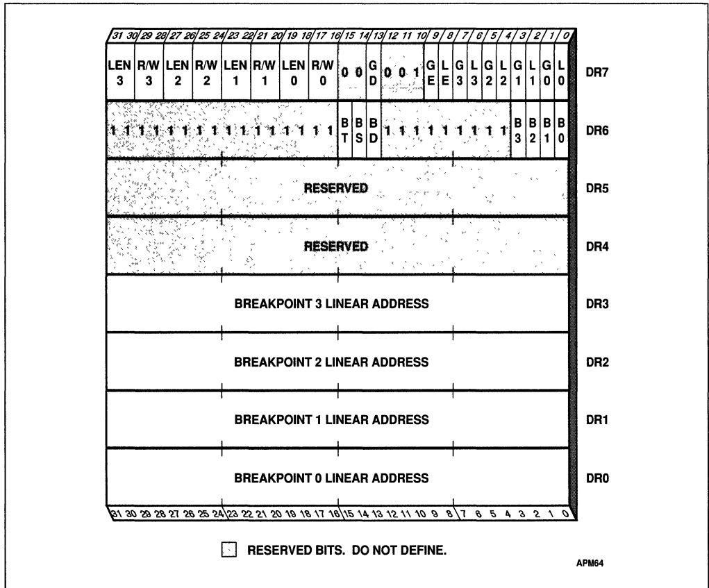
Figure 10-4. Debug Registers
