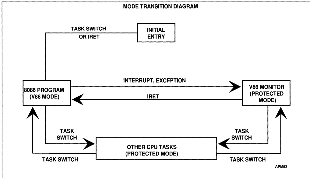
Figure 22-2. Entering and Leaving Virtual-8086 Mode
