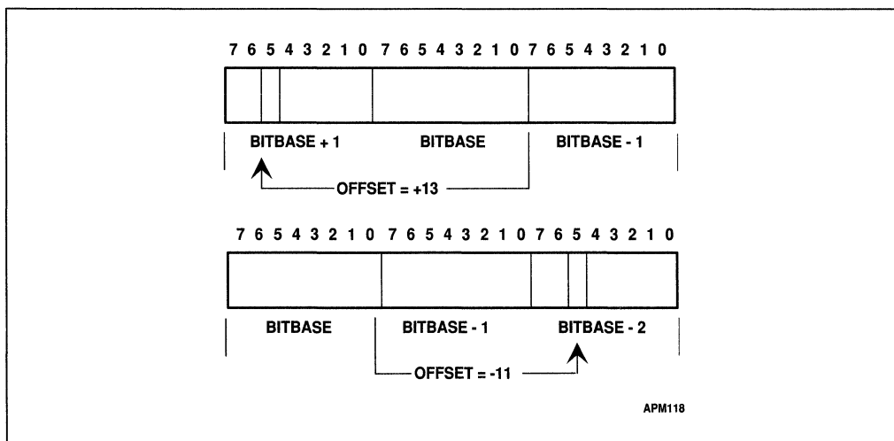
Figure 25-4. Memory Bit Indexing
