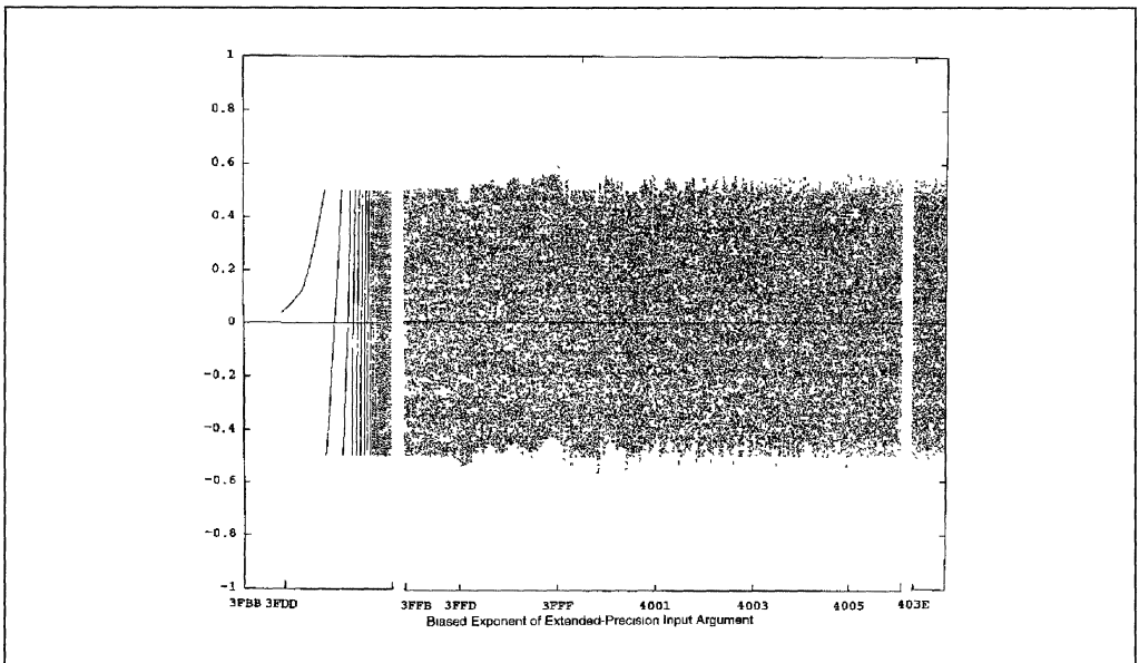
Figure G-10. Scatterplot for FSINCOS (COS, 3FBB-403E)
