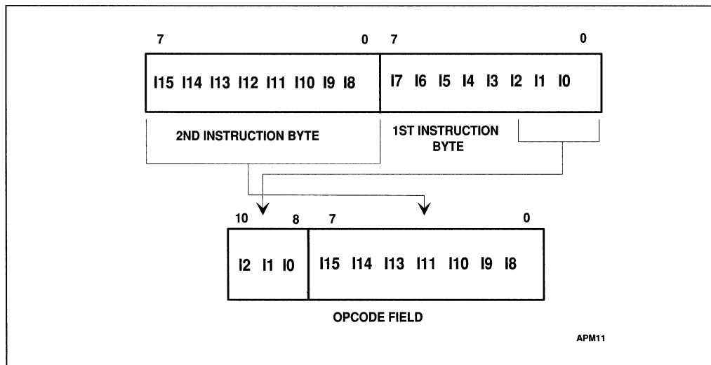
Figure 6-5. Opcode Field
