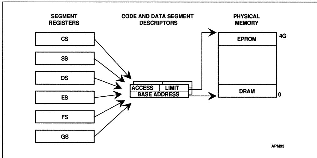
Figure 11-1. Flat Model
