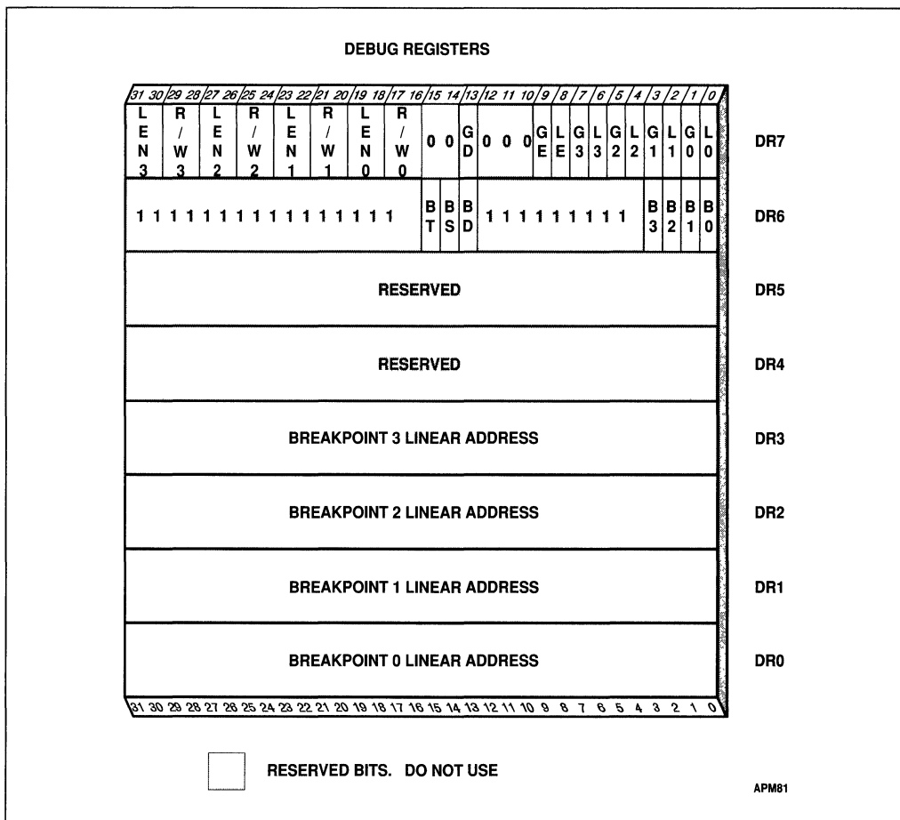
Figure 17-1. Debug Registers
