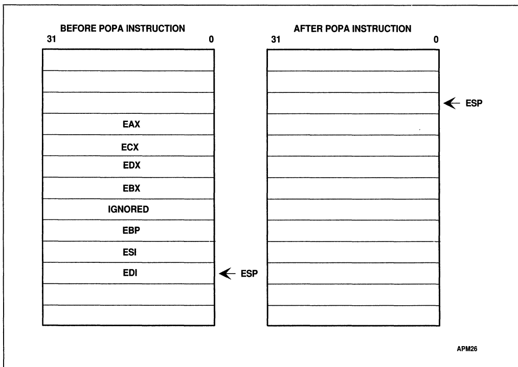
Figure 4-4. POPA Instruction
