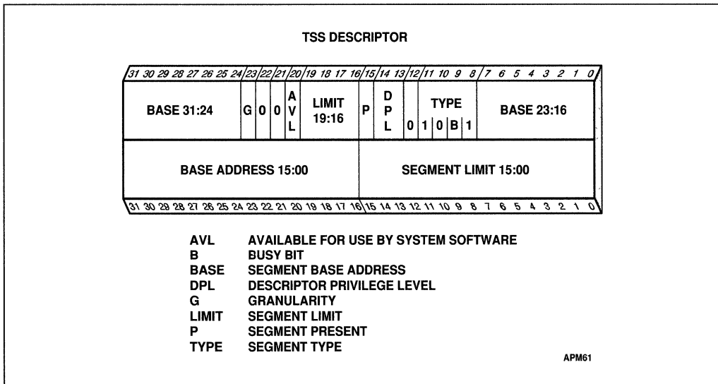
Figure 13-2. TSS Descriptor
