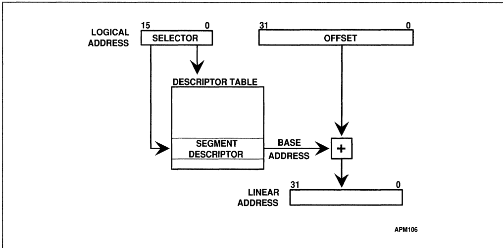
Figure 11-5. Segment Translation
