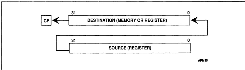
Figure 4-9. SHLD Instruction
