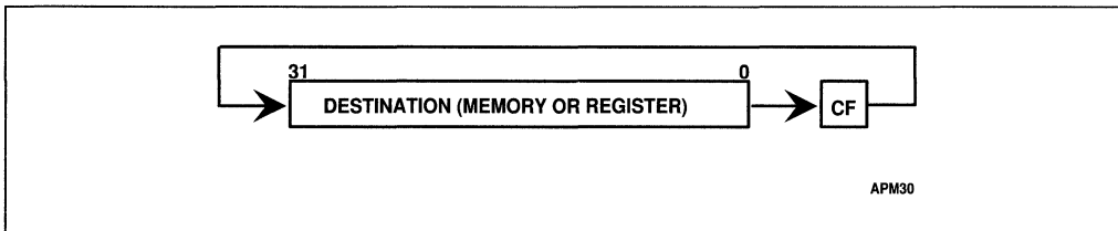
Figure 4-14. RCR Instruction
