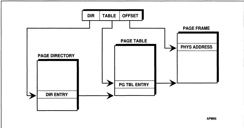
Figure 11-13. Page Translation
