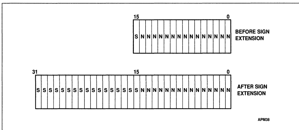
Figure 4-5. Sign Extension
