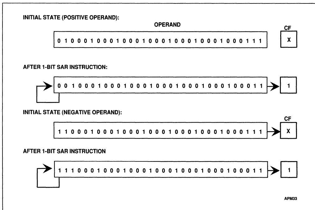
Figure 4-8. SAR Instruction
