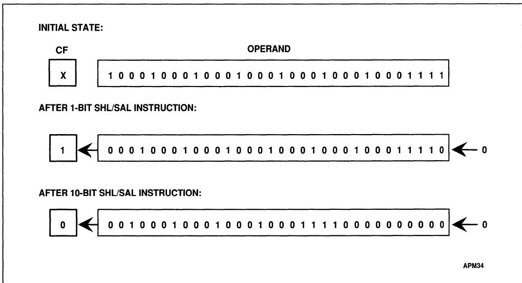
Figure 4-6. SHL/SAL Instruction
