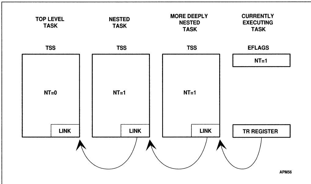
Figure 13-6. Nested Tasks
