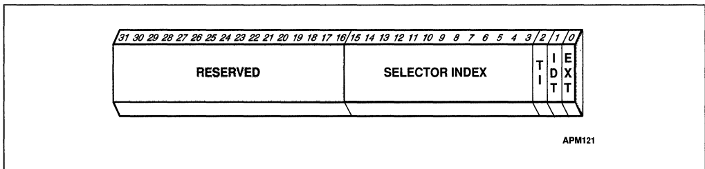
Figure 14-6. Error Code
