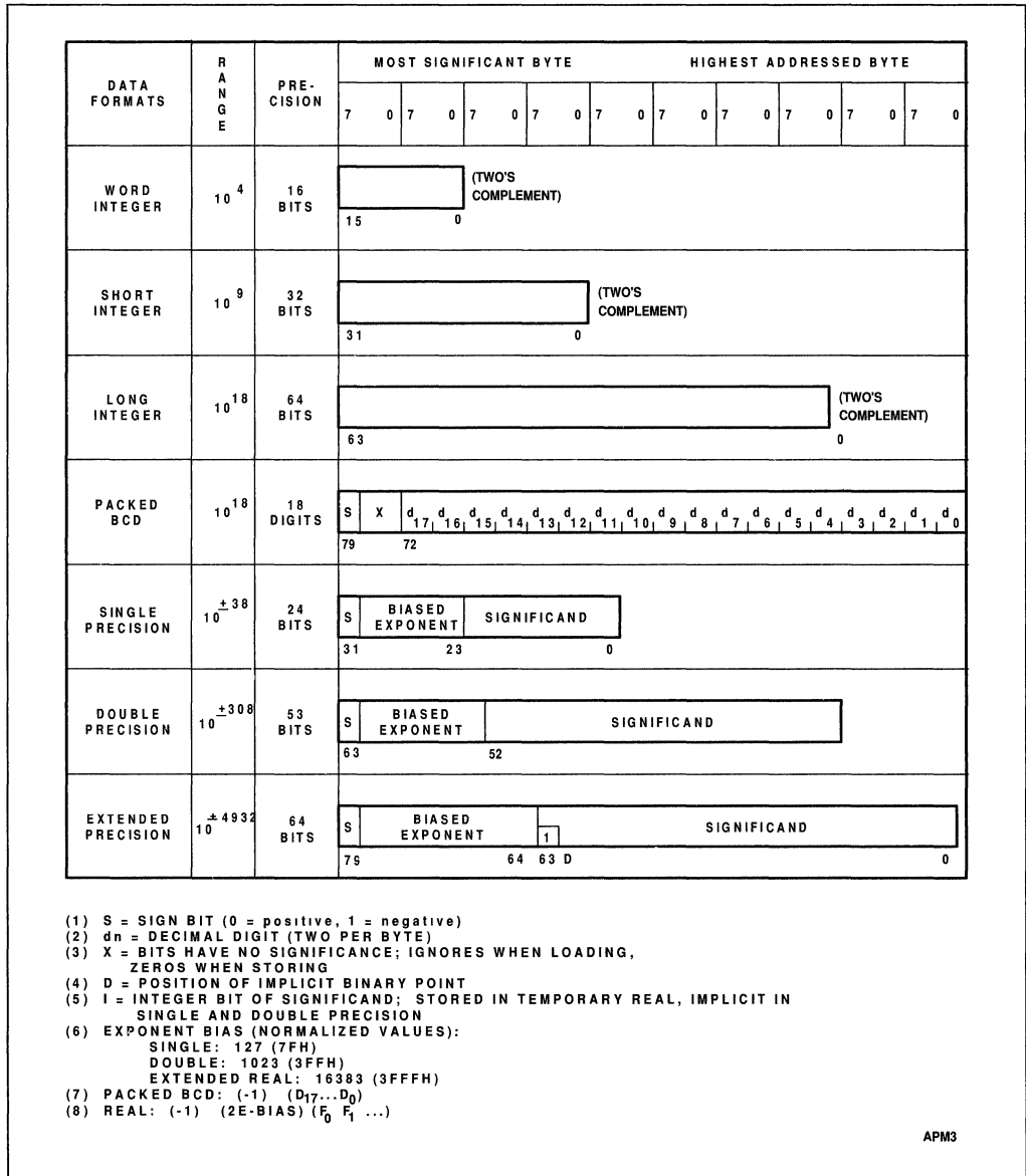
Figure 6-11. Numerical Data Formats
