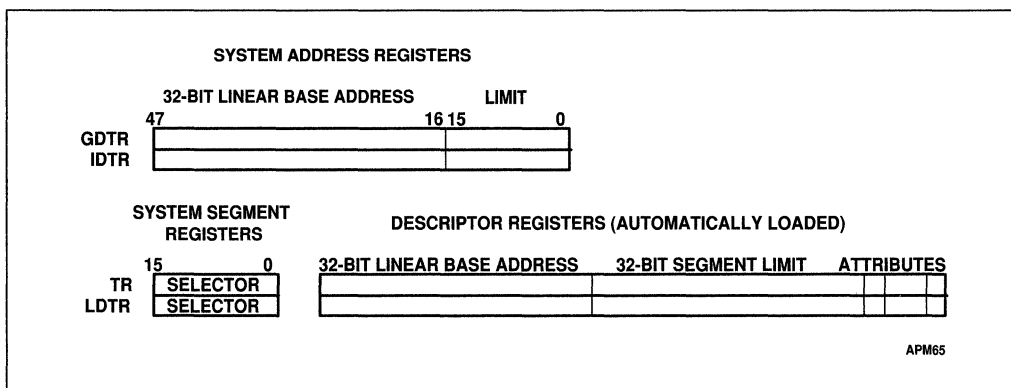
Figure 10-2. Memory Management Registers
