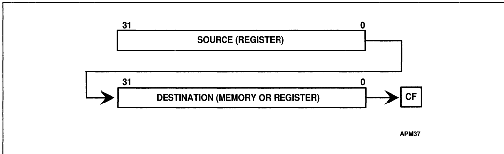
Figure 4-10. SHRD Instruction
