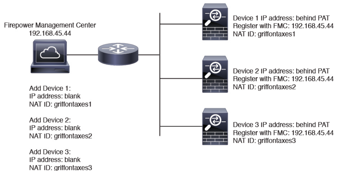
Figure 46: NAT ID for Managed Devices Behind PAT
