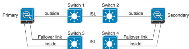
Figure 32: Connecting with a Secure Switch
