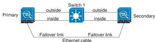
Figure 31: Connecting with a Cable
