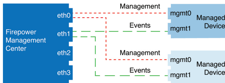
Figure 50: Separate Event Interface on the Firepower Management Center and Managed Devices
