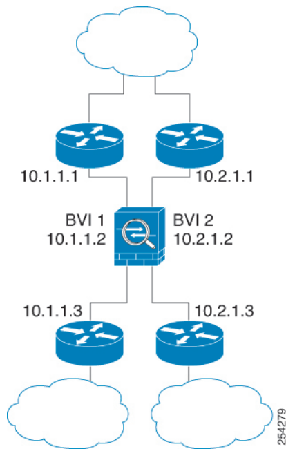
Figure 13: Transparent Firewall Network with Two Bridge Groups
