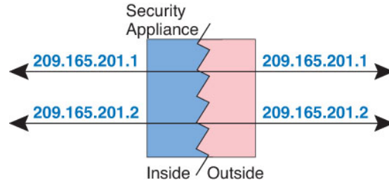
Figure 64: Identity NAT
