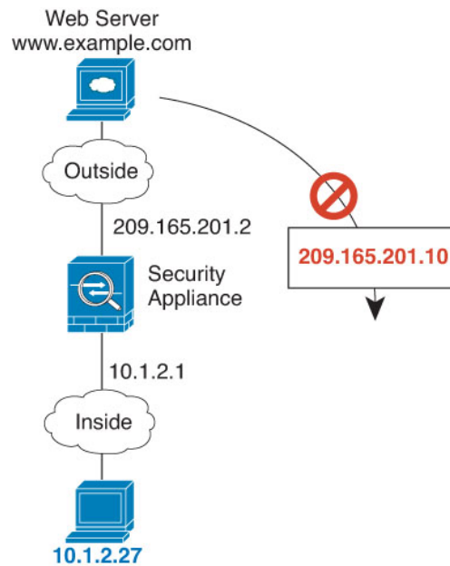
Figure 56: Remote Host Attempts to Initiate a Connection to a Mapped Address
