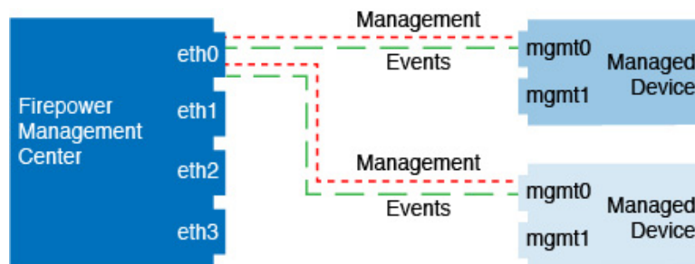
Figure 48: Single Management Interface on the Firepower Management Center
