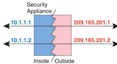
Figure 58: Static NAT
