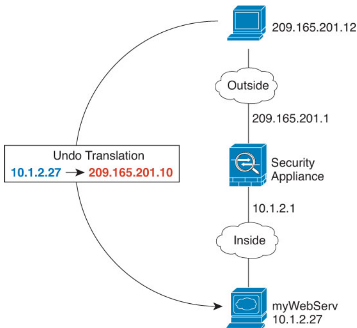
Figure 65: Static NAT for an Inside Web Server
