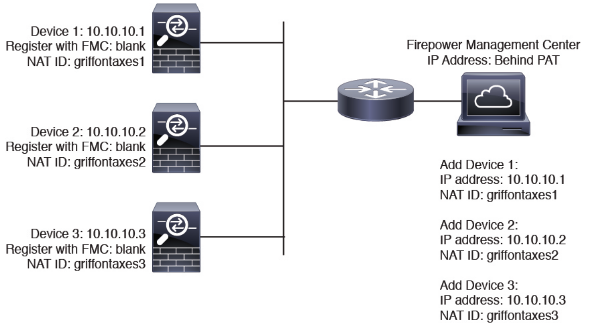
Figure 47: NAT ID for FMC Behind PAT
