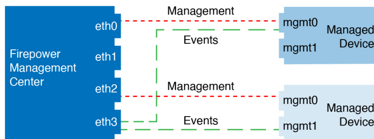
Figure 51: Mixed Management and Event Interface Usage
