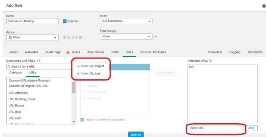
Figure 72: Manual URL Filtering Options in an Access Control Rule
