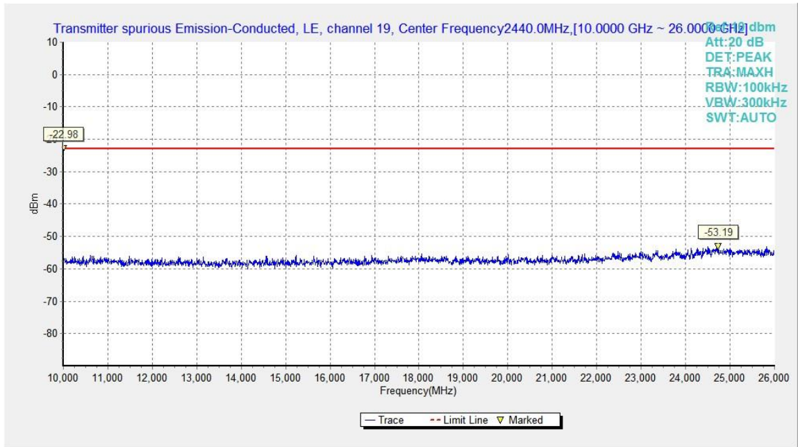
Fig.22. Transmitter Spurious Emission - Conducted: GFSK, 2440 MHz, 10GHz – 26GHz
