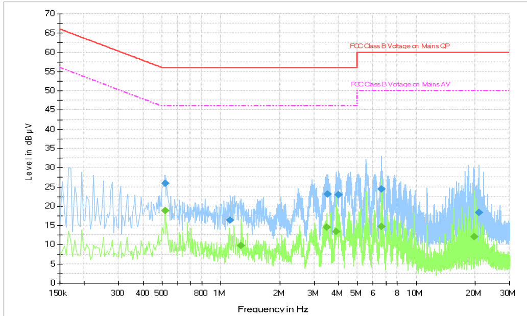
Fig.B.9.4 AC Powerline Conducted Emission-Idle
