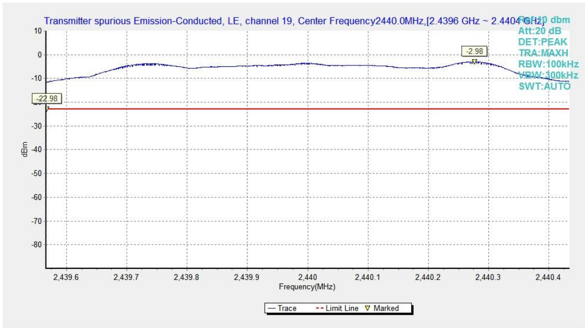
Fig.18. Transmitter Spurious Emission - Conducted: GFSK, 2440MHz
