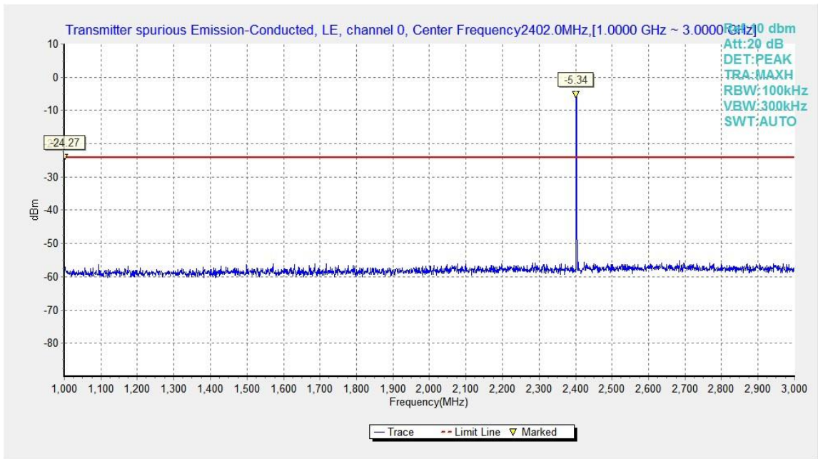
Fig.15. Transmitter Spurious Emission - Conducted: GFSK, 2402 MHz, 1GHz - 3GHz
