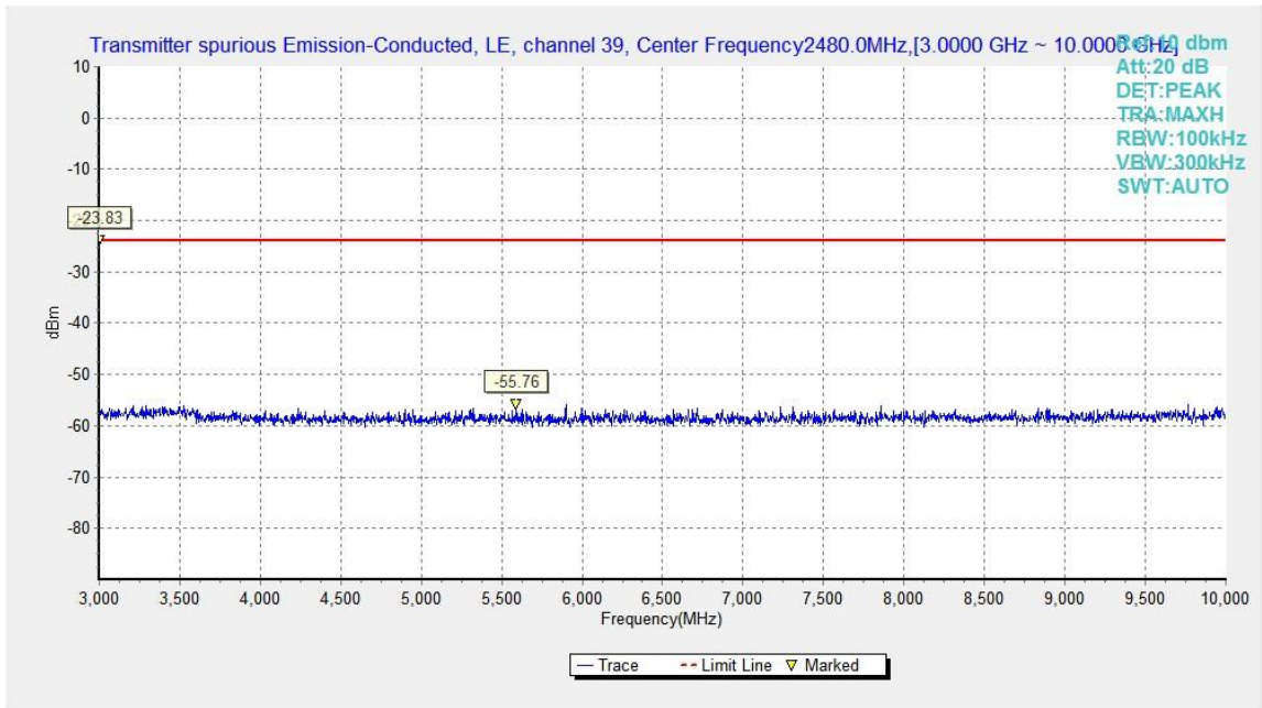
Fig.26. Transmitter Spurious Emission - Conducted: GFSK, 2480 MHz, 3GHz - 10GHz
