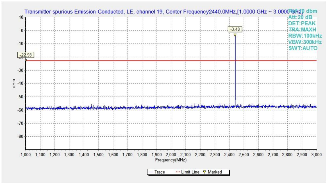
Fig.20. Transmitter Spurious Emission - Conducted: GFSK, 2440 MHz, 1GHz – 3GHz
