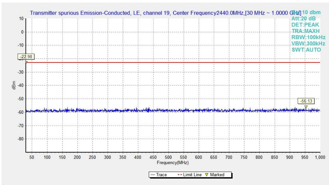
Fig.19. Transmitter Spurious Emission - Conducted: GFSK, 2440 MHz, 30MHz - 1GHz
