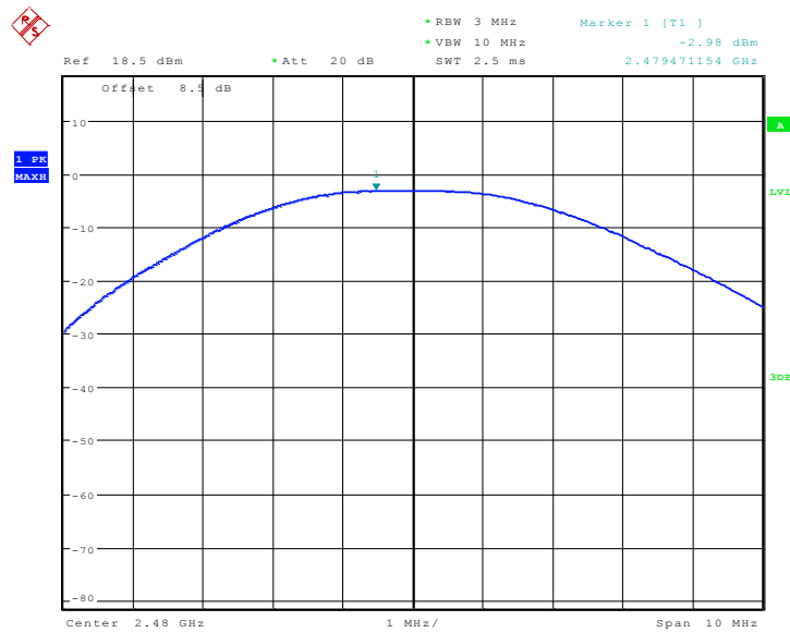
Fig.5. Peak Conducted Output Power: BLE, 2Mbps, Channel 19,
