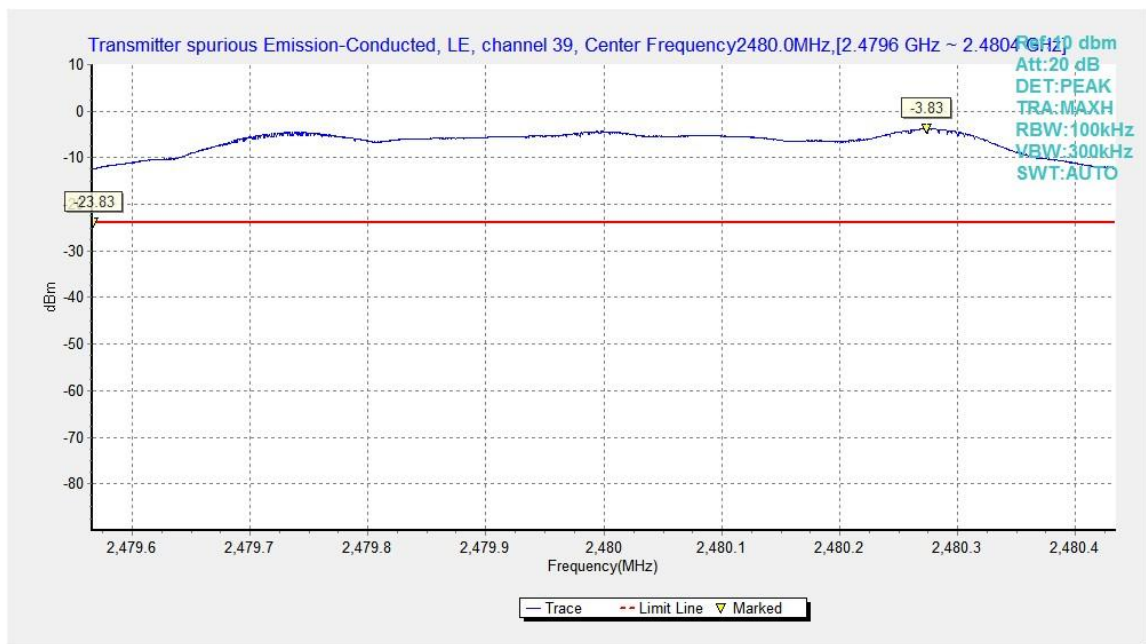
Fig.23. Transmitter Spurious Emission - Conducted: GFSK, 2480 MHz
