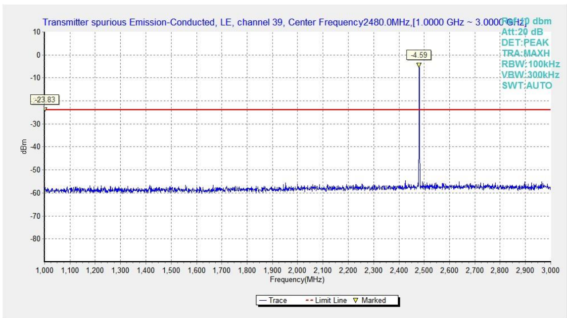
Fig.25. Transmitter Spurious Emission - Conducted: GFSK, 2480 MHz, 1GHz - 3GHz
