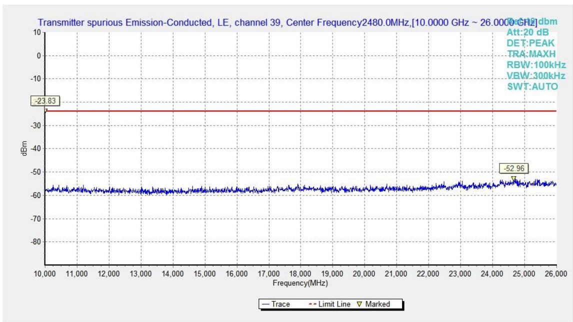
Fig.27. Transmitter Spurious Emission - Conducted: GFSK, 2480 MHz, 10GHz - 26GHz
