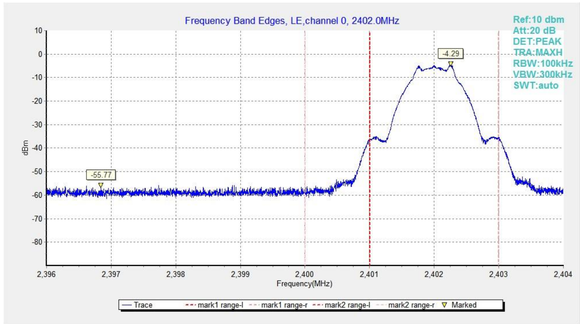
Fig.7. Frequency Band Edges: GFSK, 2402 MHz, Hopping Off
