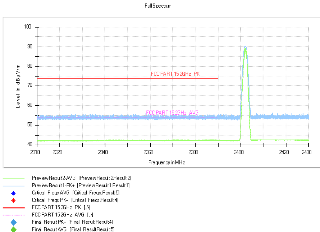
Fig.9. Frequency Band Edges: BLE 1Mbps, GFSK, 2402 MHz, Hopping Off, 2.38 GHz – 2.45GHz
