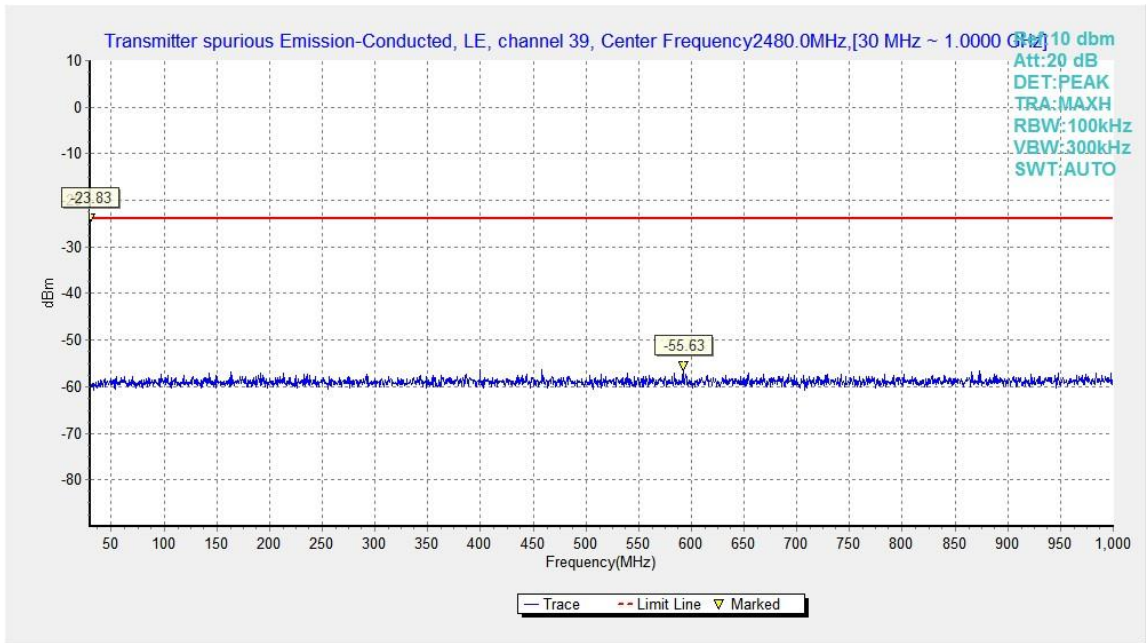
Fig.24. Transmitter Spurious Emission - Conducted: GFSK, 2480 MHz, 30MHz - 1GHz
