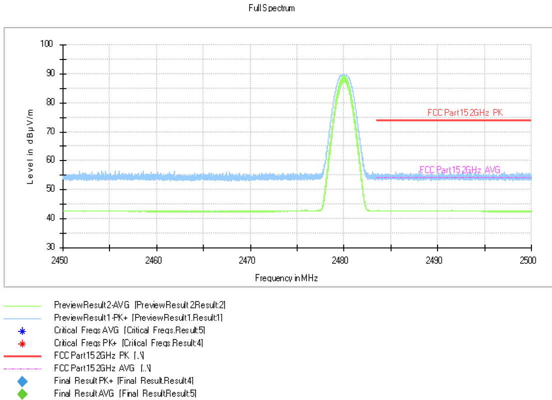
Fig.10. Frequency Band Edges: BLE 1Mbps GFSK, 2480 MHz, Hopping Off , 2.45 GHz - 2.50GHz
