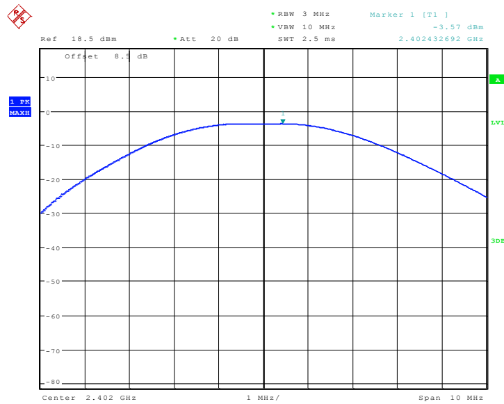
Fig.3. Peak Conducted Output Power: BLE, 1Mbps, Channel 39,
