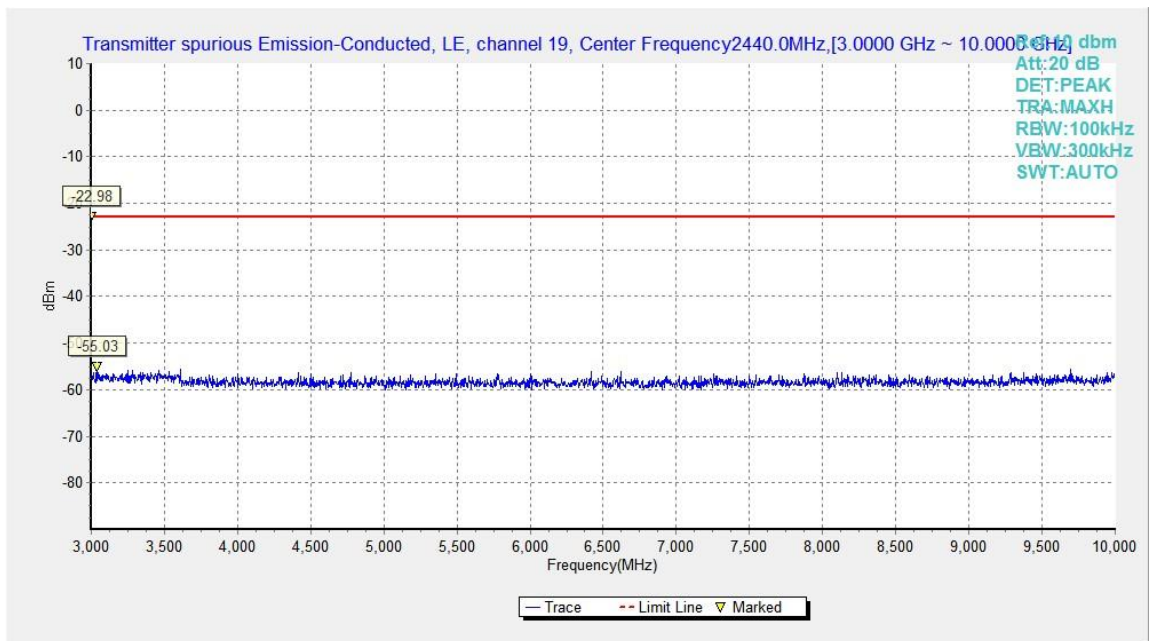
Fig.21. Transmitter Spurious Emission - Conducted: GFSK, 2440 MHz, 3GHz – 10GHz
