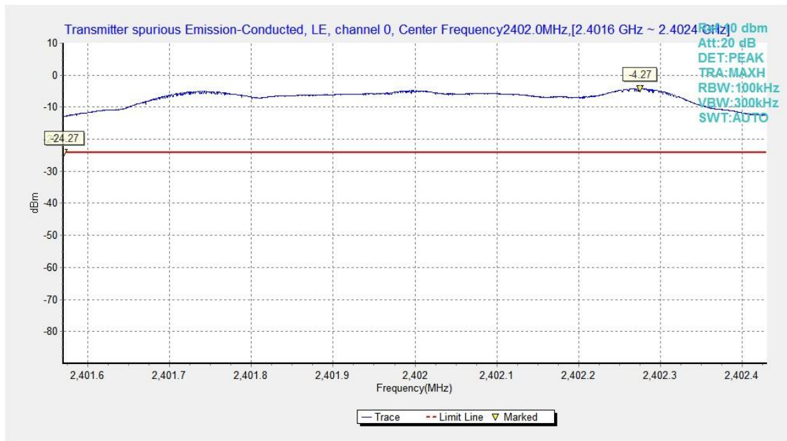
Fig.13. Transmitter Spurious Emission - Conducted: GFSK,2402MHz
