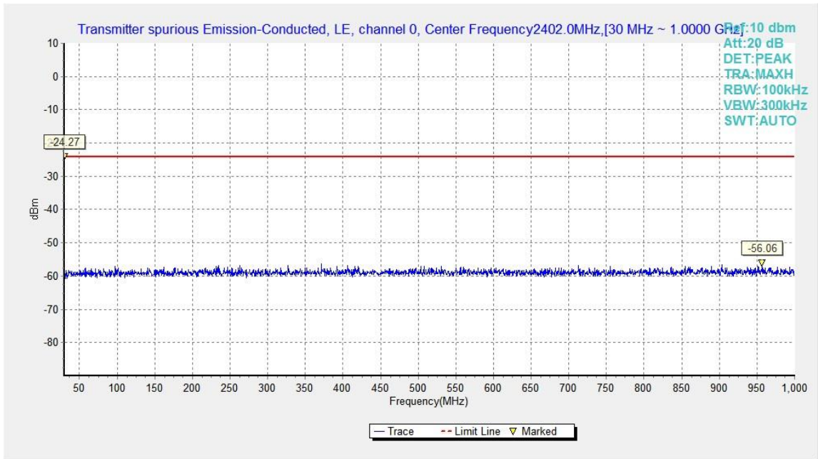
Fig.14. Transmitter Spurious Emission - Conducted: GFSK, 2402 MHz, 30MHz - 1GHz
