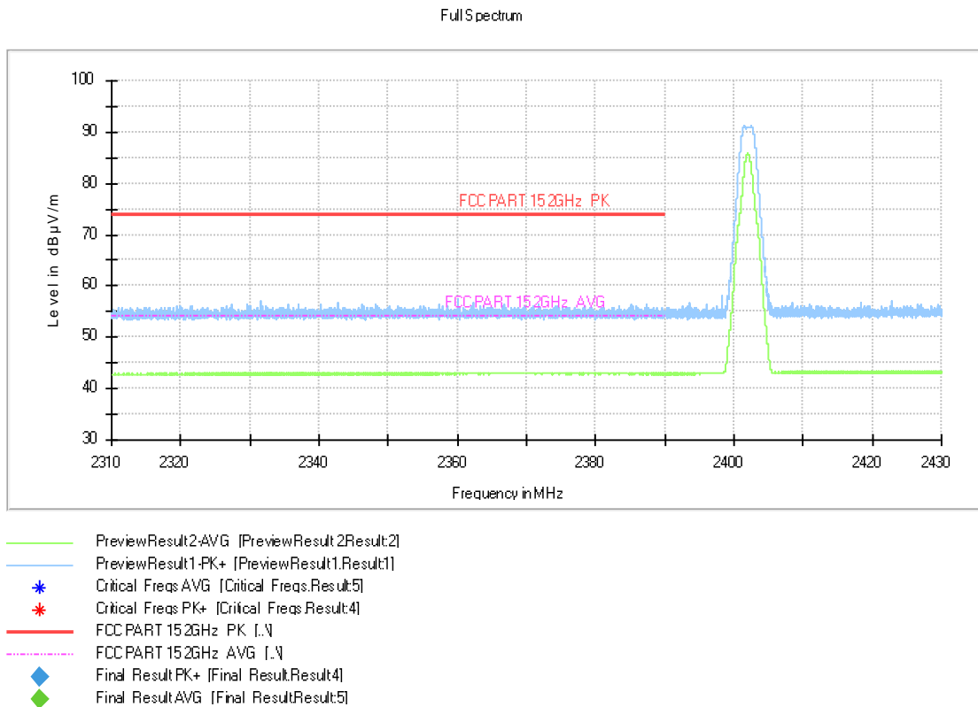
Fig.11. Frequency Band Edges: BLE 2Mbps, GFSK, 2402 MHz, Hopping Off, 2.38 GHz - 2.45GHz
