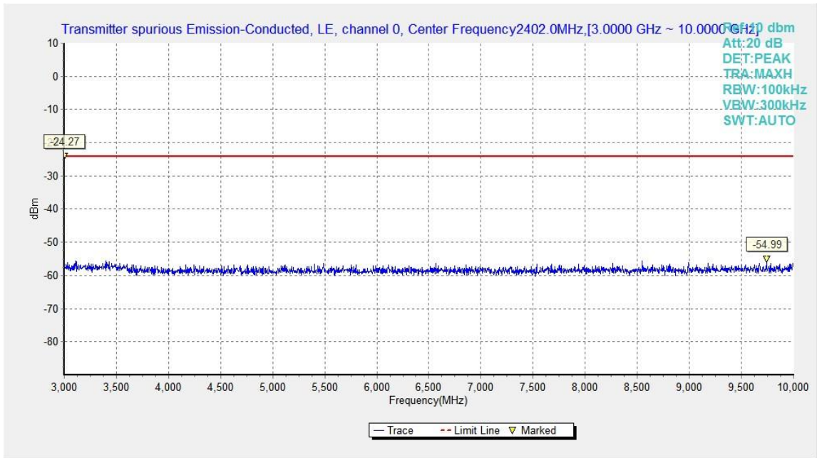
Fig.16. Transmitter Spurious Emission - Conducted: GFSK, 2402 MHz,3GHz - 10GHz
