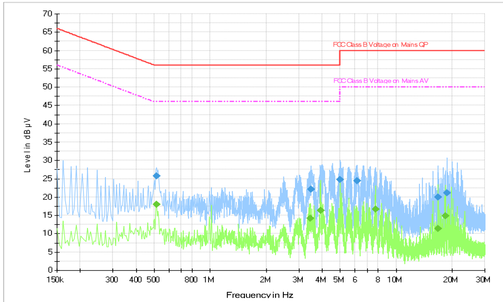
Fig.B.9.3 AC Powerline Conducted Emission- Bluetooth BLE 2Mbps
