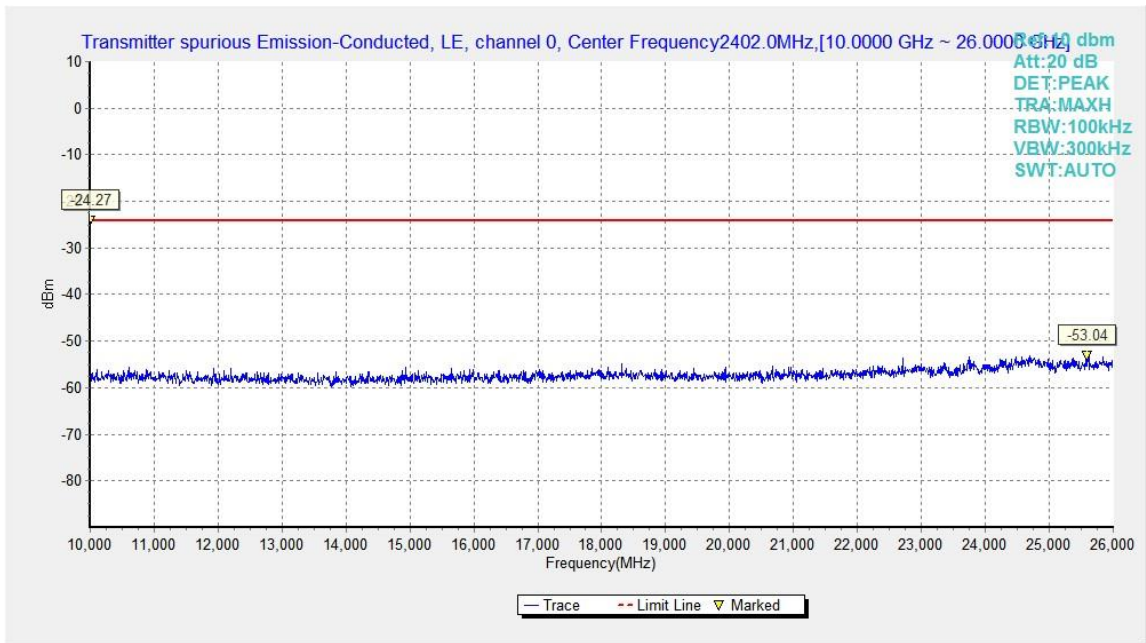
Fig.17. Transmitter Spurious Emission - Conducted: GFSK, 2402 MHz,10GHz - 26GHz
