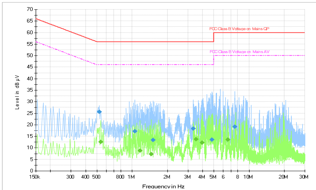
Fig.B.9.1 AC Powerline Conducted Emission- Bluetooth BLE 1Mbps
