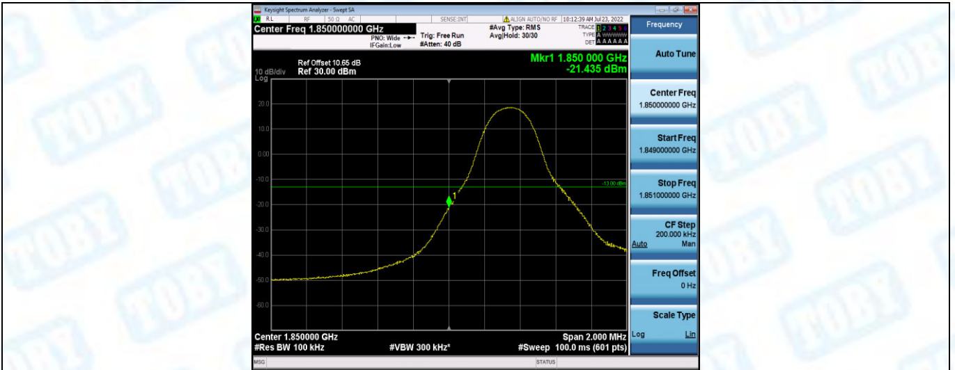
Band25-5MHz-16QAM-26065-1RB#24
