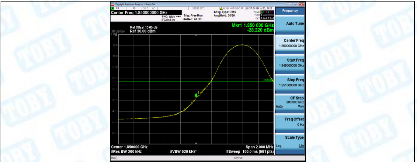
Band25-10MHz-16QAM-26090-1RB#49
