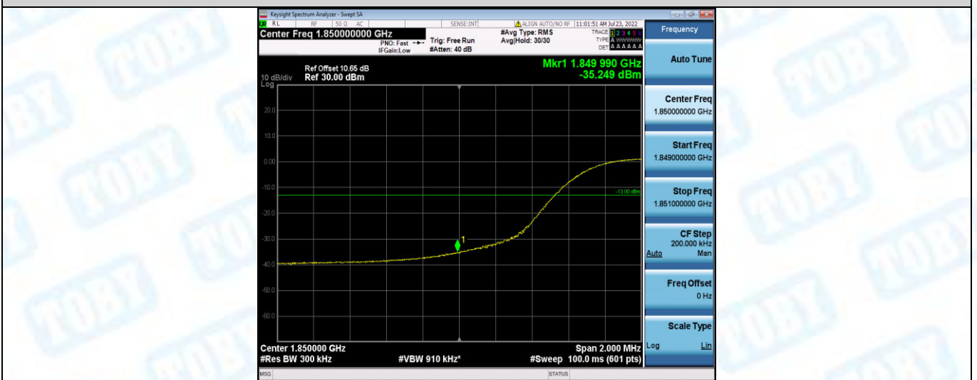
Band25-15MHz-16QAM-26615-1RB#0
