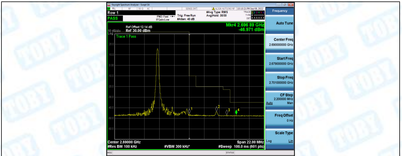
Band41-5MHz-QPSK-41565-1RB#24
