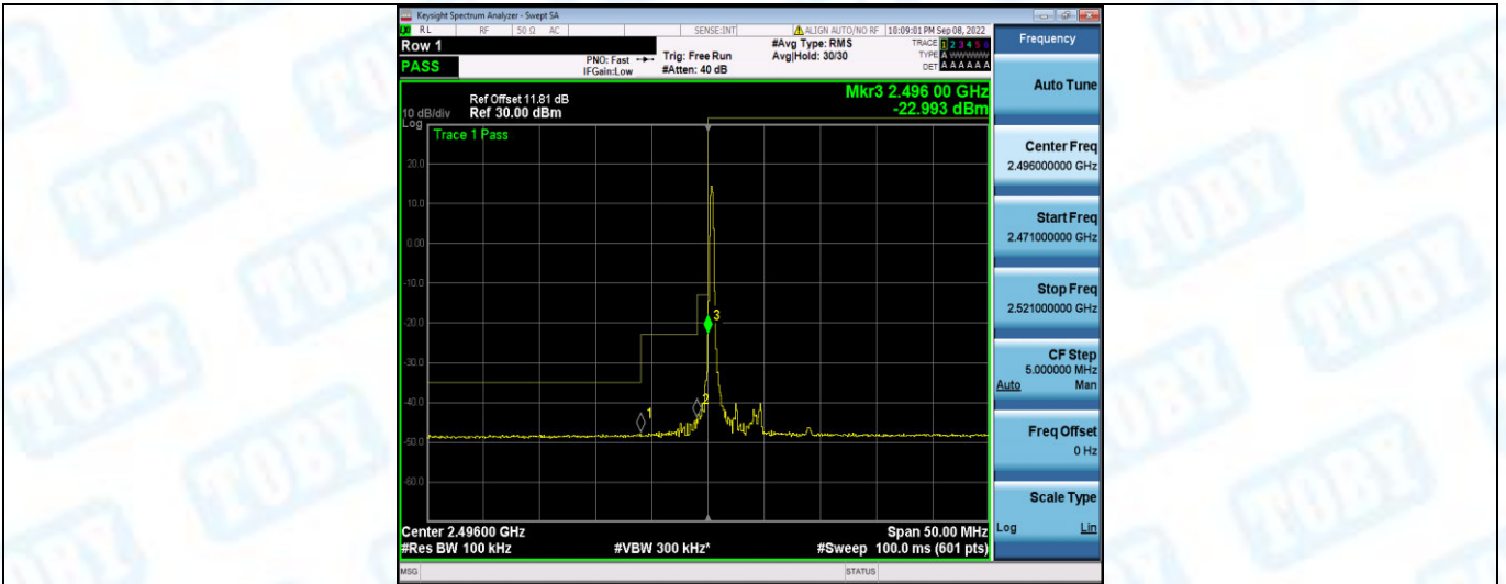
Band41-5MHz-QPSK-39675-1RB#24
