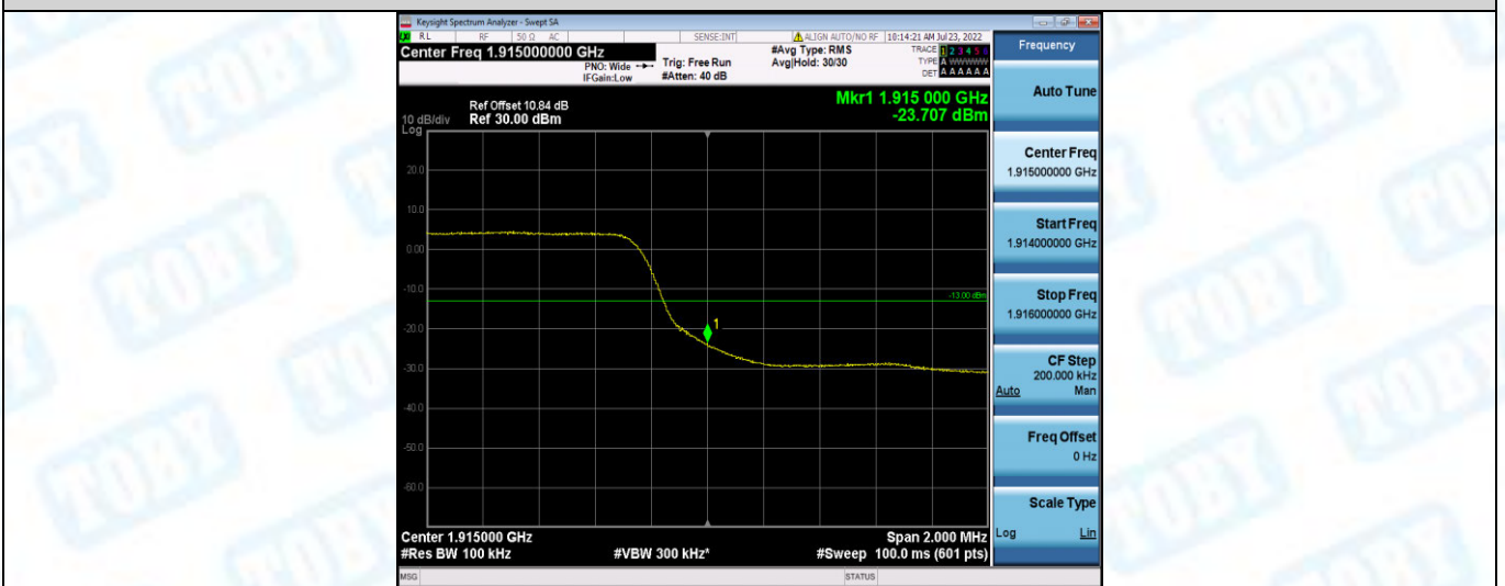
Band25-5MHz-16QAM-26065-1RB#0
