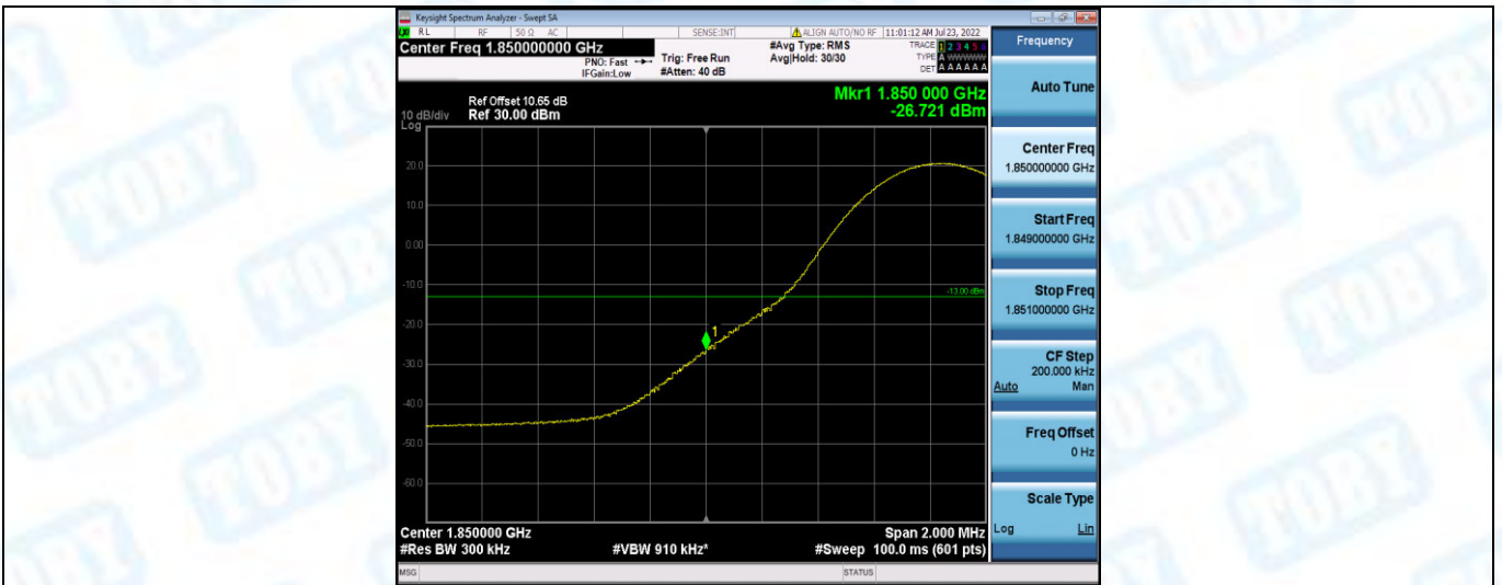
Band25-15MHz-16QAM-26115-1RB#74
