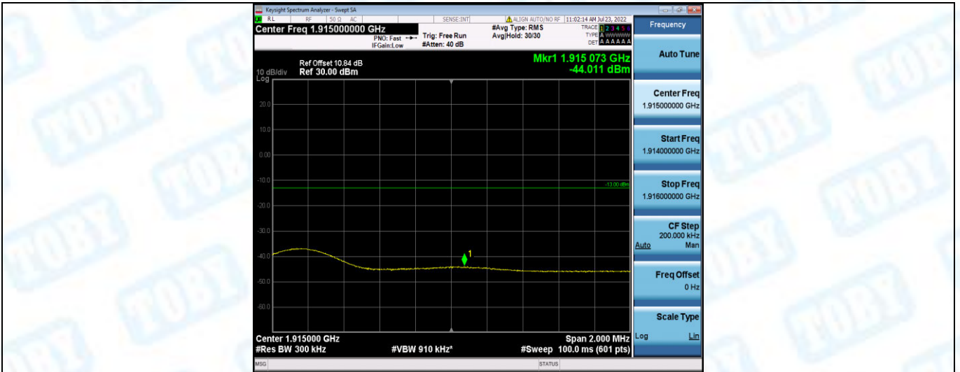
Band25-15MHz-QPSK-26615-1RB#74
