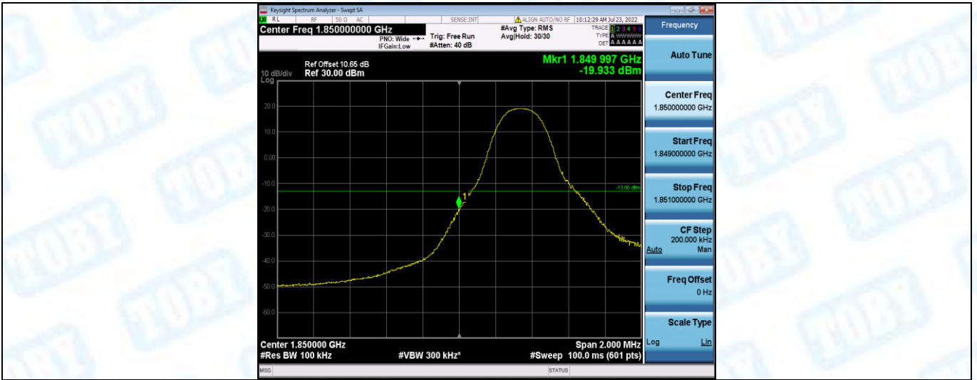
Band25-5MHz-QPSK-26065-1RB#24
