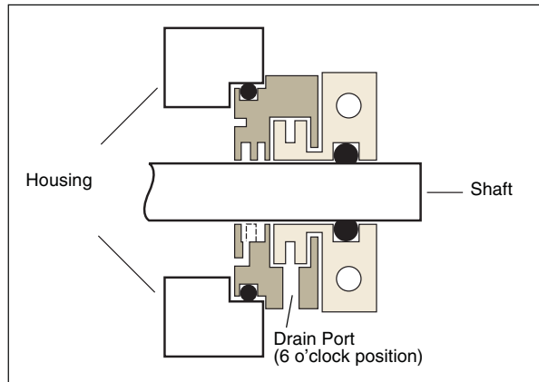
Figure 8-3. Proper Installation
