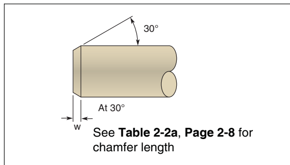
Figure 6-1. Shaft Profile
