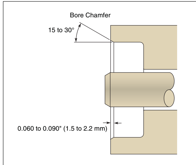
Figure 2-19. Housing Profile
