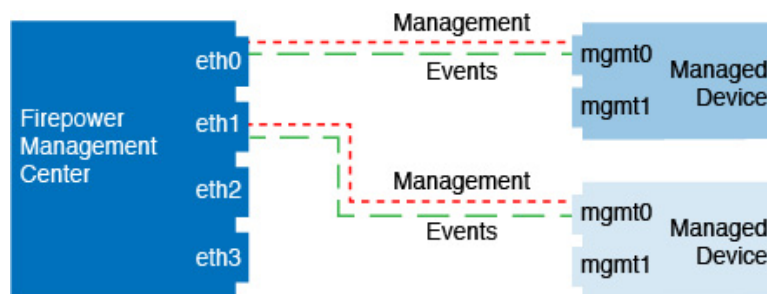
Figure 48: Multiple Management Interfaces on the Firepower Management Center
