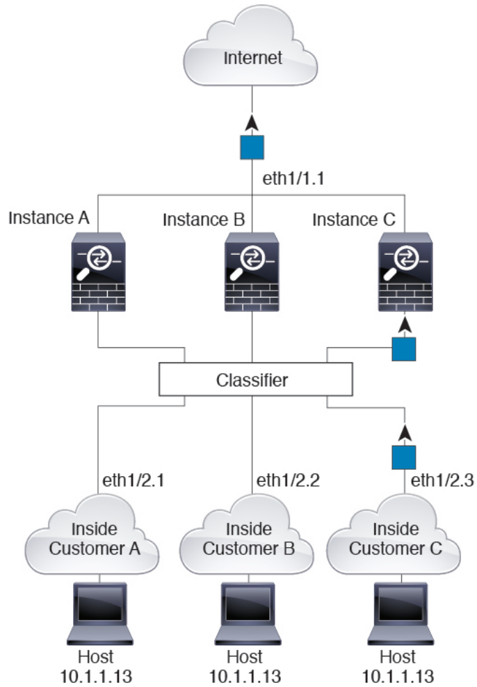
Figure 22: Incoming Traffic from Inside Networks
