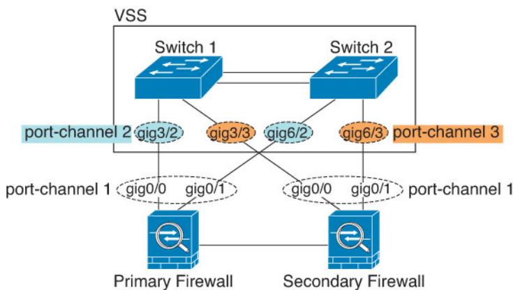
Figure 27: Active/Standby Failover and VSS/vPC
