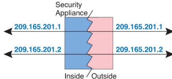
Figure 63: Identity NAT
