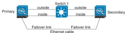
Figure 31: Connecting with a Cable
