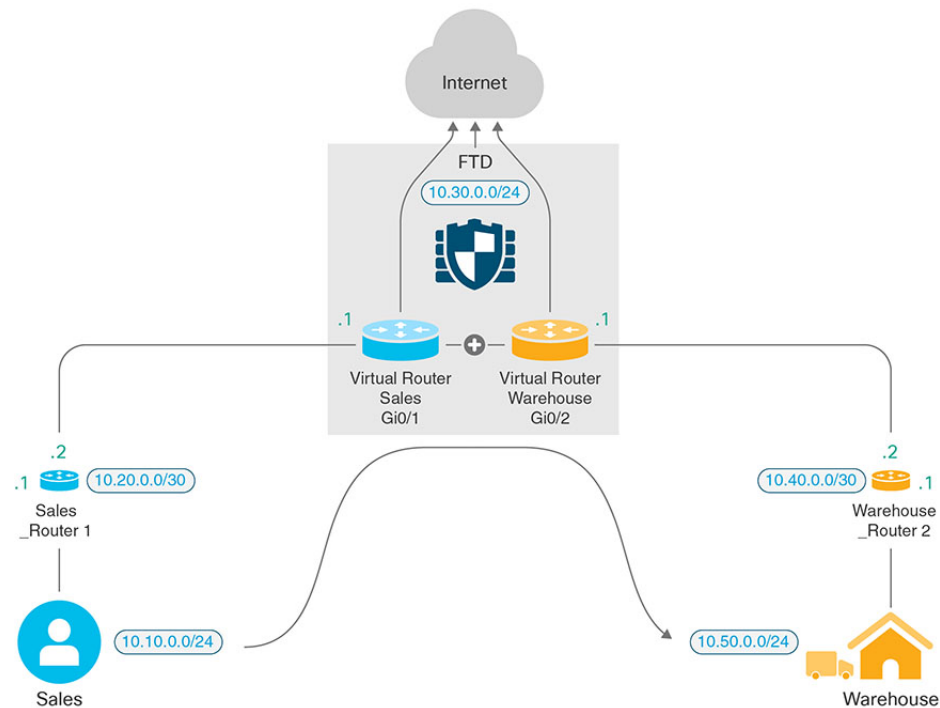
Figure 41: Interconnecting Two Virtual Routers - An Example
