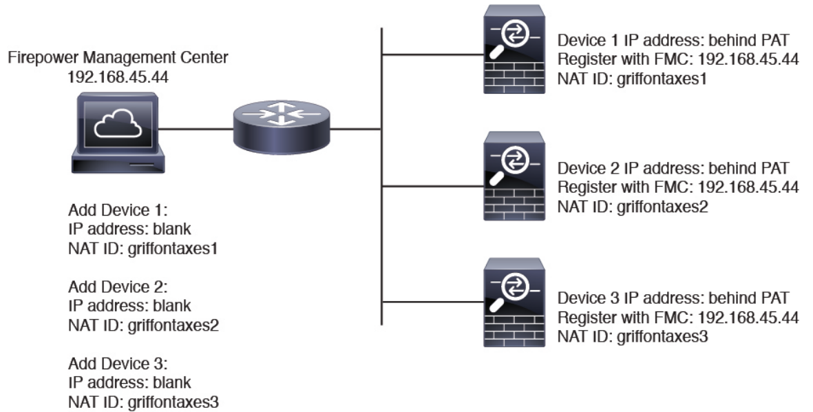
Figure 45: NAT ID for Managed Devices Behind PAT
