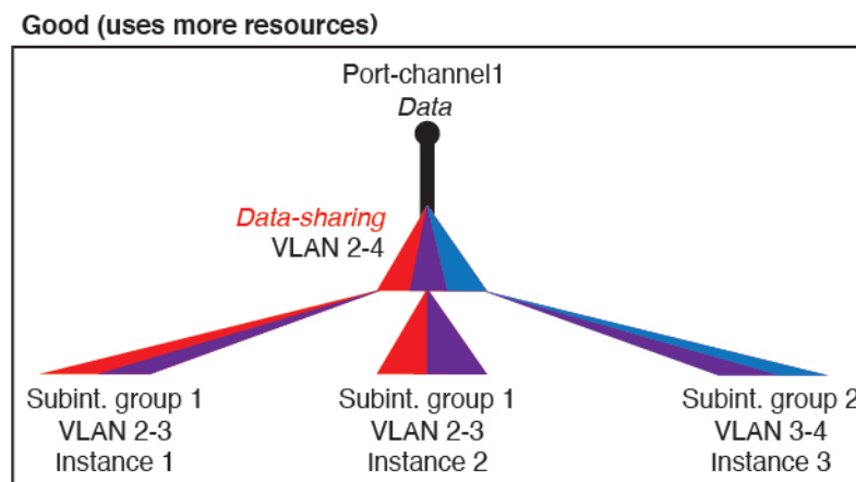
Figure 18: Good: Sharing Multiple Subinterface Groups on One Parent
