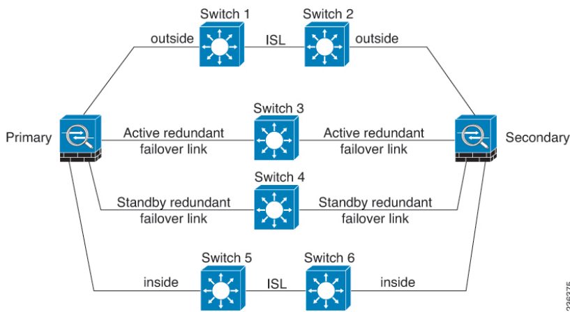
Figure 34: Connecting with Inter-switch Links
