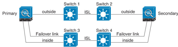
Figure 32: Connecting with a Secure Switch
