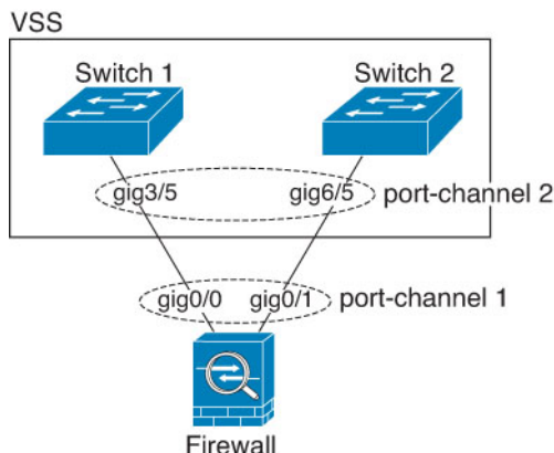
Figure 26: Connecting to a VSS/vPC
