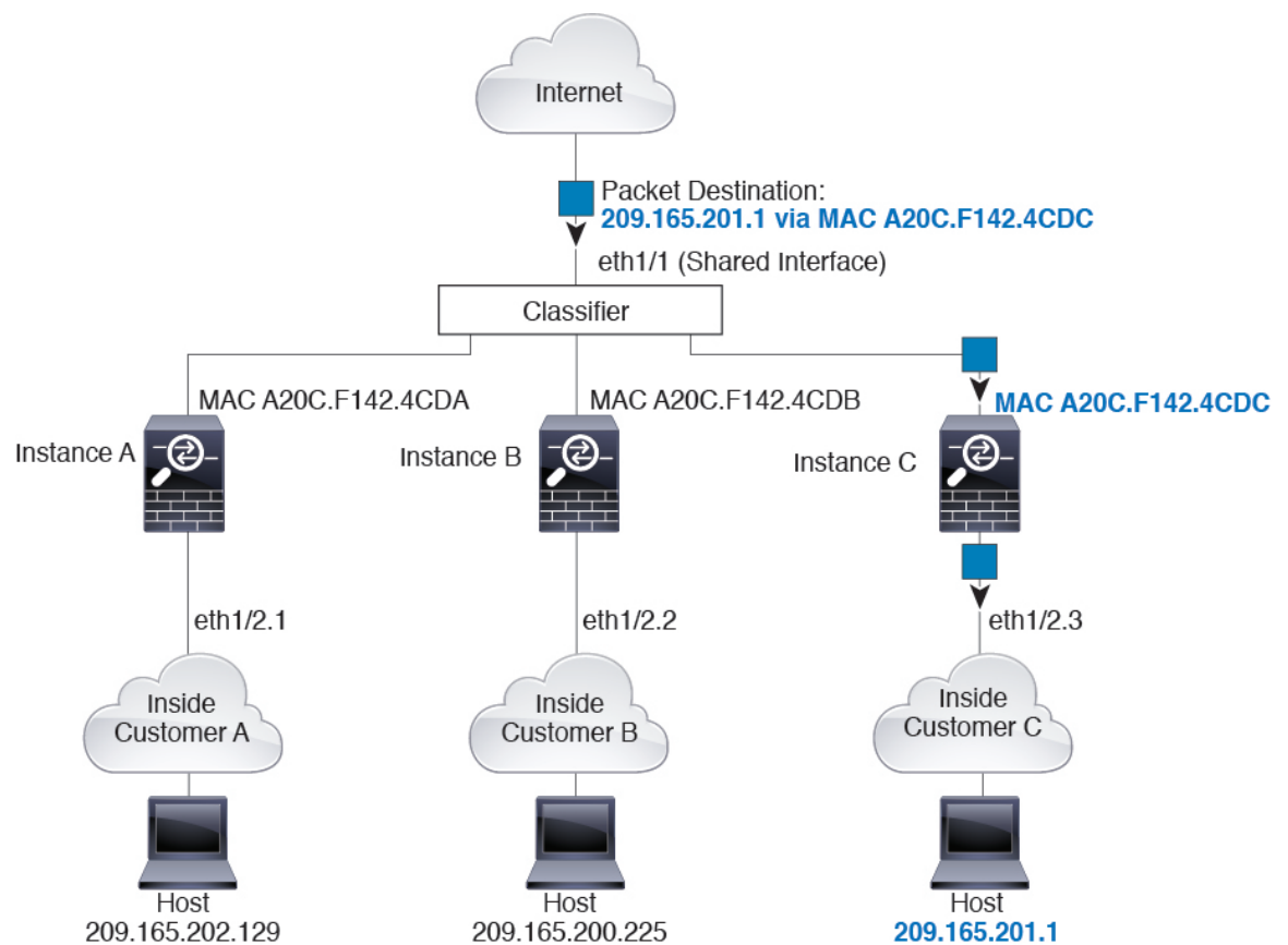
Figure 21: Packet Classification with a Shared Interface Using MAC Addresses
