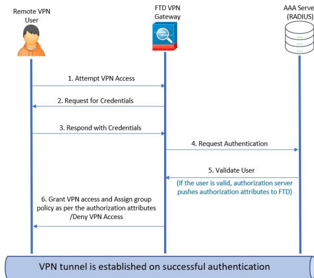
Figure 42: Remote Access VPN Group Policy Selection by AAA Server
