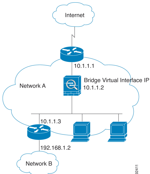
Figure 12: Transparent Firewall Network
