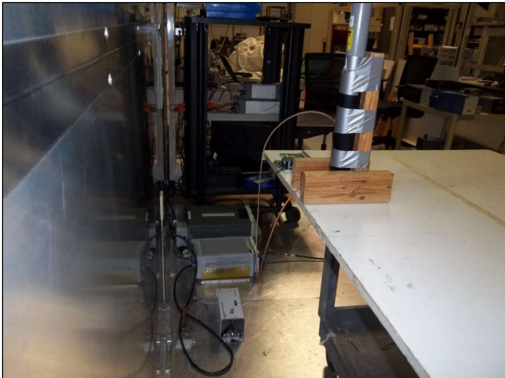
Figure 12: Conducted Emissions
