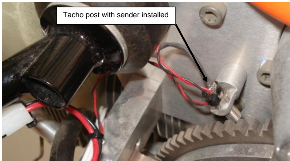
Figure 37 – Tacho Sender #1
