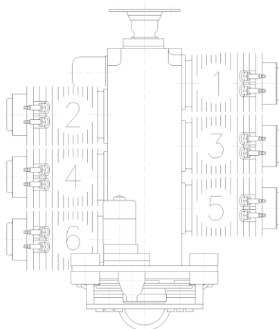
Figure 5 – 3300 Cylinder Denomination
