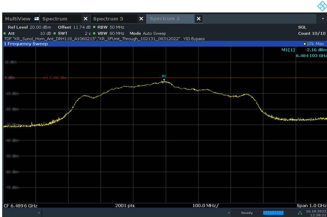
Plot 7-64. UWB Peak Power Measurement - ANT 2 - CH.5 – BPRF
