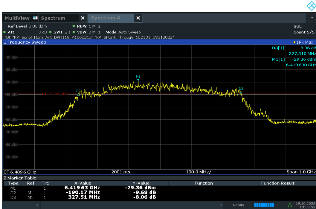
Plot 7-43. 10dBc Bandwidth – CH.5 - SP0 – Preamble 27
