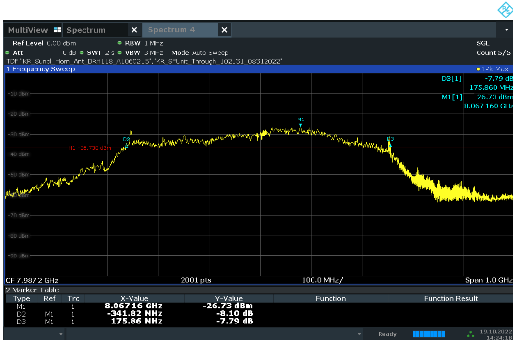
Plot 7-56. 10dBc Bandwidth – CH.9 – SP1 – Preamble 12
