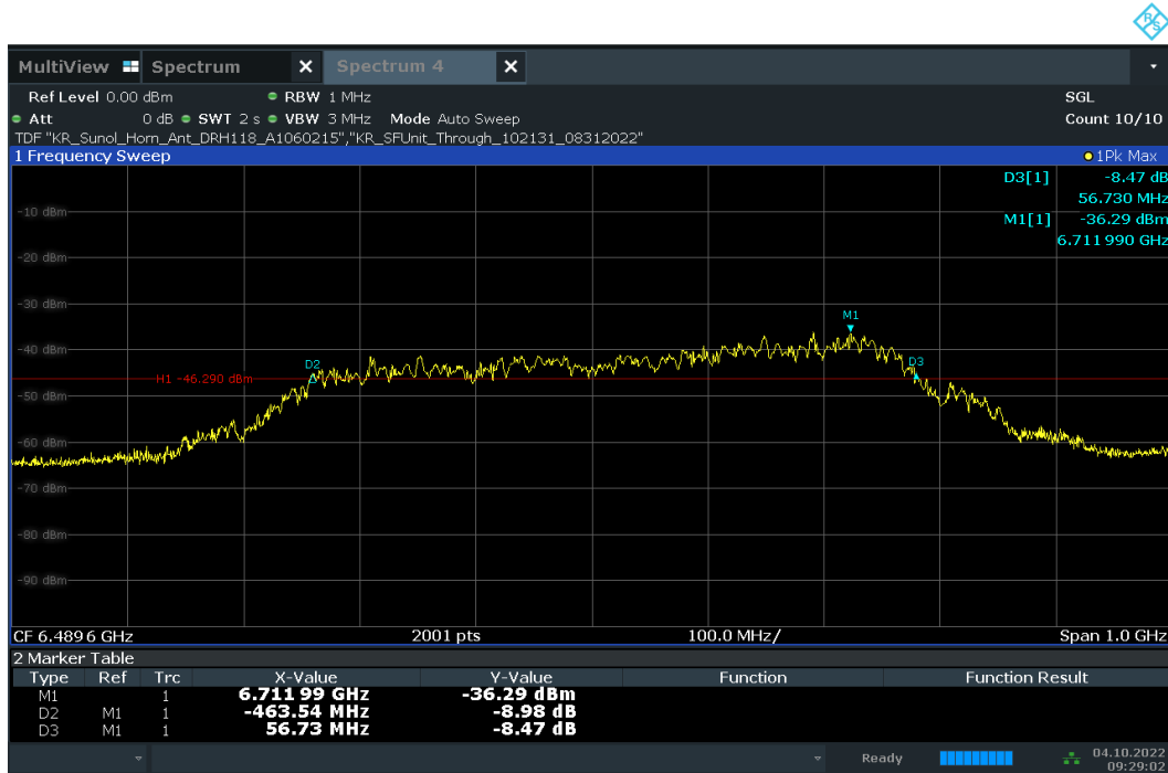
Plot 7-10. 10dBc Bandwidth – CH.5 - SP0 – Preamble 12
