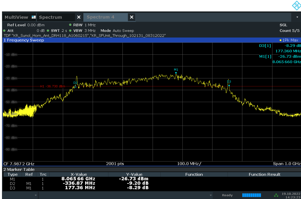
Plot 7-55. 10dBc Bandwidth – CH.9 - SP0 – Preamble 12
