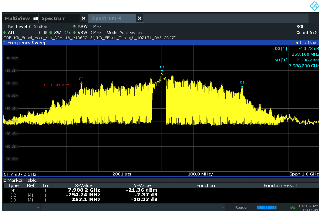
Plot 7-50. 10dBc Bandwidth – CH.9 – SP1 – Preamble 10
