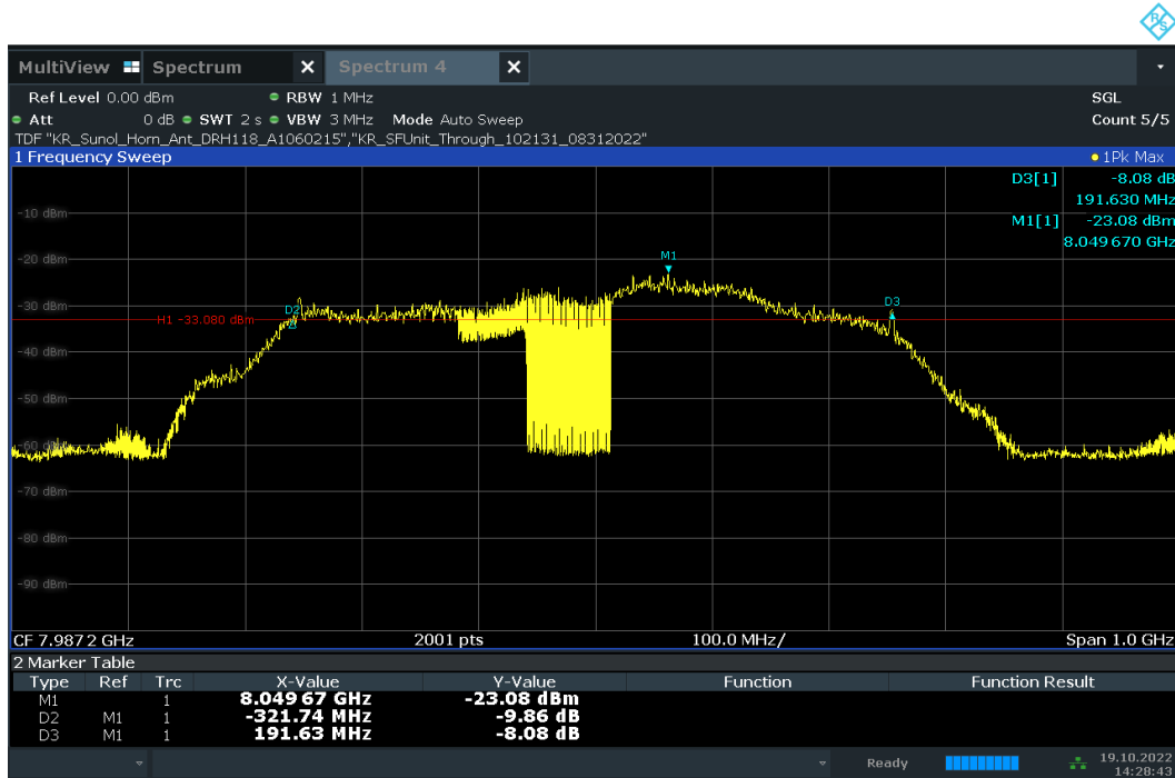
Plot 7-60. 10dBc Bandwidth – CH.9 – SP3 – Preamble 27
