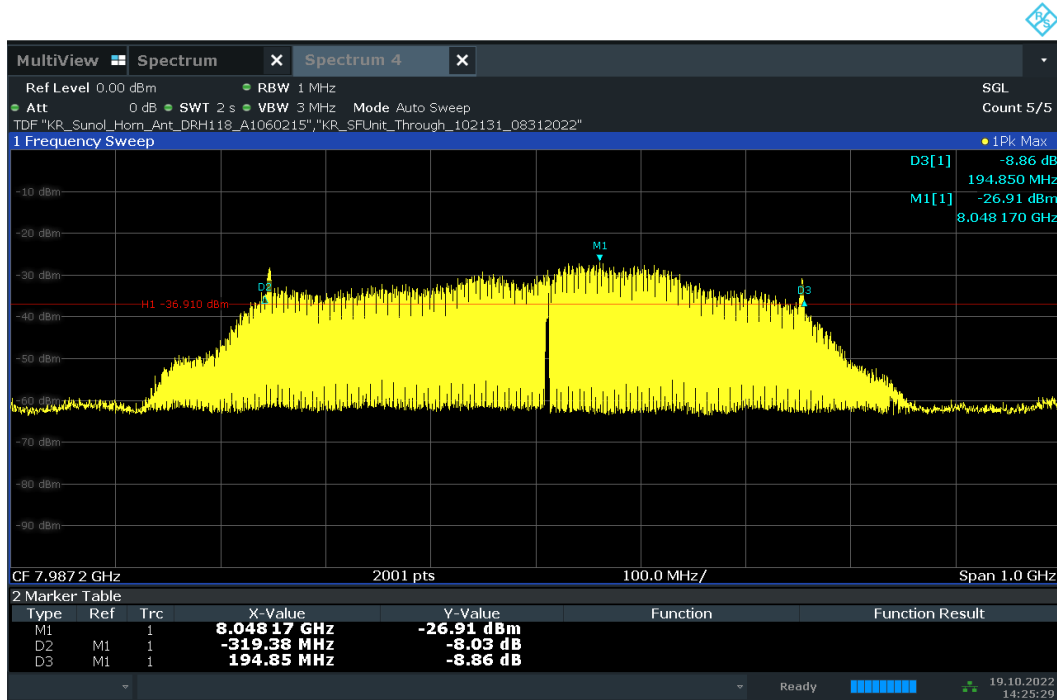
Plot 7-57. 10dBc Bandwidth – CH.9 – SP3 – Preamble 12
