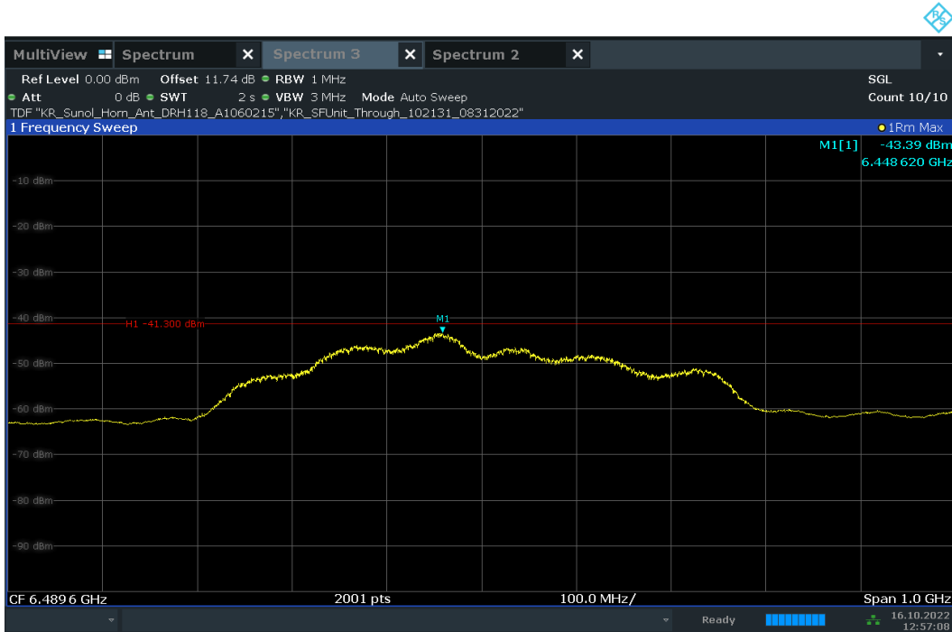
Plot 7-76. UWB Average Power Measurement - ANT 2 - CH.5 – HPRF
