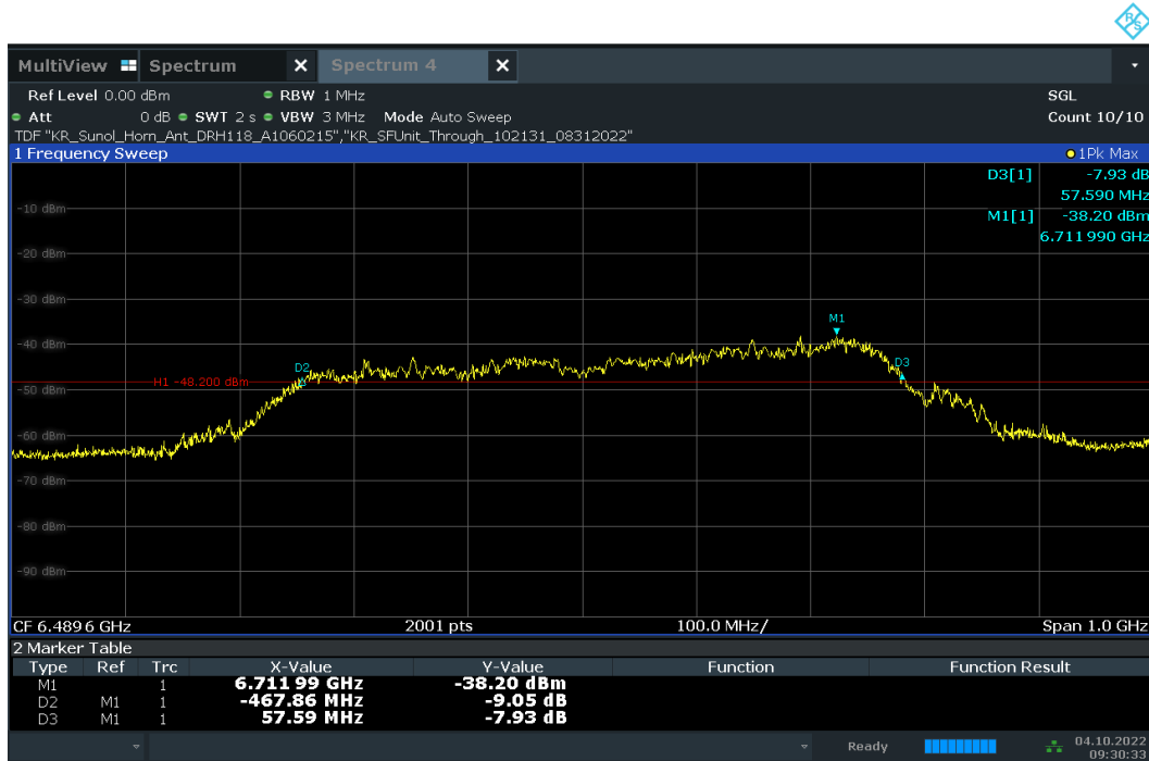
Plot 7-11. 10dBc Bandwidth – CH.5 – SP1 – Preamble 12
