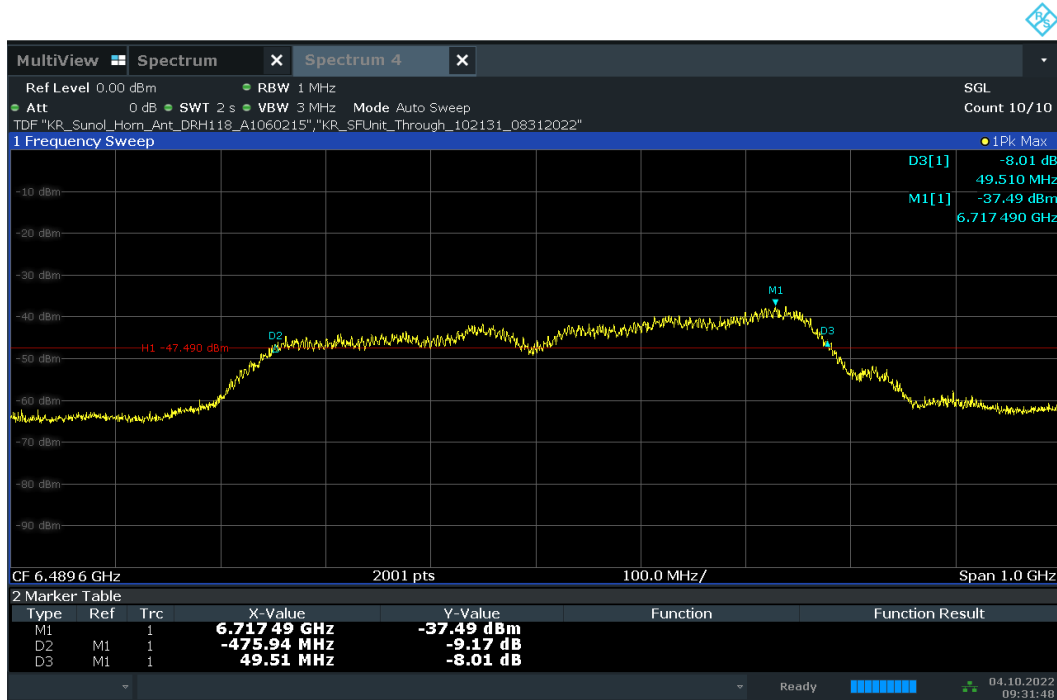
Plot 7-12. 10dBc Bandwidth – CH.5 – SP3 – Preamble 12
