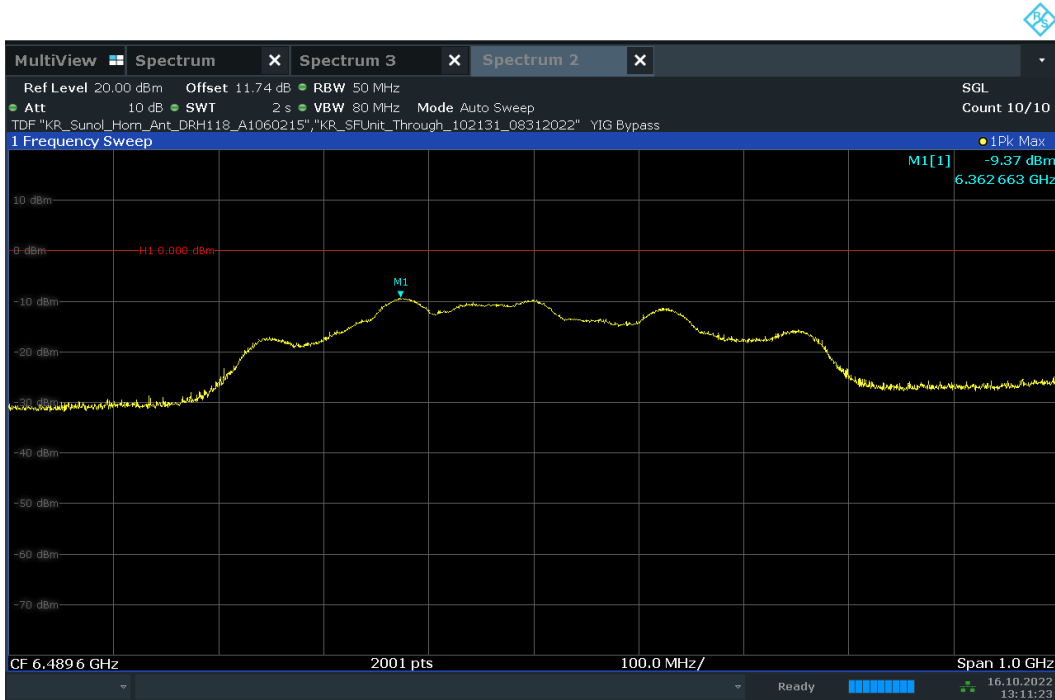
Plot 7-72. UWB Peak Power Measurement - ANT 2 - CH.5 – HPRF
