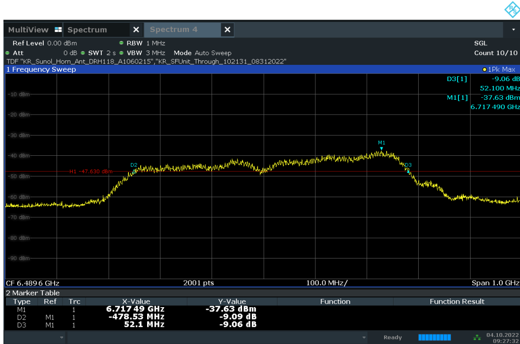
Plot 7-9. 10dBc Bandwidth – CH.5 – SP3 – Preamble 11
