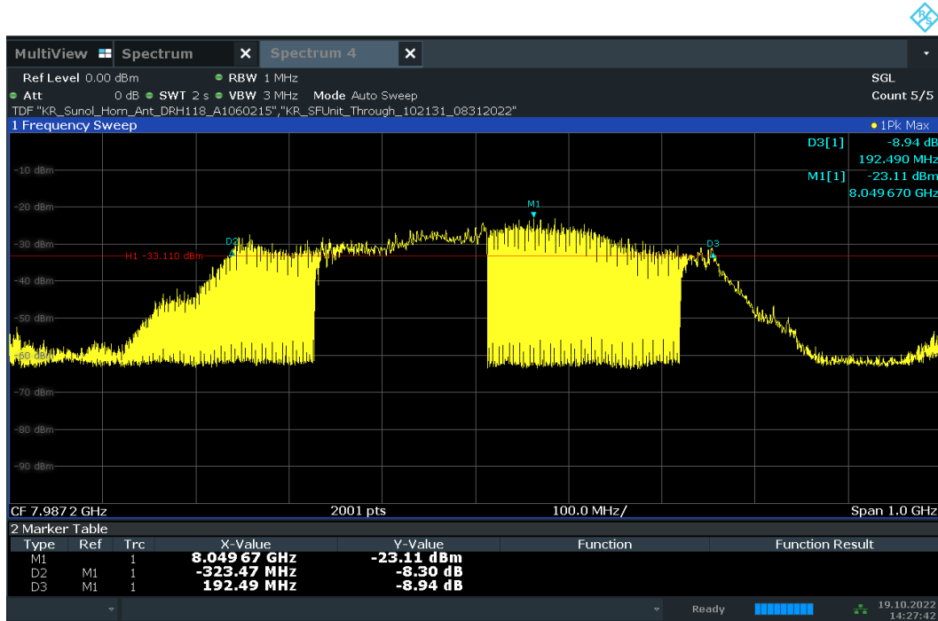
Plot 7-59. 10dBc Bandwidth – CH.9 – SP1 – Preamble 27
