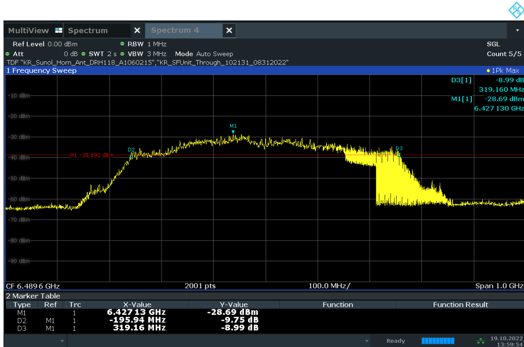
Plot 7-44. 10dBc Bandwidth – CH.5 – SP1 – Preamble 27
