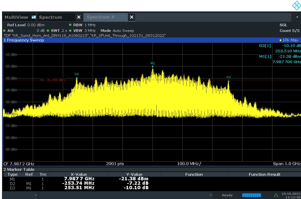
Plot 7-49. 10dBc Bandwidth – CH.9 - SP0 – Preamble 10
