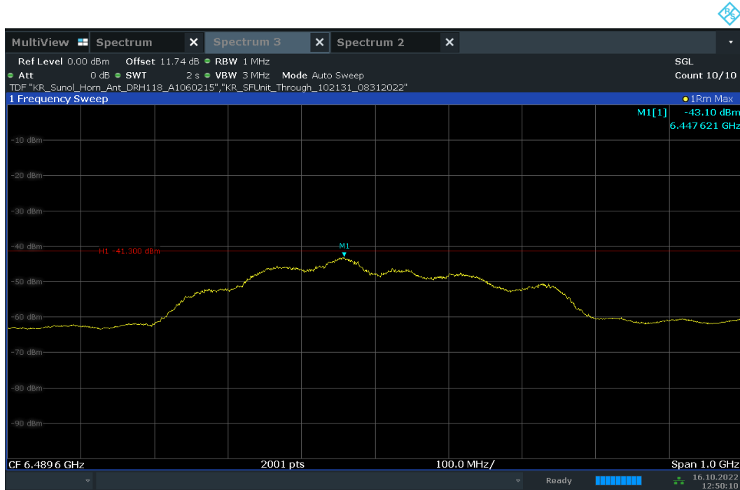
Plot 7-68. UWB Average Power Measurement - ANT 2 - CH.5 – BPRF
