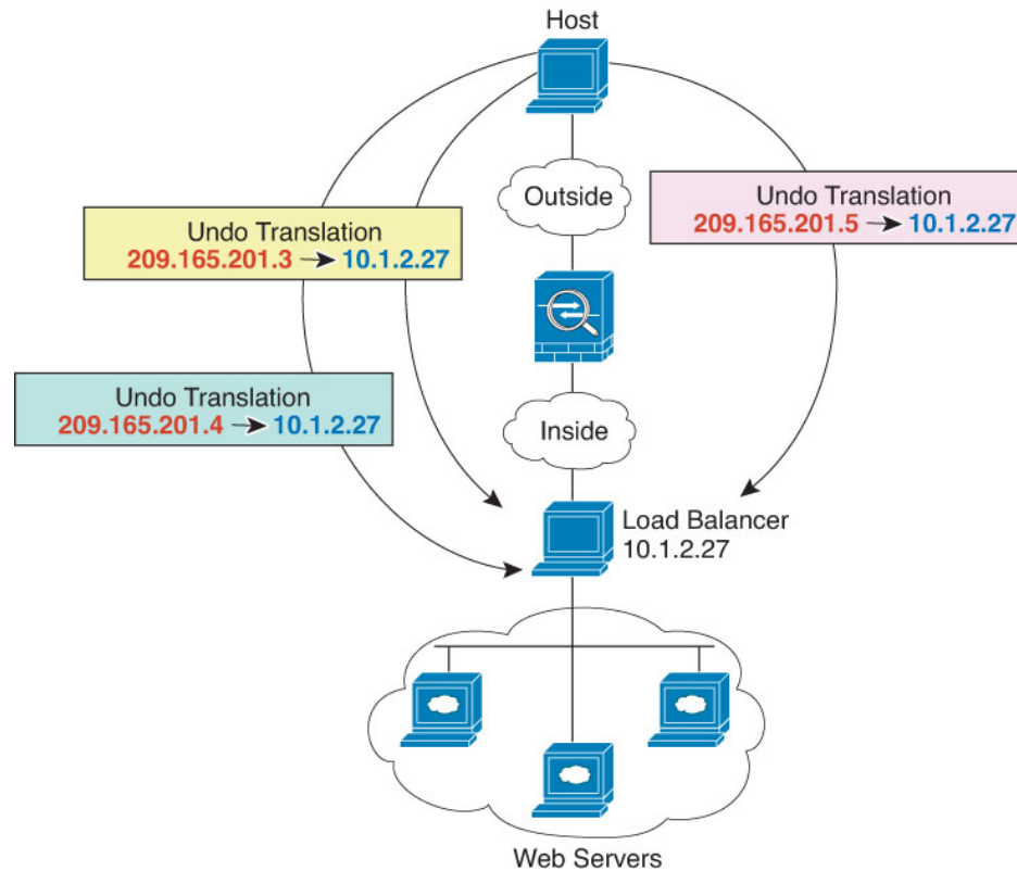
Figure 49: One-to-Many Static NAT Example
