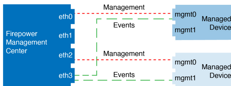
Figure 39: Mixed Management and Event Interface Usage
