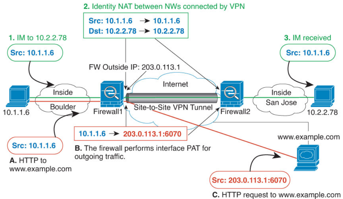
Figure 59: Interface PAT and Identity NAT for Site-to-Site VPN
