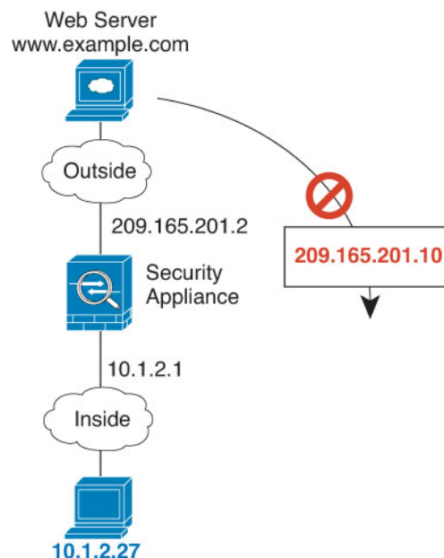
Figure 44: Remote Host Attempts to Initiate a Connection to a Mapped Address
