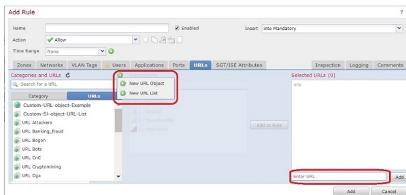
Figure 60: Manual URL Filtering Options in an Access Control Rule
