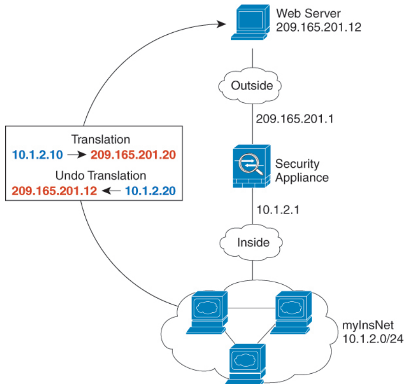
Figure 54: Dynamic NAT for Inside, Static NAT for Outside Web Server
