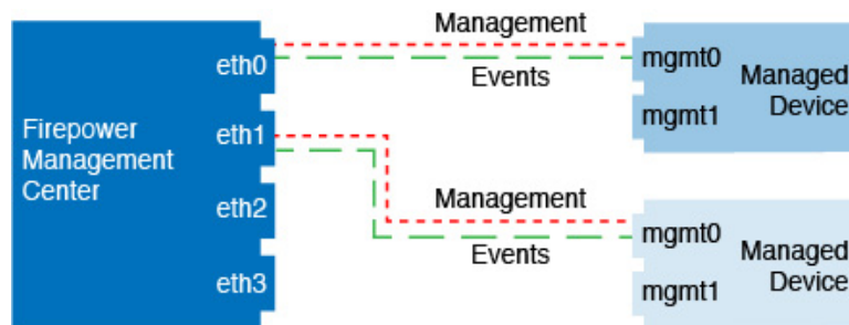
Figure 37: Multiple Management Interfaces on the Firepower Management Center
