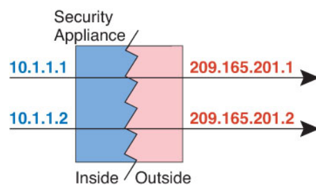
Figure 43: Dynamic NAT
