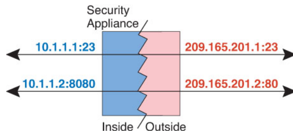
Figure 47: Typical Static NAT with Port Translation Scenario
