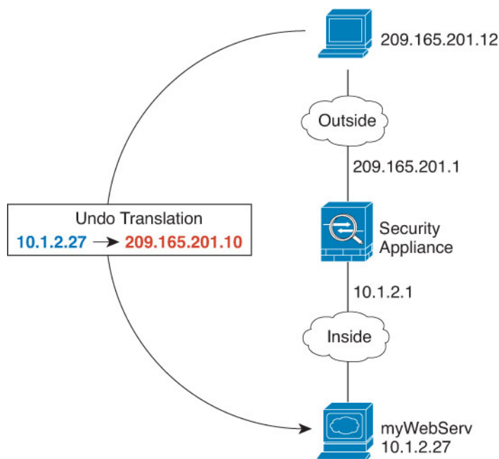
Figure 53: Static NAT for an Inside Web Server
