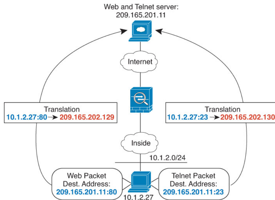
Figure 58: Manual NAT with Different Destination Ports
