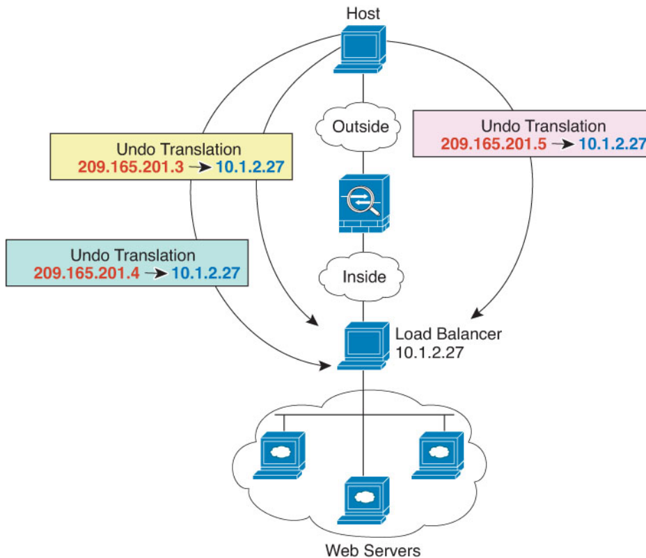
Figure 55: Static NAT with One-to-Many for an Inside Load Balancer
