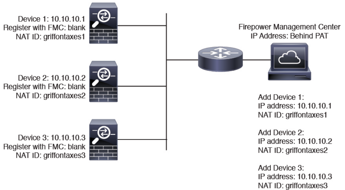
Figure 35: NAT ID for FMC Behind PAT
