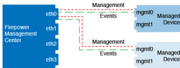
Figure 36: Single Management Interface on the Firepower Management Center
