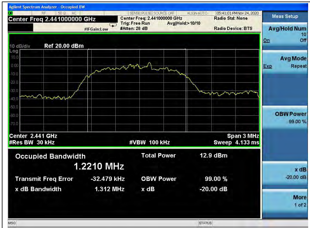
(Channel 39, 8-DPSK)
