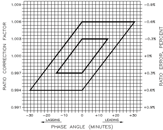
IEEE Std. C57.13 limits of accuracy class for current transformers for metering 0.3 accuracy class
