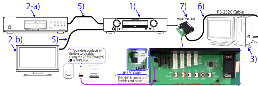
Figure 1 Device Connection Method (NR1510)
