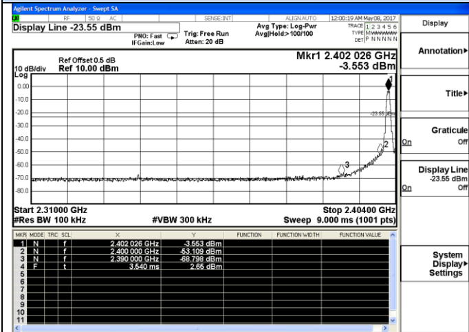
Channel 0 / 2402 MHz
