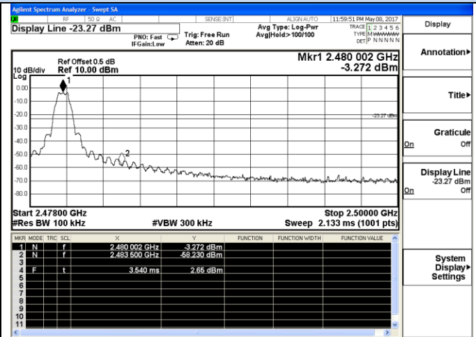
Channel 39 / 2480 MHz
