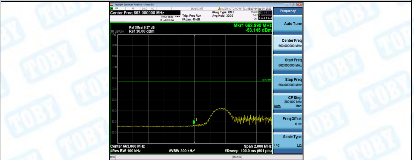
Band71-5MHz-16QAM-133147-25RB#0
