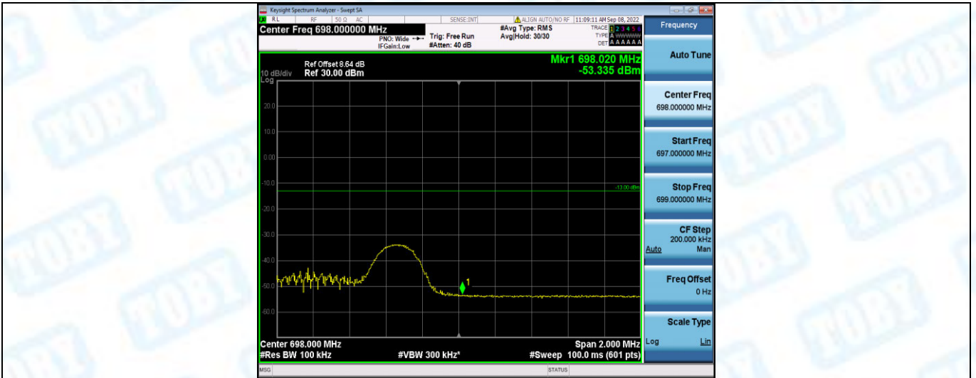
Band71-5MHz-16QAM-133447-1RB#24
