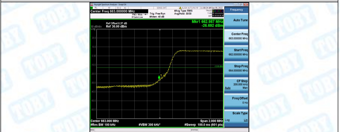
Band71-5MHz-16QAM-133447-1RB#0
