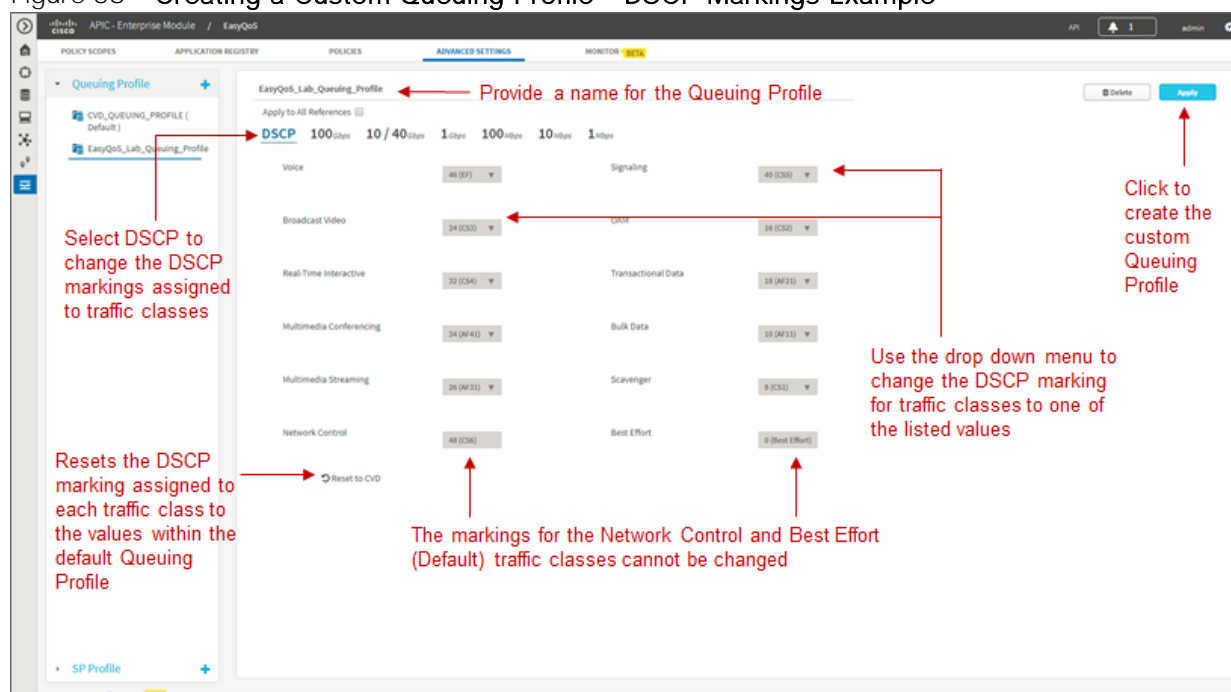
Figure 38 Creating a Custom Queuing Profile – DSCP Markings Example
