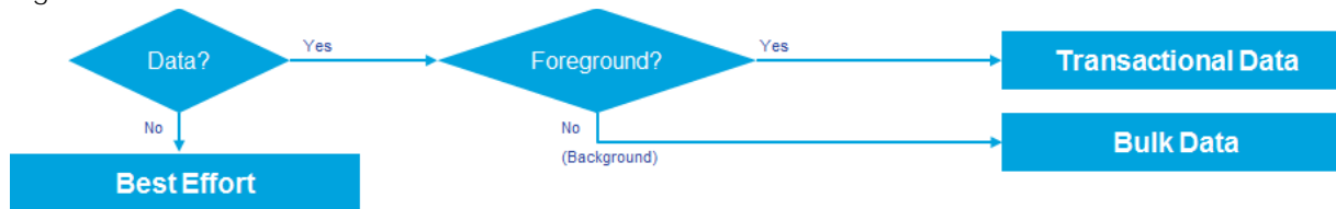
Figure 9 Data Traffic-classes
