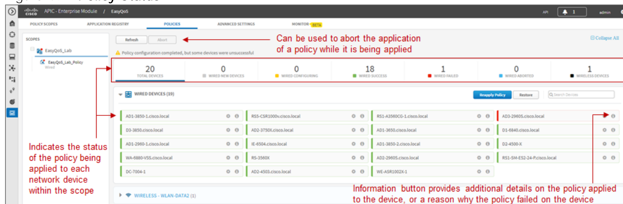
Figure 49 Policy Status
