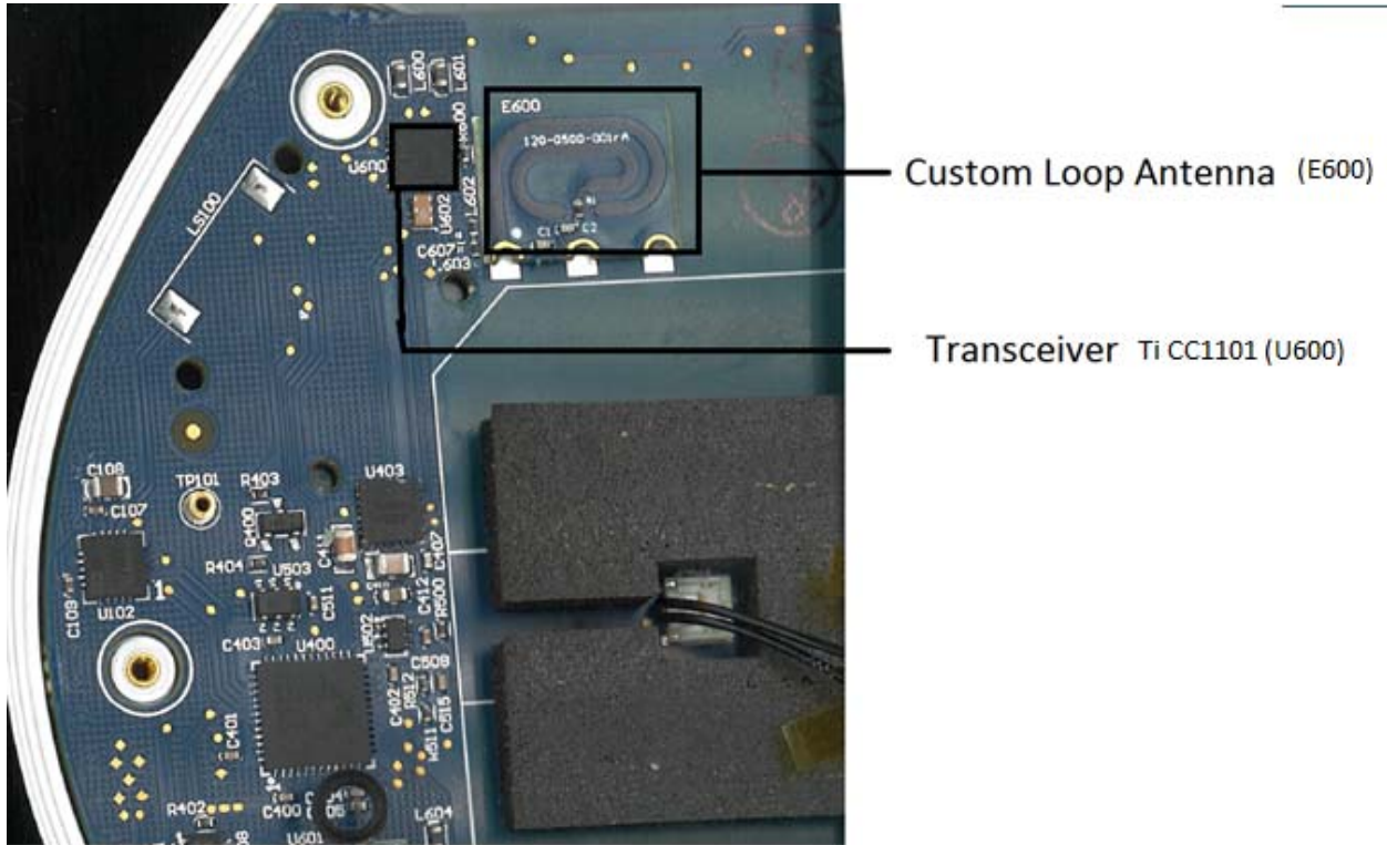
RF circuitry
