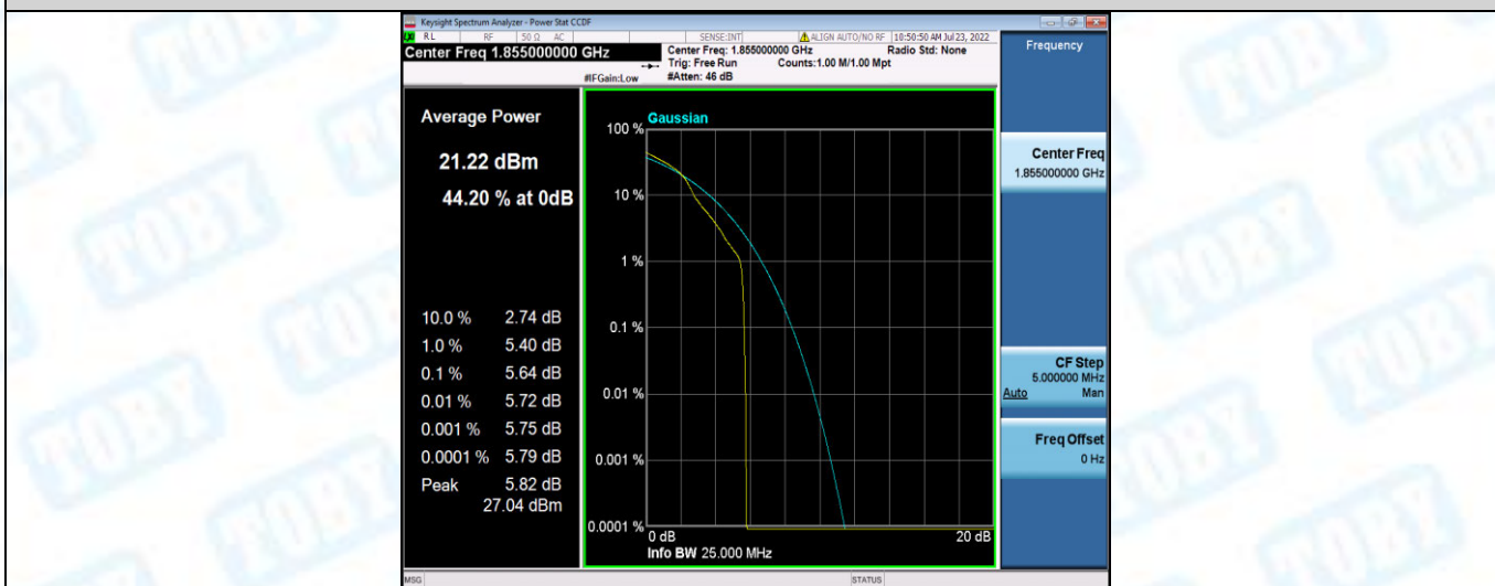
Band25-10MHz-16QAM-26090-50RB#0
