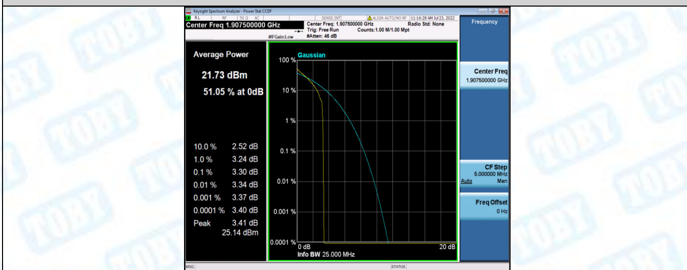
Band25-15MHz-QPSK-26615-75RB#0
