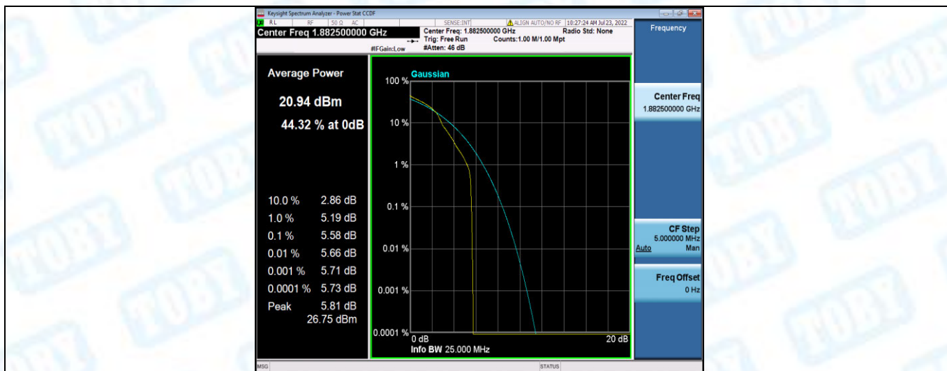
Band25-5MHz-16QAM-26365-25RB#0
