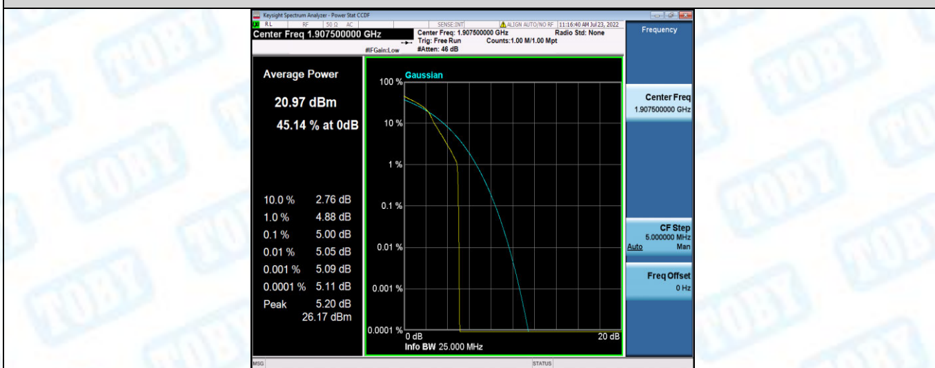
Band25-15MHz-16QAM-26615-75RB#0
