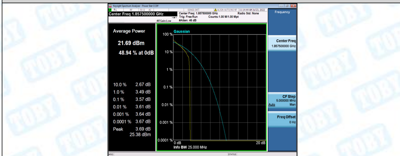
Band25-15MHz-QPSK-26115-75RB#0
