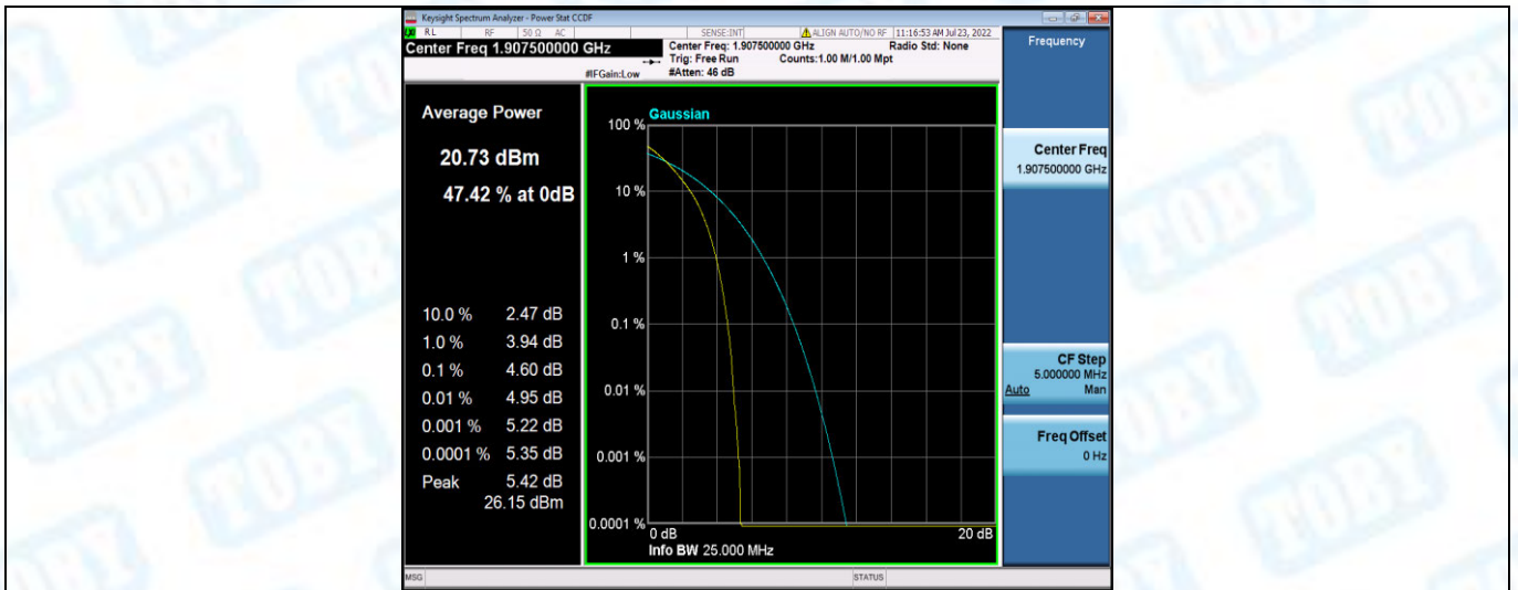
Band25-15MHz-16QAM-26115-1RB#0
