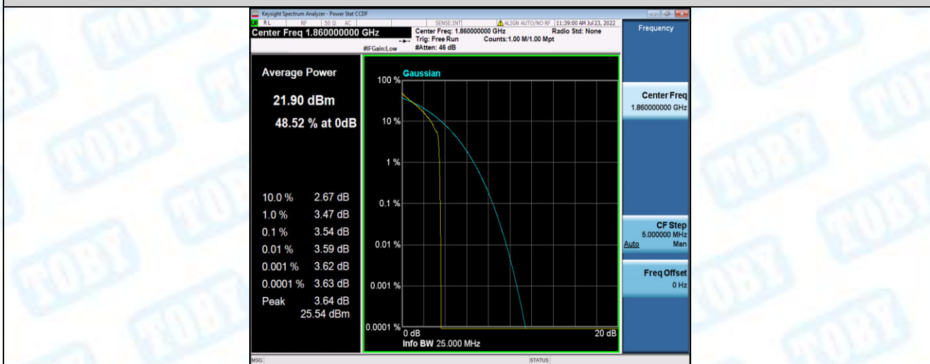
Band25-20MHz-QPSK-26140-100RB#0
