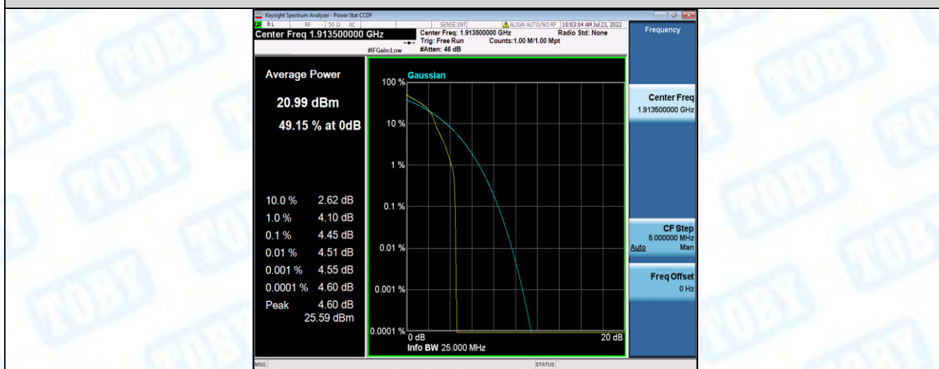
Band25-3MHz-16QAM-26675-15RB#0
