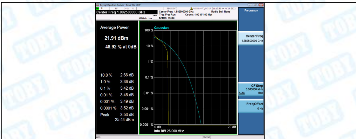
Band25-15MHz-QPSK-26365-75RB#0
