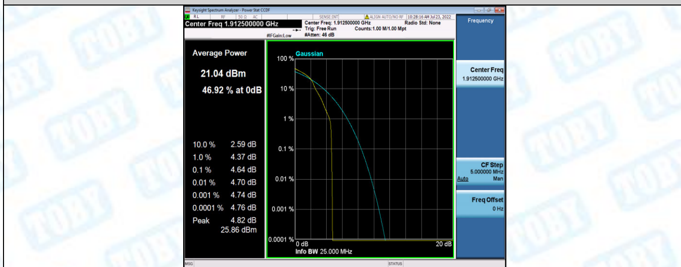
Band25-5MHz-16QAM-26665-25RB#0
