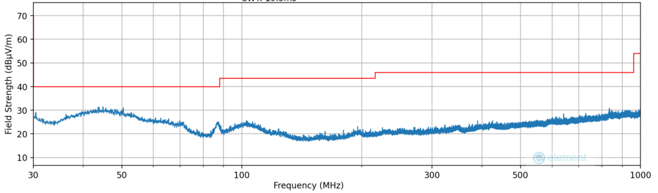
Plot 7-4. Radiated Spurious Plot 30MHz – 1GHz (Pol. H)
