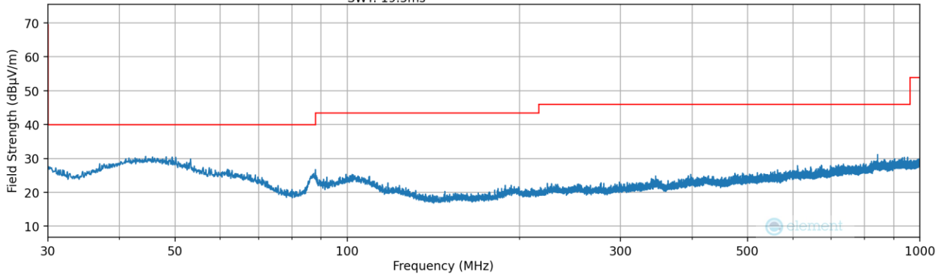
Plot 7-5. Radiated Spurious Plot 30MHz – 1GHz (Pol. V)
