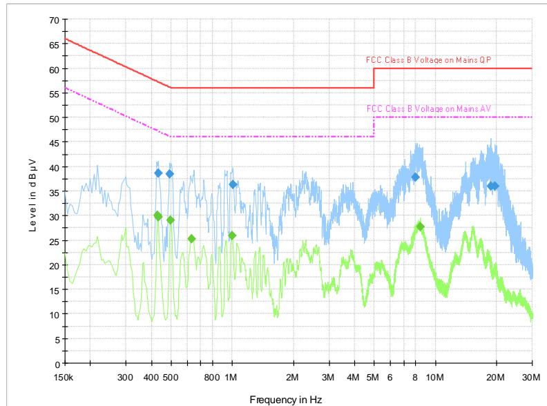
Fig.B.9.1 AC Powerline Conducted Emission-blutetooth
