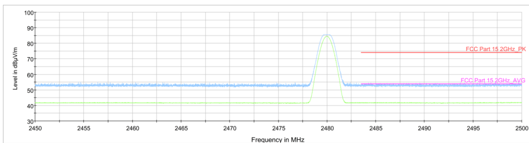
Fig.4. Frequency Band Edges: GFSK, 2480 MHz, Hopping Off, 2.45 GHz - 2.50GHz
