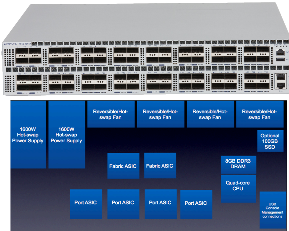
Figure 4: Arista 7250QX-64 (above: Physical Image, below: Logical device layout)
