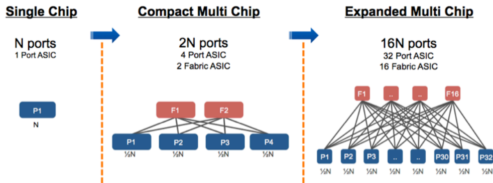
Figure 3: Comparison of single chip and multi chip scale and flexibility
