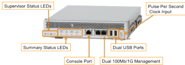
Figure 9: Arista 7300 Supervisor Module.
