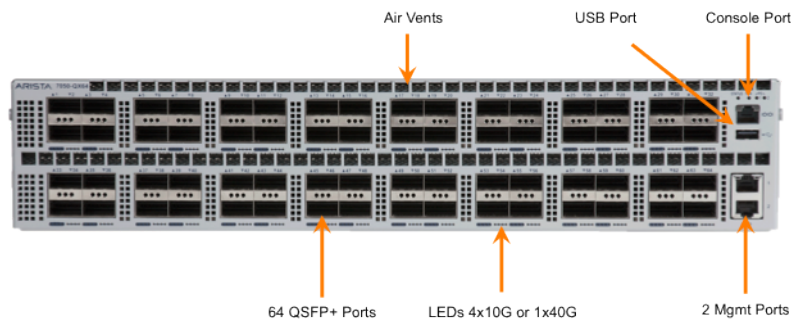
Figure 10: Arista 7250QX
