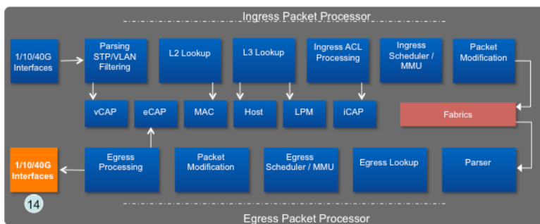
Figure 26: Packet Processor stage 14: Network Interface (Egress)
