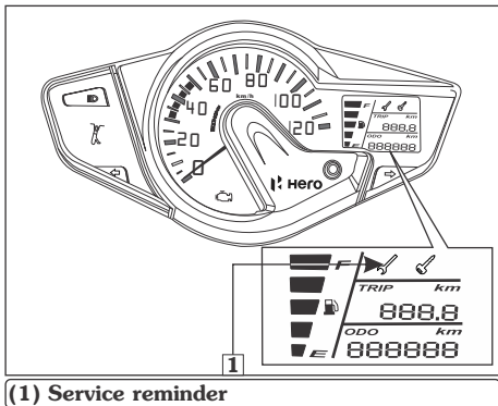
(1) Service reminder
