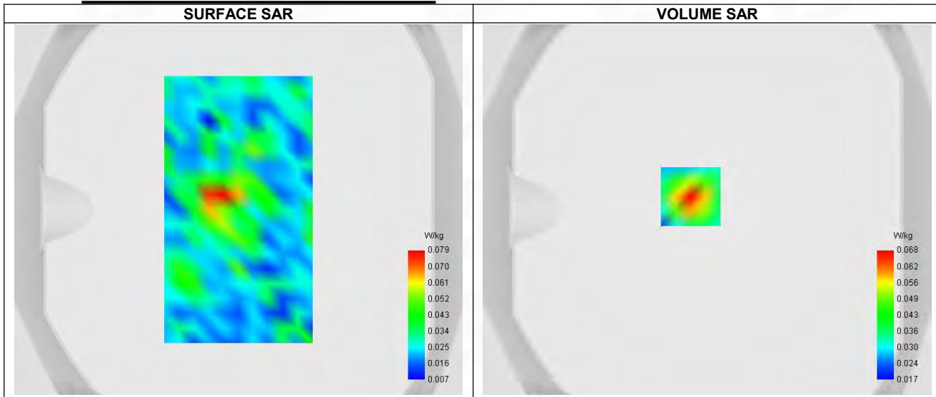
Maximum location: X=-9.00, Y=7.00 ; SAR Peak: 0.12 W/kg
