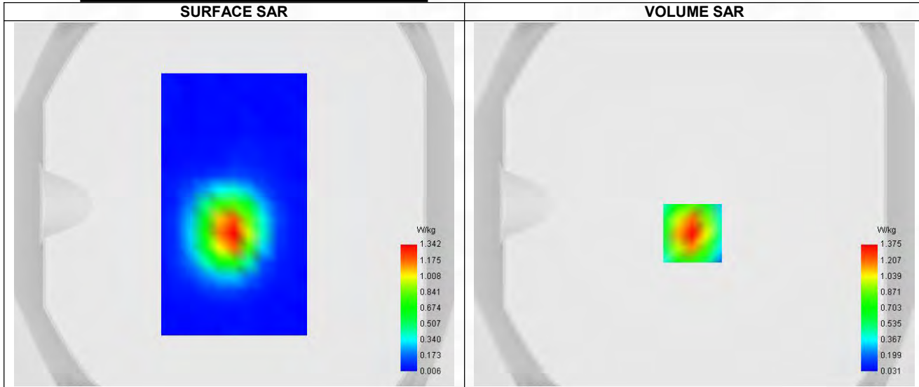
Maximum location: X=-1.00, Y=-16.00 ; SAR Peak: 1.94 W/kg
