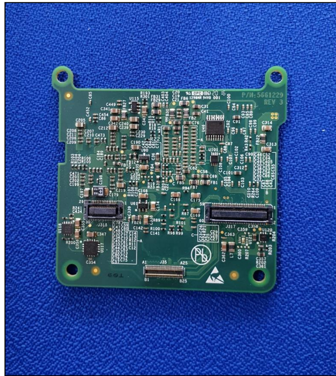
Photo 1: MST Board
